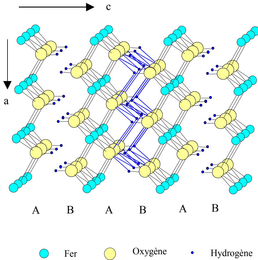
Figure 2: Structure de \beta\text{-Fe(OH)}_2
