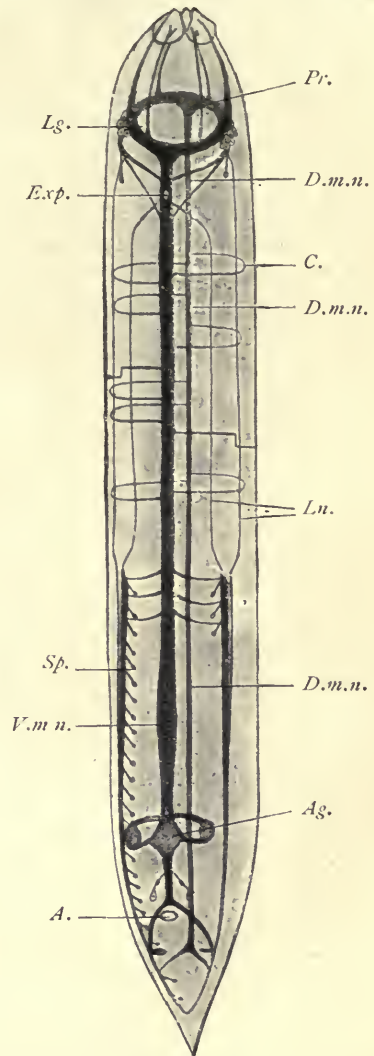
FIG. 263.—Schematic representation of the nervous system of a male Ascaris megalocephala . A. , anus; Ag. , anal ganglion; C. , commissures; D.m.n. , dorsal median nerve; Exp. , excretory pore; Pr. , œsophageal sensory ring; Lg. , lateral ganglia; Ln. , lateral nerve; Sp. , papilla; V.m.n. , ventral median nerve. (After Brandes.)
