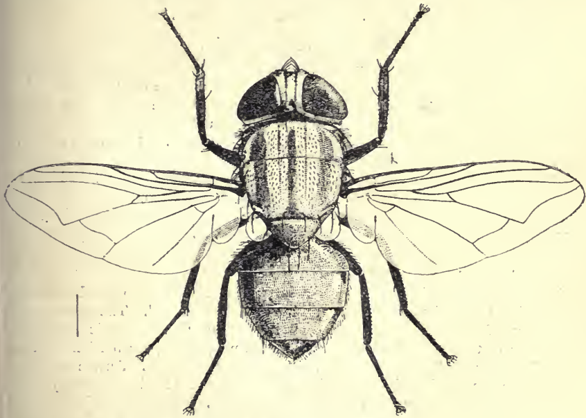
FIG. 408.—The screw-worm fly ( Chrysomyia macellaria ).
