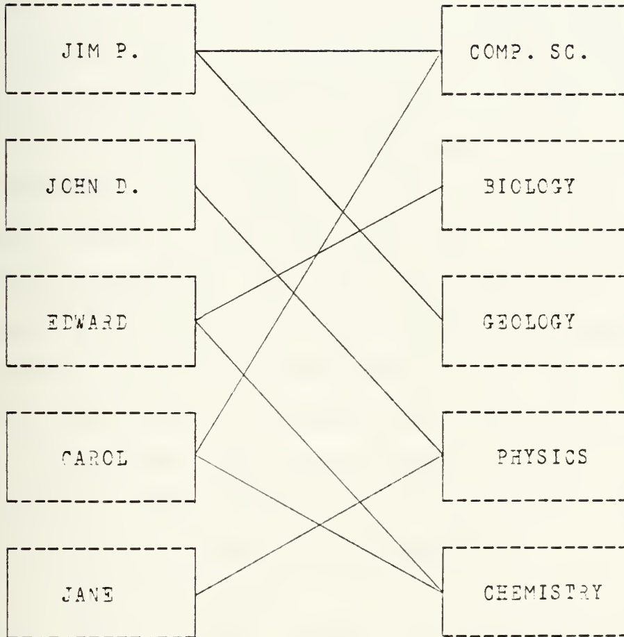
Fig. 2-2. STUDENT-COURSE Relationships.
