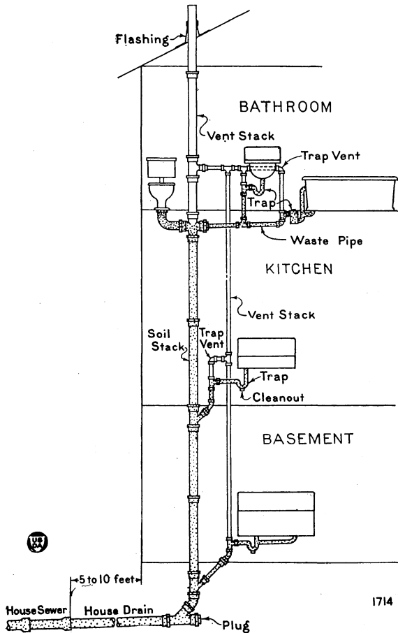
FIG. 5.—A typical 5-fixture job. Drainage pipes are stripped and vent pipes are outlined
