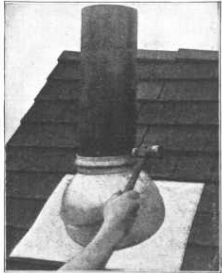
FIG. 41.—Beating down the lead collar to make a water-tight joint
