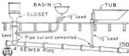
FIG. 1.—Plumbing fixtures poorly connected; the bathtub has no trap; the basin trap is subject to self-siphonage and is forced by bubbles of sewer air when the water-closet is flushed; cutting into vitrified sewer pipe makes rough, leaky, easily obstructed joints and is a poor substitute for branch fittings
