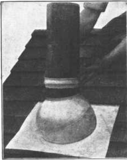
FIG. 40.—Dropping the lead collar upon an adjustable roof flange
