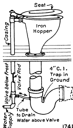
FIG. 32.—An antifreezing water-closet
