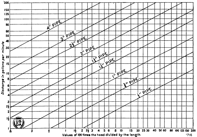
FIG. 7.—Diagram giving the discharge of 1/2-inch to 4-inch straight water pipes
