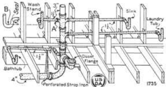
FIG. 26.—Supporting and roughing-in a simple, one-pipe system—a very economical method for bungalows and cottages with fixtures on one floor and near the soil stack. Note three points: (1) There are no back vents; (2) all small waste pipes enter the stack above the closet branch, thus preventing the water-closet from siphoning the small traps; (3) in no instance is the inside bottom of the waste pipe at the stack (point A) lower than the dip of the trap (point B), thus preventing self-siphonage of the trap; this provision limits the length of the waste: for example if the trap seal is 2 inches and the slope of the waste is ¼ inch per foot, its length should not exceed 8 feet (2 divided by ¼ equals 8) and less would be better.
