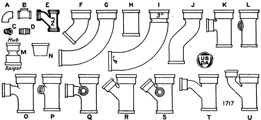
FIG. 8.—Fittings: A, plain elbow or ell, turns one-quarter of a circle or 90 degrees; B, beaded tee branch; C, shoulder bushing; D, shoulder nipple; these four are typical wrought water pipe fittings; E, section of 90-degree long-turn Y branch or TY drainage fitting recessed and threaded for wrought pipe; note that the point Z is below the center line of the inlet pipe, an important feature in soil and waste lines; F, eighth or 45-degree bend, cast-iron, hub and spigot type; G, long-sweep quarter bend; H, sleeve, sometimes used for joining two spigot ends on repair work; I, long-sweep reducing quarter bend, 4-inch spigot, 3-inch hub, often used at the bottom of 3-inch soil stacks; J, offset; K, T-branch; L, T-branch tapped for wrought pipe; M, reducer; an increaser has the spigot on the smaller end; N, plug; O, sanitary T-branch; P, sanitary T-branch tapped for wrought pipe; Q, sanitary T-branch with right-hand side inlet; R, Y-branch; S, Y-branch with right-hand side inlet; T, combination Y and eighth bend or TY fitting; U, upright Y-branch.
