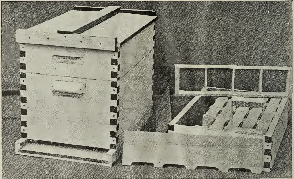
FIG. 4.—The above shows the AE64S | 8 Dovetailed hive—a 1½-story hive for comb honey, with 4¼-inch slotted sections. The super at the right is opened up, showing the 4¼-inch slotted sections used in slotted-section holders with slotted separators. You will observe that the only difference between this hive and the foregoing is in the inside fixtures of the super. This hive has the slotted 4¼-inch sections, section-holders, and separators, while the first has the plain 4¼ sections, section-holders, and fences. This difference is indicated by the change of the letter P to S in the number. This hive is also furnished in all the different combinations and sizes. With this hive will be included this year the wire spring instead of the wooden wedge back of the follower. You will see the spring attached to the follower in the above illustration. This is a decided improvement. You can also have the option of the slat separator in the S supers if preferred.
