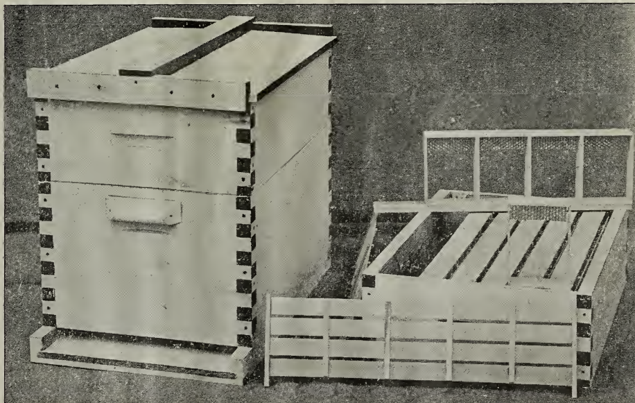
FIG. 5.—The above shows the AE64I | 8 Dovetailed hive, a 1\frac{1}{2} -story hive for comb honey with 3\frac{7}{8} \times 5 plain sections (Ideal). The super at the right is opened up, showing the Ideal sections, five in a row, supported on a plain slat \frac{3}{8} inch thick, in a deep super, with I fences. This super takes 30 sections in the eight-frame size, where only 24 of the 4\frac{1}{4} -inch sections can be placed in the regular shallow super. These sections hold the same as the 4\frac{1}{4} of the same width, and satisfy the demand for a tall section. In some markets, which are educated to a full-weight section, these are not as desirable as the 4 \times 5 \times 1\frac{1}{8} plain, which hold more nearly a pound. This size can not be used to advantage in the 8-frame super unless they are placed on slats crosswise the deep super, and short fences are used. A super so equipped is designated by the letter I, in place of I, and holds 30 4 \times 5 \times 1\frac{1}{8} plain sections on I, plain slats with 11 I, fences.
