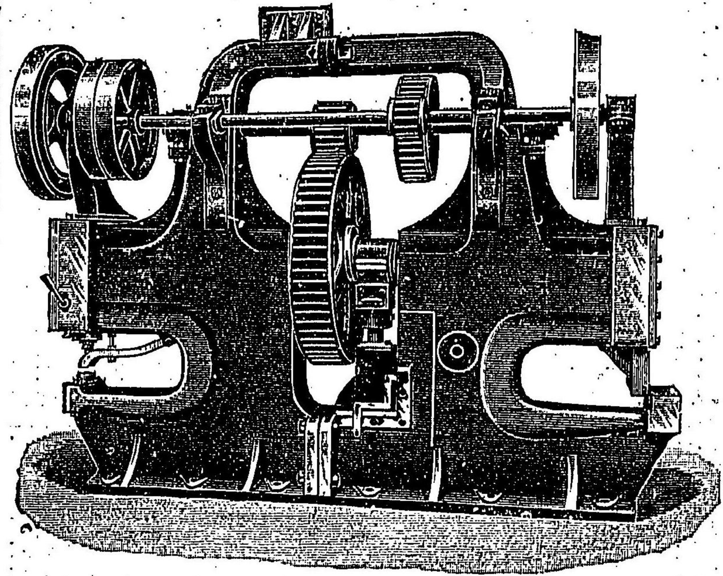
Punching Shearing & Angle-iron Cutting Machine.
