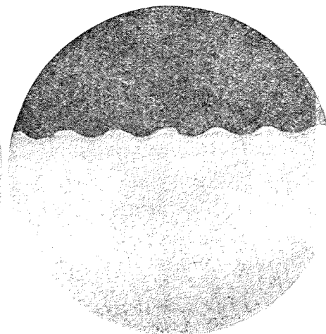
Fig. 7 Zinc cross section after 54000 prints Fig. 8 Copper cross section after 54000prints
