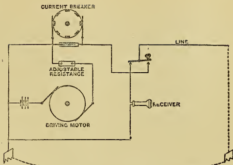
FIG. 1. Diagram of connections of Mr. Preece's system.
