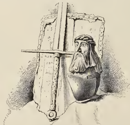
Fig. 8. SWORD AND SHIELD OF EDWARD III., ETC.
