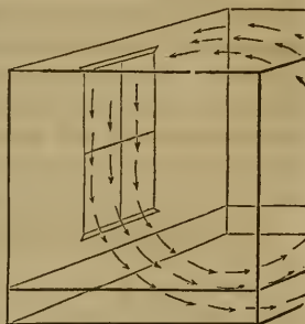
Currents produced in winter by single windows.
