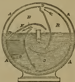
Meter for measuring the flow of Gas.
