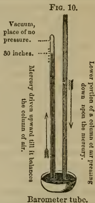
Barometer tube.
