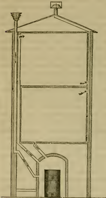
Manner of warming by Hot-Air Furnaces.
