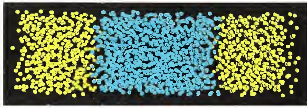
Fig. 16. Two-component fluid-fluid interface system at equilibrium. As seen in the figure, equilibrium is characterized by two distinct interfaces.
