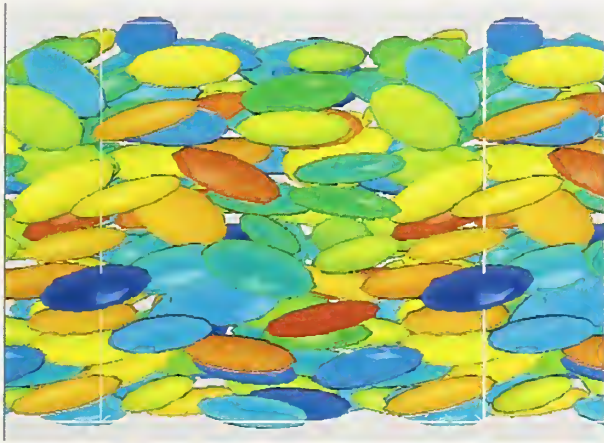
Fig. 8. Dense suspension of ellipsoids similar to typical aggregate contribution in concrete. Jeffery's Orbits are suppressed and the alignment between ellipsoids is enhanced.
