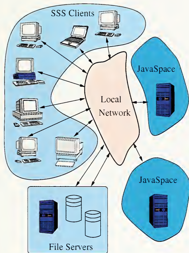
Fig. 26. A high-level view of the Screen Saver Science architecture. Clients access a shared object space (JavaSpace) to retrieve tasks to perform, return results, send messages to other clients, broadcast status messages for general use, and exchange other messages as needed. Large data sets will be stored on disk with client access to these files coordinated through entries in the shared object spaces.
