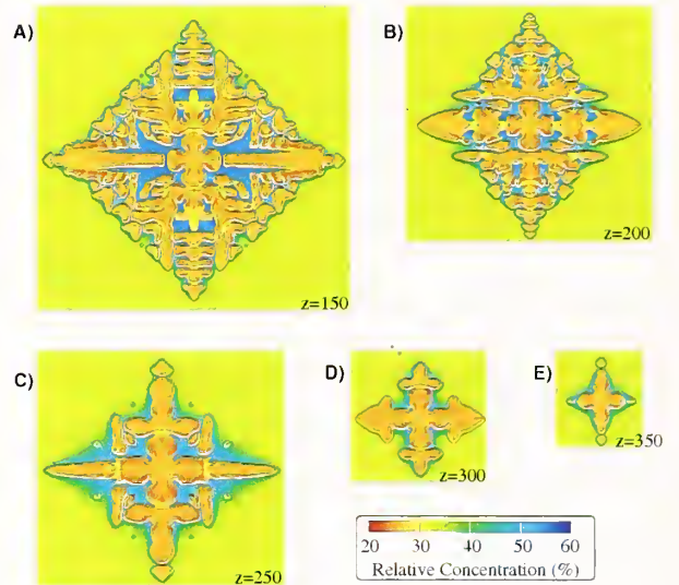
Fig. 25. Several more 2D slices of the dendrite in Fig. 23. Each z value indicates by an integer the position of the slice along the z axis.
