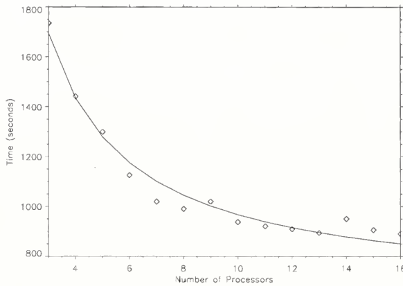
Fig. 21. Execution time versus number of processors for concentric spheres problem.
