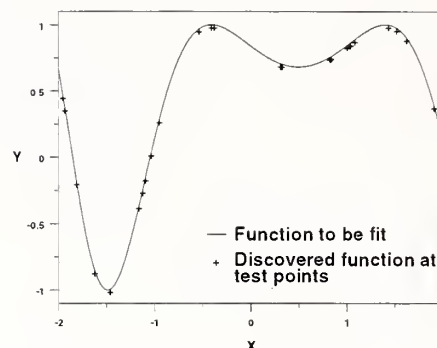
Fig. 27. Results of an example regression run. Values of the GP-discovered function are shown at points that were used by the GP system to determine fitness.
