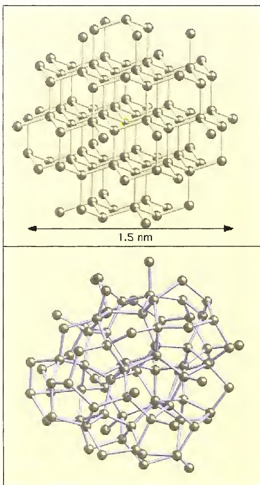
Fig. 12. (a) The 87 atom cluster used to calculate the XANES of crystalline Ge. (b) A similar cluster of 87 atoms of aGe from the CRN displayed with the same length scale.
