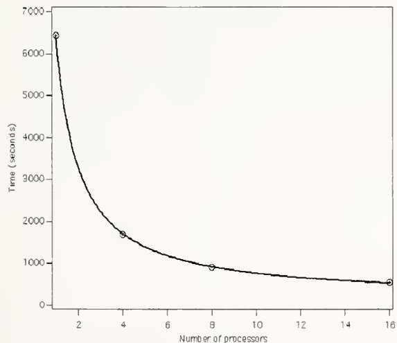
Fig. 6. Hy-CI Scaling with Cluster Size.
