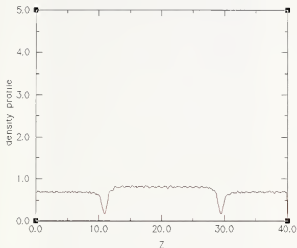
Fig. 18. Plot of the particle density. The fact that the unlike particles do not like to mix is evident from the distinct decrease (the dips in the curve) in the particle density in the interfacial regions.
