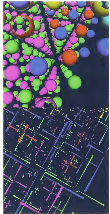
Fig. 22. A section of a nanostructure (top) with orbitals (bottom).
