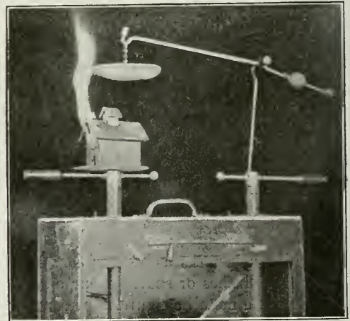
FIG. 25.—Barn with hayfork track, fired by flash. If track had been grounded current would have followed ground wire, and no fire would have occurred. If points had been used flash would have been prevented.
