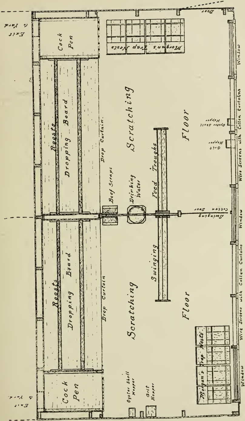
Fig. 2. Ground Plan of House No. 2.
