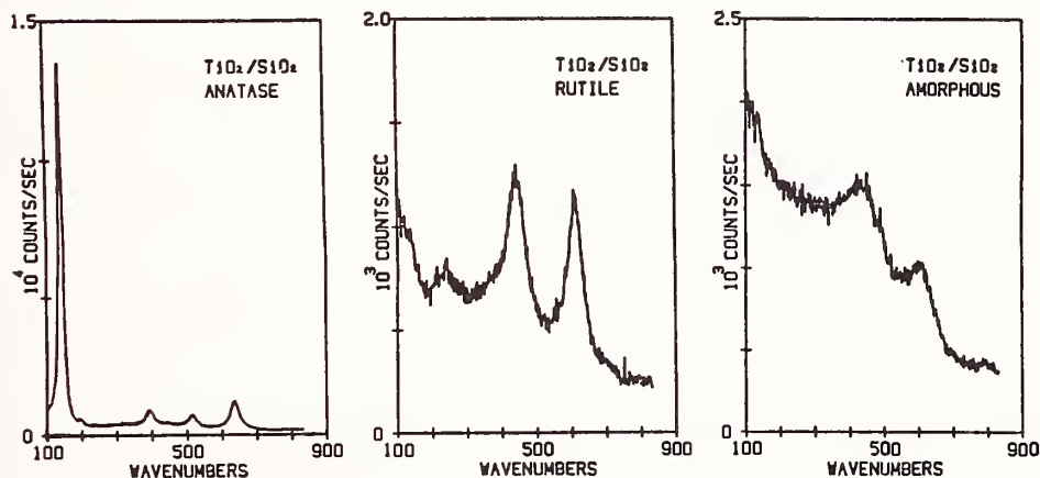
Figure 1. Raman spectra of stoichiometric TiO_2 films with different structures demonstrating the effectiveness of using Raman spectroscopy for thin film characterization. Film thickness is 500 nm.
