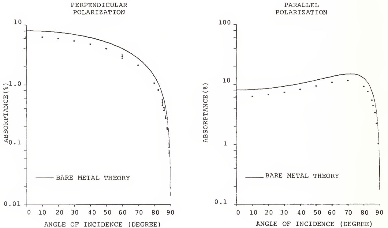
Figure 2. Absorptance curves for bare silver at 0.5145 \mu\text{m} for both s and p polarizations. The solid curve is Fresnel's equations using the values of n and k given in reference 5.
