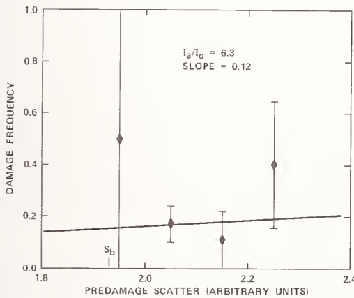
Figure 11(a). Distribution of damage frequency vs predamage scatter for Mirror C at I_a/I_0 = 6.3 presented in the manner of figure 5. Data points represent damage frequencies of tenth-unit scatter intervals. The scatter scale differs significantly from that of Samples A and B because of the different test configuration.
