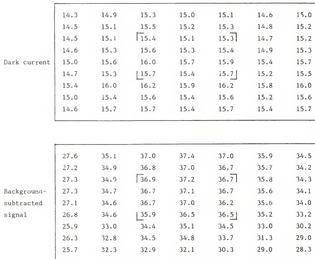
Figure 4. Mappings of vidicon target dark current and background - corrected signal in trapix grey levels (0-83) at T=0^\circ\text{C} . The bracketed 3 x 4 cell region corresponds approximately to the central 3.75 x 3.13 mm region of the target.
