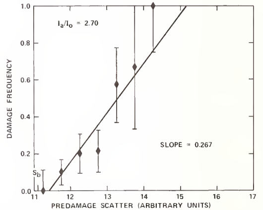
Figure 8(b). Distribution similar to figure 8(a) for Mirror B at I_a/I_0 = 2.70 .
