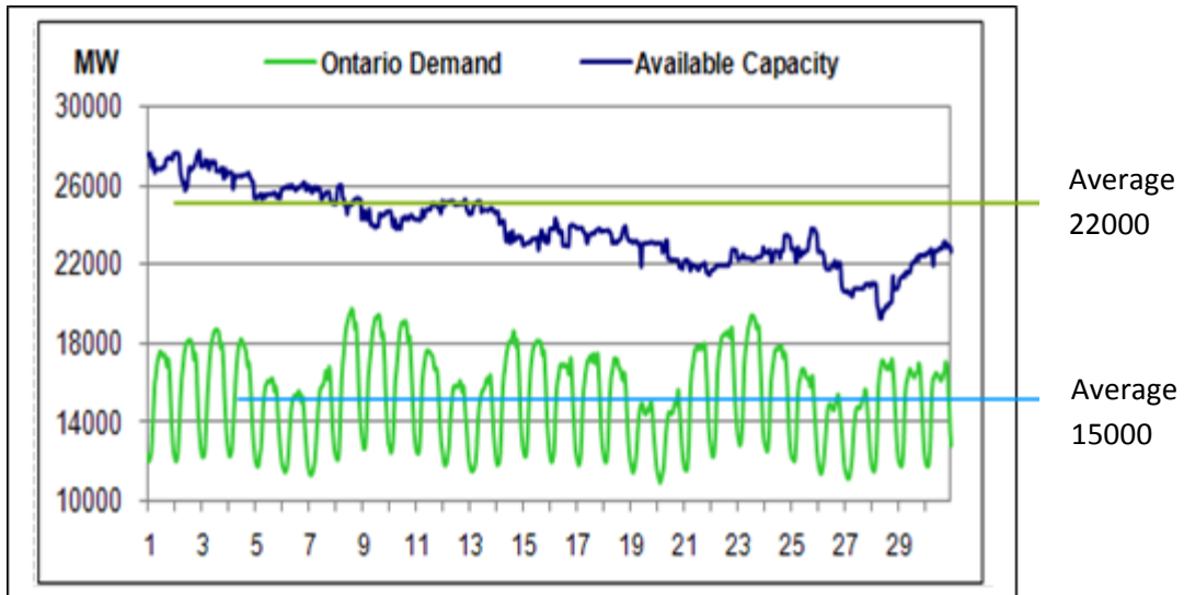
Ontario Demand and Capacity Load Variation for a Month
