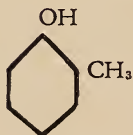
o-Cresol
