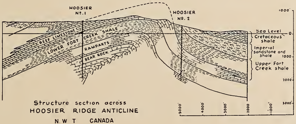
Fig. 4. Cross-section through coral-reef anticline with reef exposed at surface crest where only "tar" and solid bitumen were encountered with sulphur water. Example of oil reservoir which has lost its oil content due to erosion of impervious cap rock.
