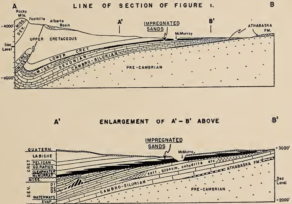
Fig. 3. Diagrammatic cross-sections, Rocky Mountains to McMurray area.
