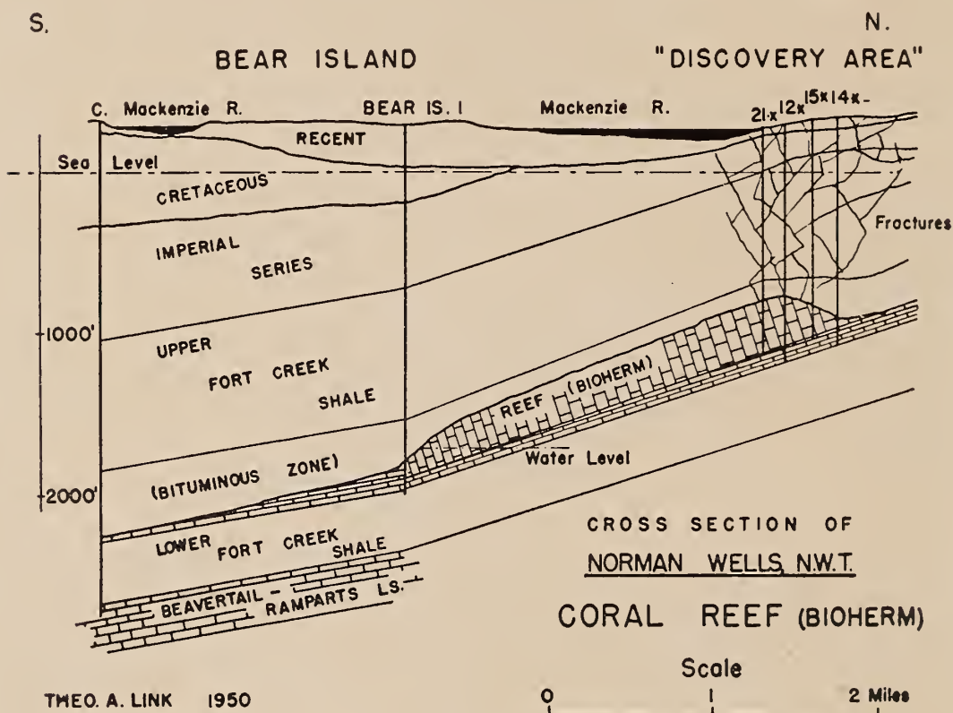
Fig. 3. Cross-section, through Norman Wells pool, Northwest Territories, showing surface fractures through which oil and gas are escaping, giving rise to oil seepages and impregnation of recent delta gravels and sand deposits with oil. Depth from surface to top of reef is 1,000 feet.
