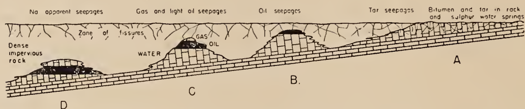
Fig. 5. Ideal diagram illustrating escape of oil and gas through fractures from reef reservoirs at various depths. (A) Reef exposed at surface with only bitumen in rock and sulphur springs. (B) Reef near enough to surface to have lost all its gas and considerable oil. (C) Reef buried sufficiently to have retained some of its gas and most of its oil. (D) Reef buried at depth beyond reach of surface fractures so that it retained its original gas and oil content.
