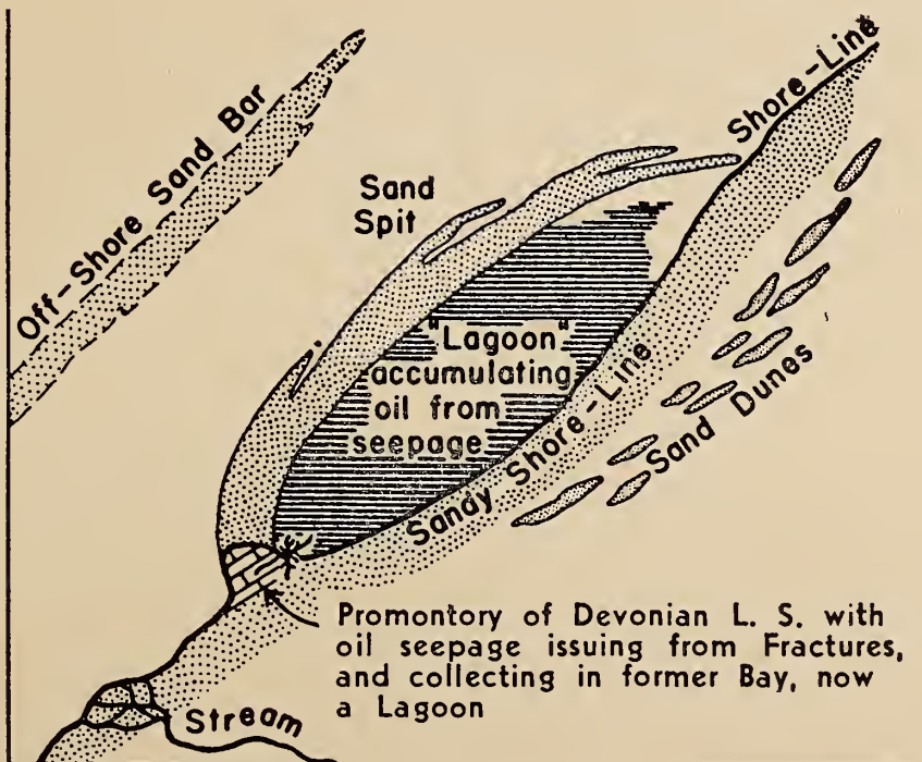
Fig. 7. Sketch map illustrating how oil seepage from Devonian could cause accumulation of layers of “bitumen” interbedded in bituminous sands.
