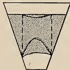
(B) SLUMP OF TOP SURFACE INSIDE THE SHEAR FAILURE.
