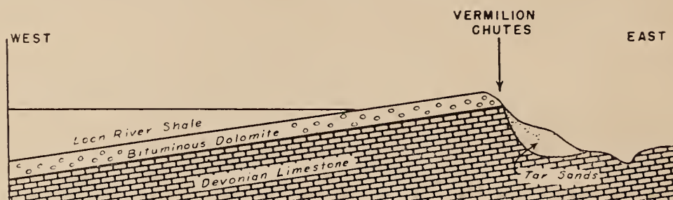
Fig. 6. Diagrammatic cross-section of Vermilion chutes, Peace River, Alberta. (From S. E. Slipper.)
