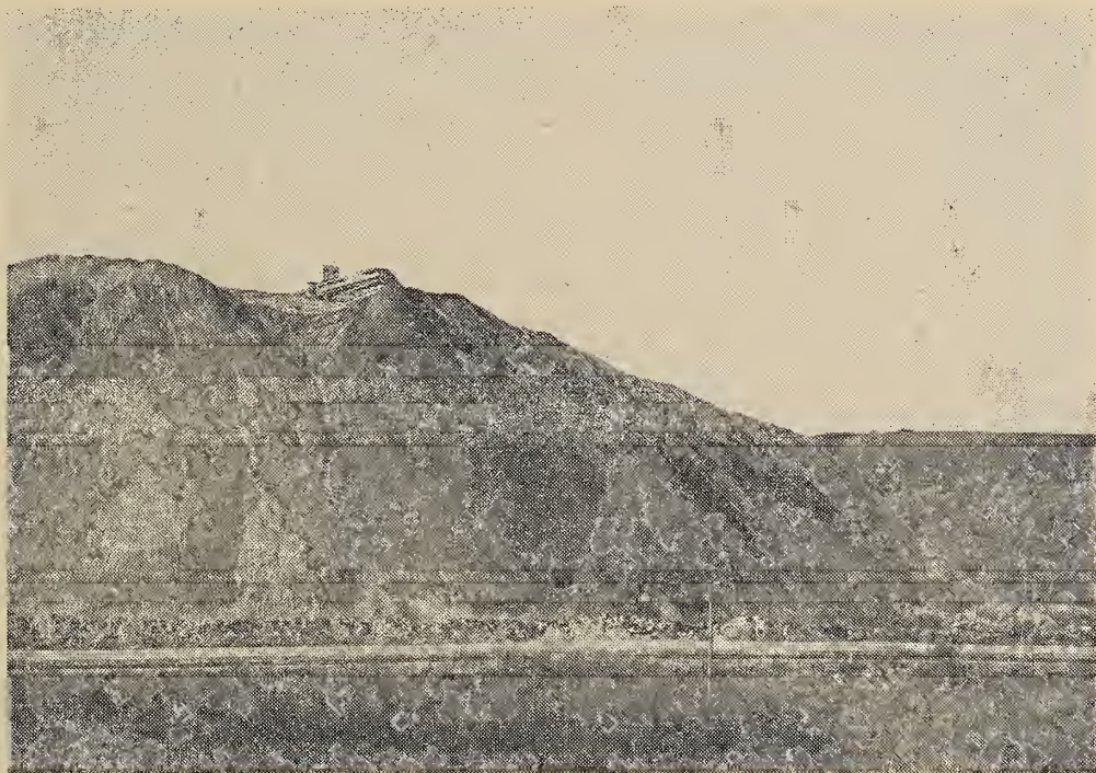
View of the overburden dump. Vertical height at this point is 150 ft. No difficulty has been experienced with slides except when depositing wet material on swampy ground covered with muskeg.
