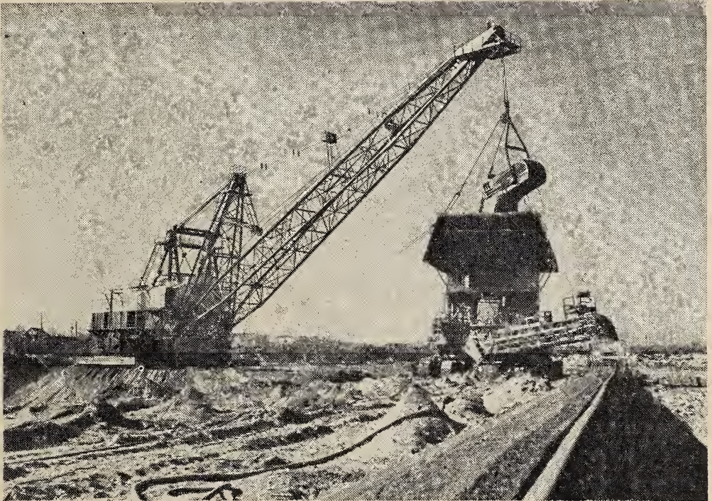
View of dragline and screening plant at the Morton mine. The model 1150-B dragline has a 180-ft. boom with a 30-cu. yd. bucket. The maximum digging depth is 110 ft. and the dumping height is 60 ft. Ground pressure of the base is 11 p.s.i. and of the walking shoes 21.9 p.s.i.
