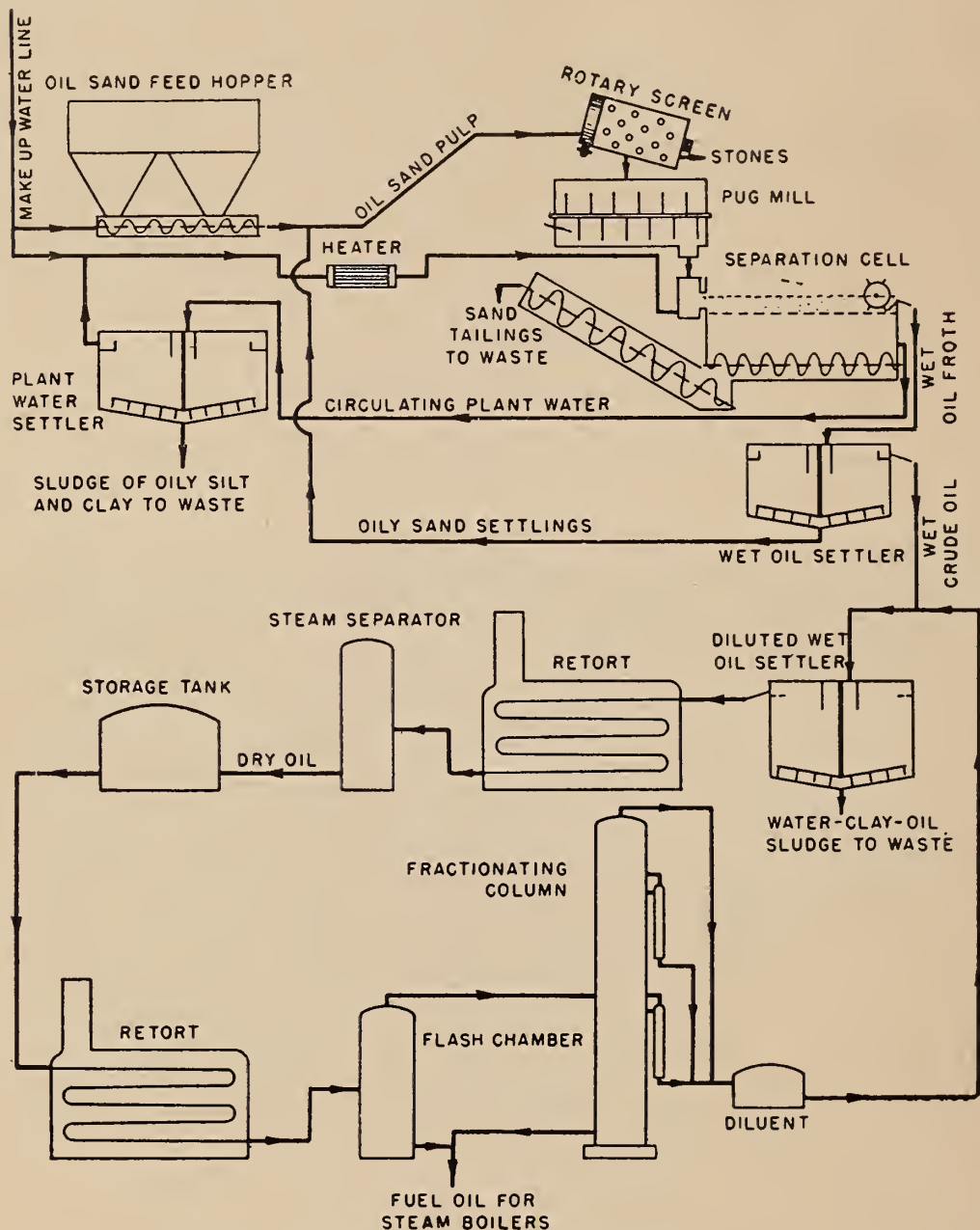
Flow-Sheet of Oil-Sand Pilot Plant at Bitumount
