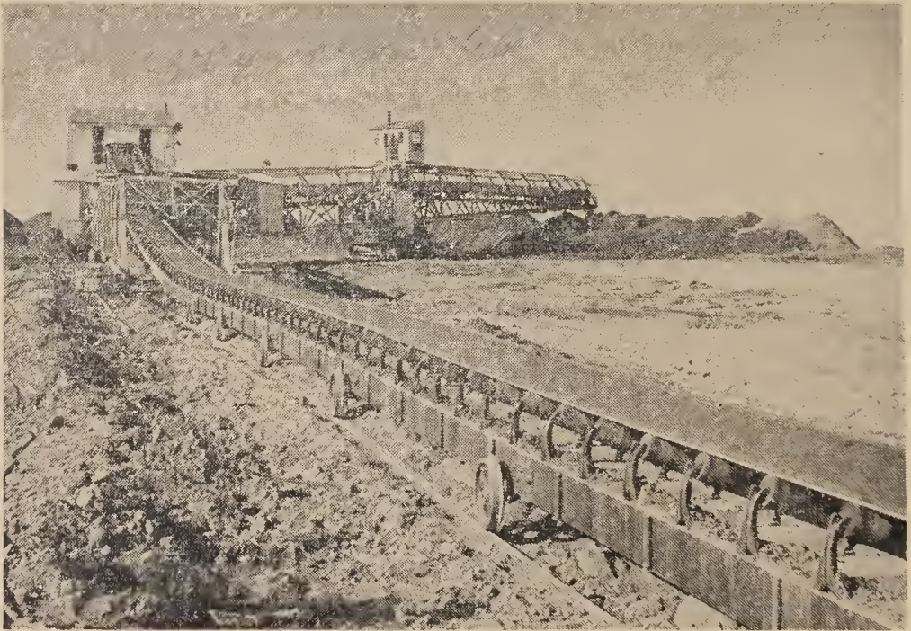
View of trailing truss and stacker. The stacker boom is 245 ft. long, with 75 ft. of cantilever beyond the support. Its centre of support is a ball and socket joint mounted on an electrically propelled 54-B shovel base. The stacker swings through an arc of 180°. Stacker equipment is controlled from the house directly above the support point. The trailing truss and conveyor are pulled forward by power units in the bolster at the pivot point as the dump advances. Stacker can advance on a grade of 10%, but length of trailing conveyor on 10% grade is limited to about 600 ft.
