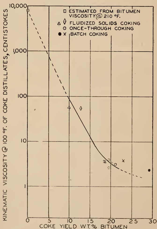
Fig. 2. Viscosities of coke distillates produced from bitumen.
