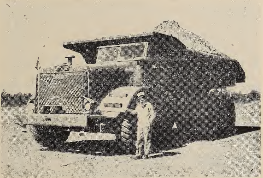
A 50-ton experimental model LLD Euclid truck having two 300-h.p. Cummins engines driving tandem rear axles. Note the thermostatically controlled shutter over the radiator core. The cooling fans are also controlled by the temperature of the engines. Capacity of the box is 32 cu. yd. water level.
