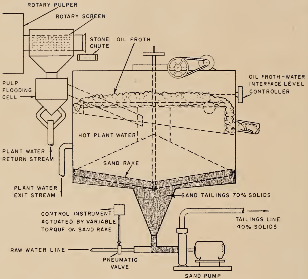
Fig. 1. Diagrammatic drawing of simplified separation cell.
