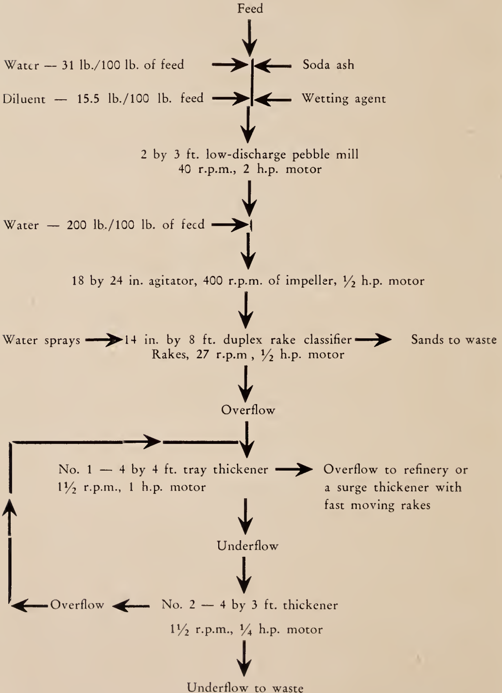
Fig. 1. Flow-sheet.
