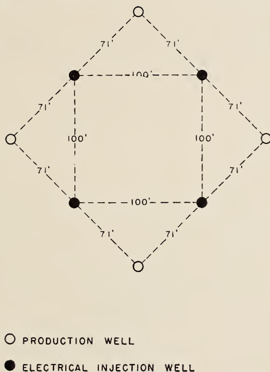
Fig. 1. Modified five-spot well system for recovery of oil by electrovolatilization.
