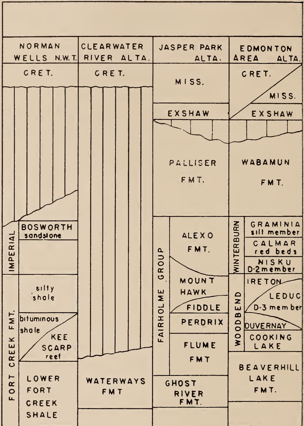
Fig. 1. Four Upper Devonian sections of Western Canada.
