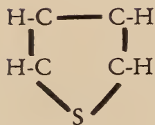
Thiophene
