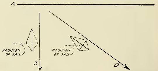
DIAGRAM ILLUSTRATING THE ACTION OF THE WIND ON AN ICE-BOAT.
