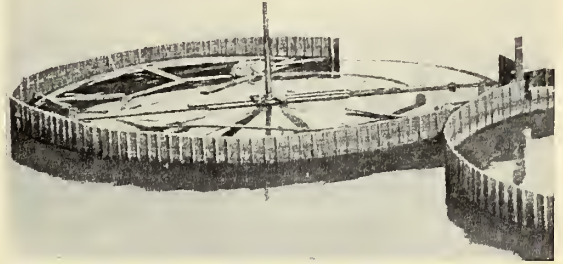
A PARTLY COMPLETED CYLINDER SHOWING THE TEMPLET ABOUT WHICH THE SHEET-PILES HAVE BEEN DRIVEN.
