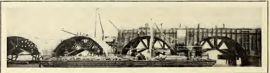
SETTING UP THE FORMS FOR THE FIFTY-FOOT CONCRETE ARCHES.
