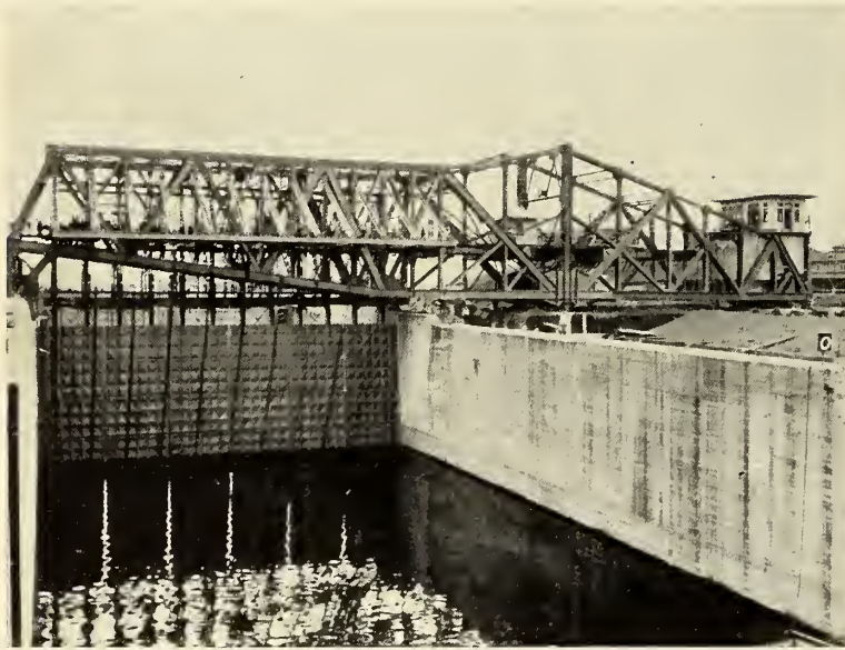
EMERGENCY GATE WITH PLATES LET DOWN TO CUT OFF THE FLOW OF WATER.
