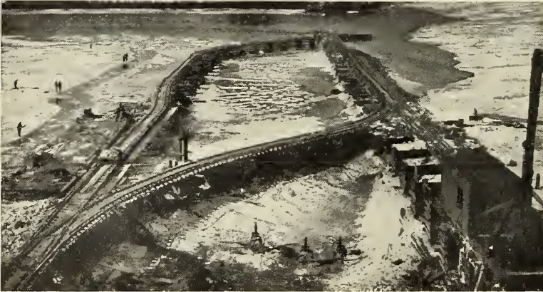
HOW THE COFFER-DAMS WERE BUILT, ONE IN ADVANCE OF THE OTHER.
