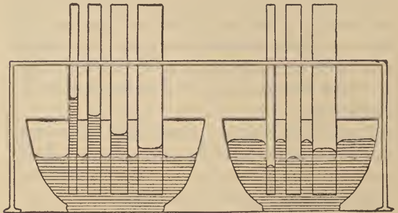
CAPILLARITY
