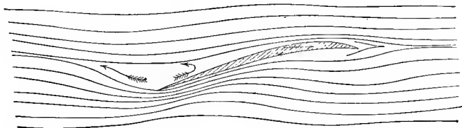
FIG. 25.—PROBABLE ARRANGEMENT OF STREAM LINES DURING MOVEMENT OF CONVEXED AND CONCAVED PLANE.
