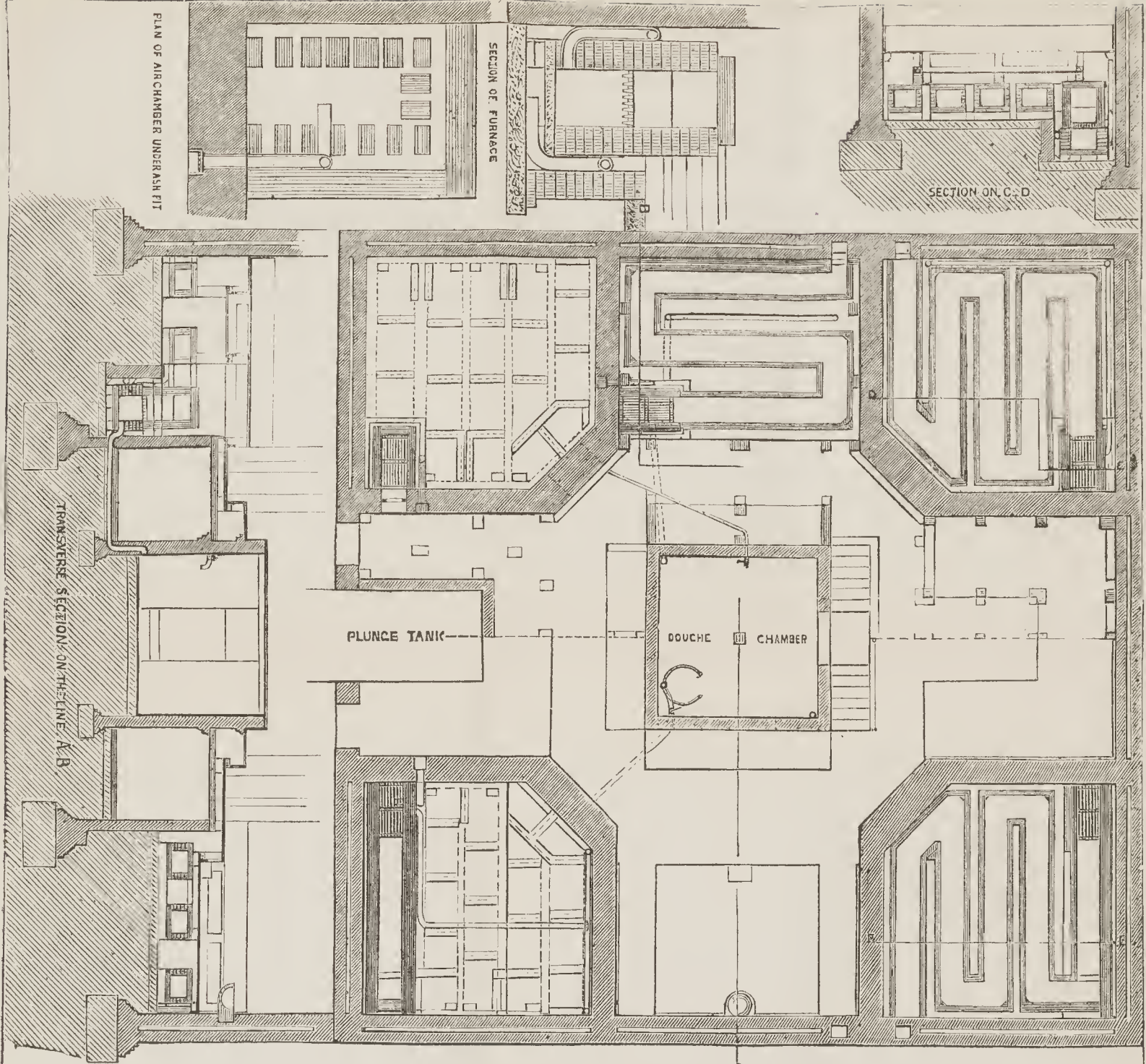
PLAN SHEWING SECTIONS AND FOUNDATIONS OF FLYES AIRPIPES &c
