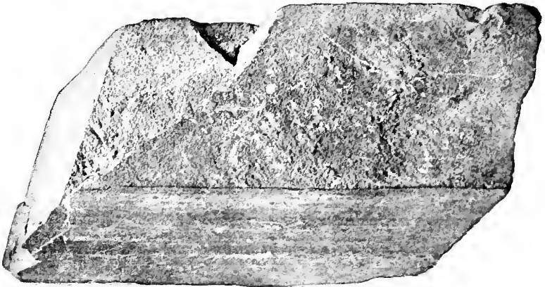
FIG. 34. Fracture cleavage developing polygonal blocks in slate previously possessing flow cleavage.
