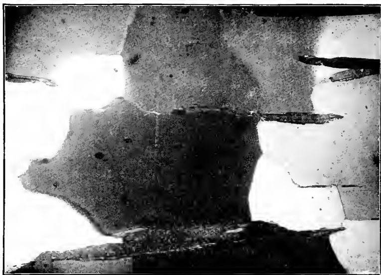
FIG. 38. Photomicrograph of micaeous and quartzose schist showing recrystallized quartz. From Hoosac, Mass. The view illustrates in detail the relation of recrystallized quartz grains to recrystallized mica flakes. The mica flakes for the most part separate different quartz individuals, but they may be seen to bound two or more individuals and to project well into them. It is not probable that such a relation could be brought about by granulation, slicing, or gliding, and it seems best explained by recrystallization.
