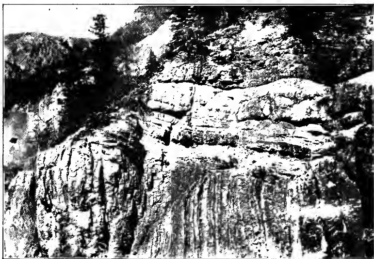
FIG. 66. Horizontally bedded limestone, resting unconformably on vertical beds of Proterozoic quartzite. Box Canyon, near Ouray, Colo. After R. T. Chamberlin.
