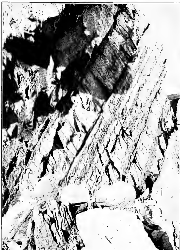
FIG. 37. Fracture cleavage, jointing and flow cleavage developed in graywacke and slate, Alaska. After Gilbert (photograph by U. S. Geol. Survey.) Use principle of strain ellipsoid (See pp. 18-21) to ascertain direction of relative displacement and theoretic position of fracture planes and flow planes. (See also Figs. 9 and 10).
