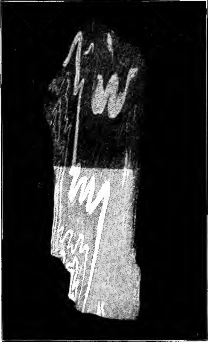
FIG. 34. Illustrating incompetent folds developed by flowage in gneiss. After Van Hise.
