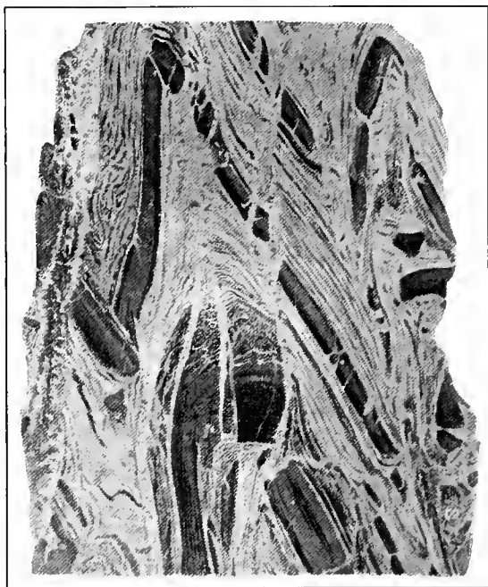
FIG. 52. Folding of brittle and soft layers contrasted in jasper. The broken dark layers are chert, the light layers are secondary iron oxide.
