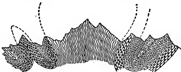
FIG. 49. Generalized fan fold or normal anticlinorium of central massif of the Alps. After Heim.
