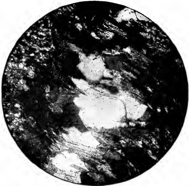
FIG. 45. Photomicrograph of micaceous and quartzose schist with cleavage developed across original bedding, from Little Falls, Minn. A graywacke-slate, in which the banding has been marked by difference in texture as well as in composition, has been subjected to deformation, with the result that a cleavage has been superposed at right angles to the original bedding. Originally the longer diameters of the particles of the bedded rock were parallel to the bedding. Accompanying the development of flow cleavage most of the constituents of the rock have been recrystallized. The quartz particles shown in the light band have been drawn out with their longer diameters nearly at right angles to the former plane of their longer diameters, and abundant new mica has developed with its greater diameters and mineral cleavage normal to the plane of bedding.
