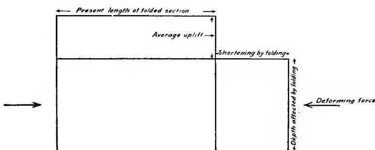
FIG. 61. Illustrating a method of determining depth affected by folds.
