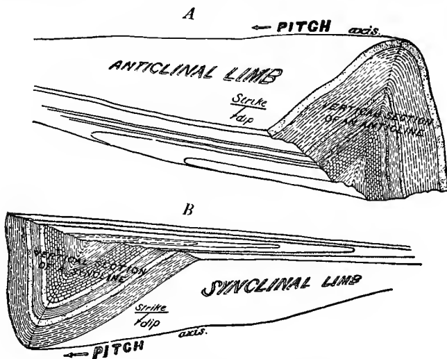
FIG. 48. Parts of folds. After Willis.
