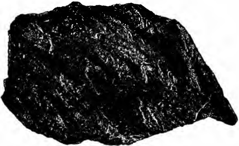
FIG. 28. Fault-slip cleavage in gneiss from southern Appalachians. The gneiss has been closely crenulated and the minute folds may be observed to pass into minute faults which now represent planes of fracture cleavage. The faults may have been cemented or may have been welded by actual pressure. Parallel to the faults there has also been developed a parallel arrangement of the mineral particles, perhaps due in part to the slipping along the fault planes, and it is exceedingly difficult to distinguish between the fracture cleavage and the flow cleavage.
