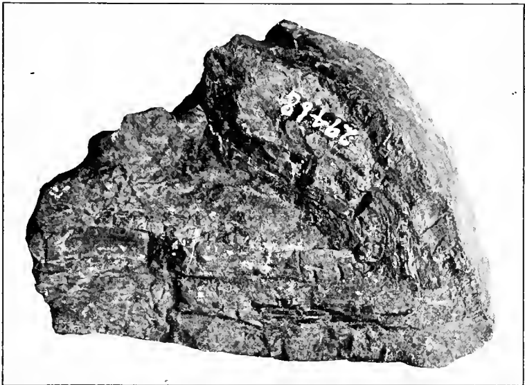
FIG. 53. Folding of brittle and soft layers contrasted in jasper. Note the tension cracks in the brittle layers.
