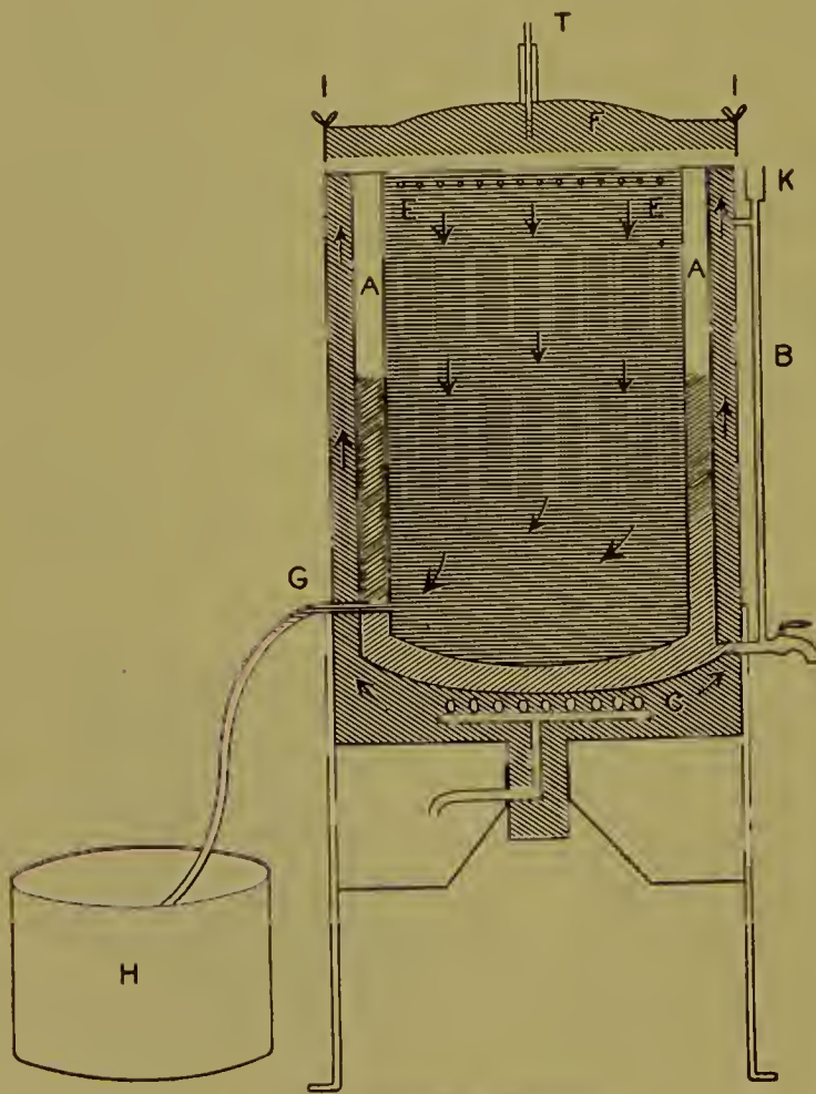
Lautenschläger's apparatus.
