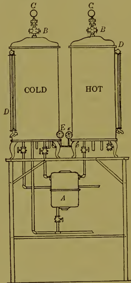
Water-sterilizing tanks.
