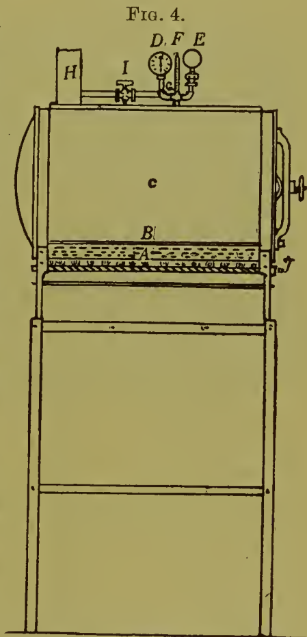
Sterilizer for dressings. Longitudinal section.
