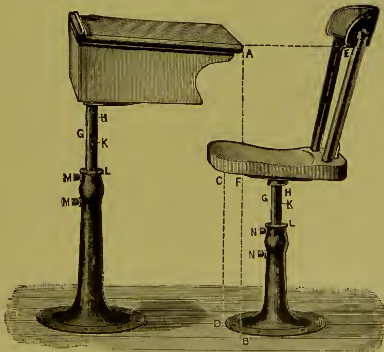
Adjustable seat and desk, showing their proper relative arrangement.
