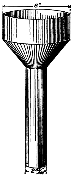
FIG. 21.—Rain gauge, with measuring tube attached.
