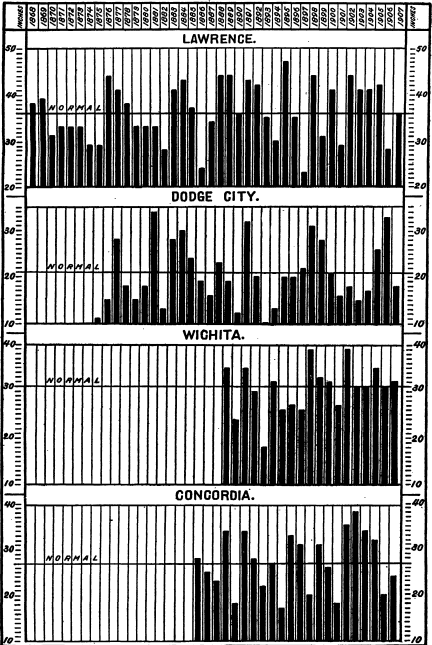
FIG 2.—Variations in annual precipitation at Kansas stations.
