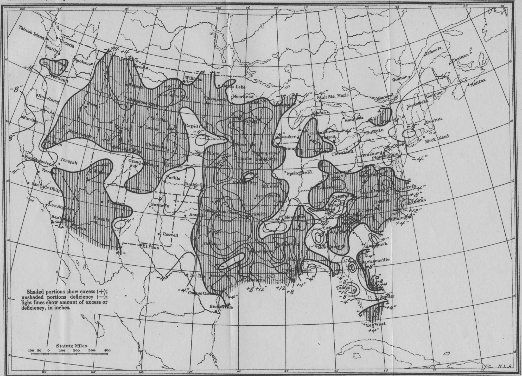
DEPARTURES FROM NORMAL PRECIPITATION FOR THE CROP SEASON OF 1908, FROM MARCH 1 TO SEPTEMBER 30.
