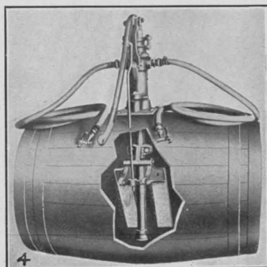
[Fig. 1.—Bucket pumps. Fig. 2.—Knapsack pump. Figs. 3 and 4.—Barrel pumps, showing also agitators.]
