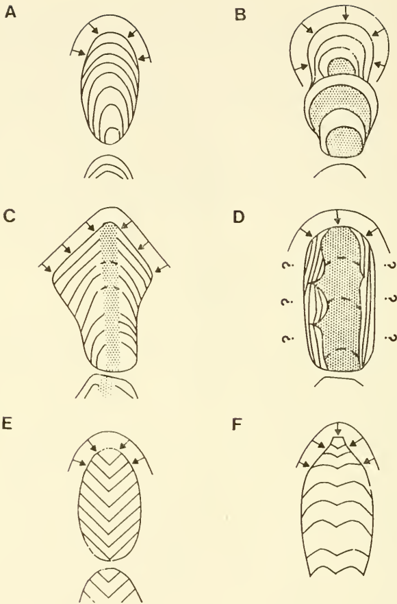
Text-figure 1 A-F. Diagrammatic profiles of compound zoecial walls in the outer exozone portion of cerioporid cyclostomes. Solid lines with arrows indicate inferred position of depositing portion of inner membrane responsible for last episode of cortex growth. Dashed lines in cortex indicate indistinct lamination; solid lines in cortex indicate distinct lamination; cross-hatching indicates subgranular to homogeneous calcareous tissue. In A-D, growth surfaces parallel lamination, and each lamina probably represents a single growth episode. In E and F, the growth surface parallels the depositing epithelia, but cuts across lamination; laminae probably grew by edgewise growth. Zoecial linings are included only in D. Linings may be deposited as sheetlike increments, or by edgewise growth.
