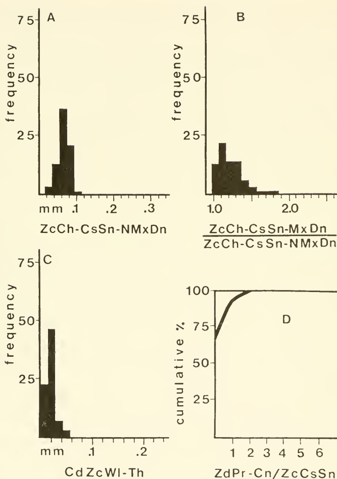
Text-figure 14 A-D. Histograms and cumulative curve from the lectotype and one topotype of Heteropora cryptopora (Goldfuss). A. Normal to maximum cross-sectional dimension of a zoecial chamber. B. Ratio of the maximum cross-sectional dimension of a zoecial chamber to the normal to maximum cross-sectional dimension of a zoecial chamber. C. Compound zoecial wall thickness. D. Count of interzooidal pores per zoecial cross section.
