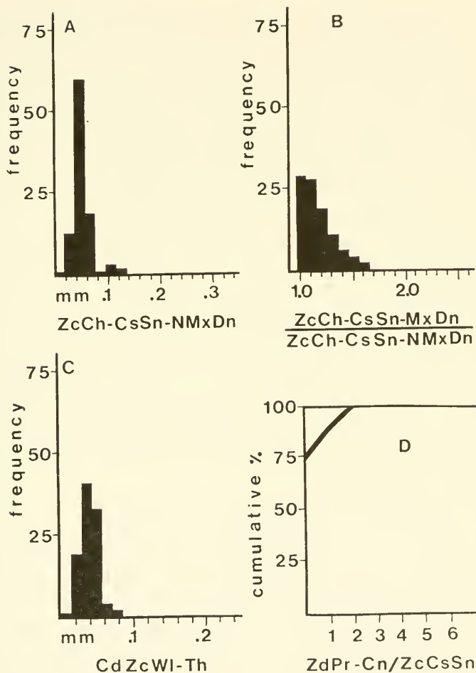
Text-figure 18 A-D. Histograms and cumulative curve from three topotypes of Tetrocycloecia dichotoma Canu. A. Normal to maximum cross-sectional dimension of a zoecial chamber. B. Ratio of the maximum cross-sectional dimension of a zoecial chamber to the normal to maximum cross-sectional dimension of a zoecial chamber. C. Compound zoecial wall thickness. D. Count of interzooidal pores per zoecial cross section.
