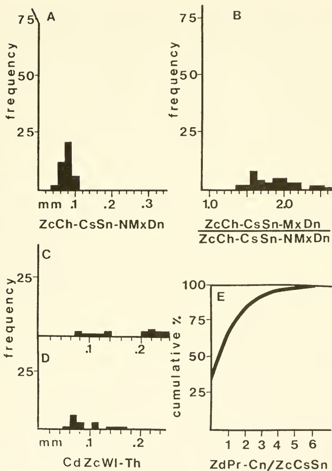
Text-figure 13 A-E. Histograms and cumulative curve from the lectotype and two topotypes of Haploecia multilamellosa (Canu and Bassler). A. Normal to maximum cross-sectional dimension of a zoecial chamber. B. Ratio of the maximum cross-sectional dimension of a zoecial chamber to the normal to maximum cross-sectional dimension of a zoecial chamber. C. Compound zoecial wall thickness as measured in longitudinal section. D. Compound zoecial wall thickness as measured in transverse section. E. Count of interzooidal pores per zoecial cross section.
