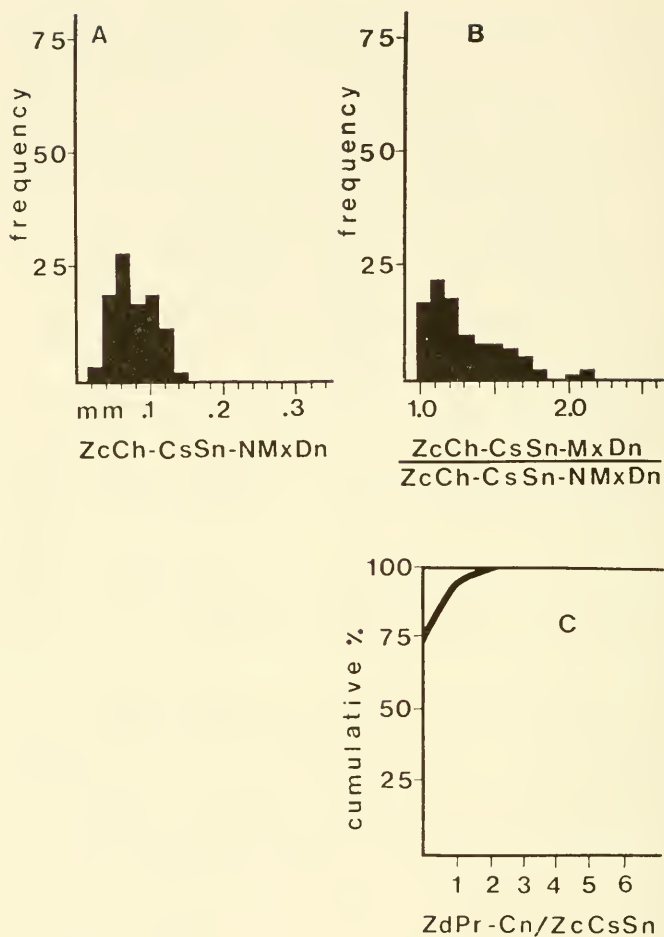
Text-figure 15 A-C. Histograms and cumulative curve from the lectotype of Lciosocia parvicella (Gabb and Horn). A. Normal to maximum cross-sectional dimension of a zooecial chamber. B. Ratio of the maximum cross-sectional dimension of a zooecial chamber to the normal to maximum cross-sectional dimension of a zooecial chamber. C. Count of interzooidal pores per zooecial cross section.
