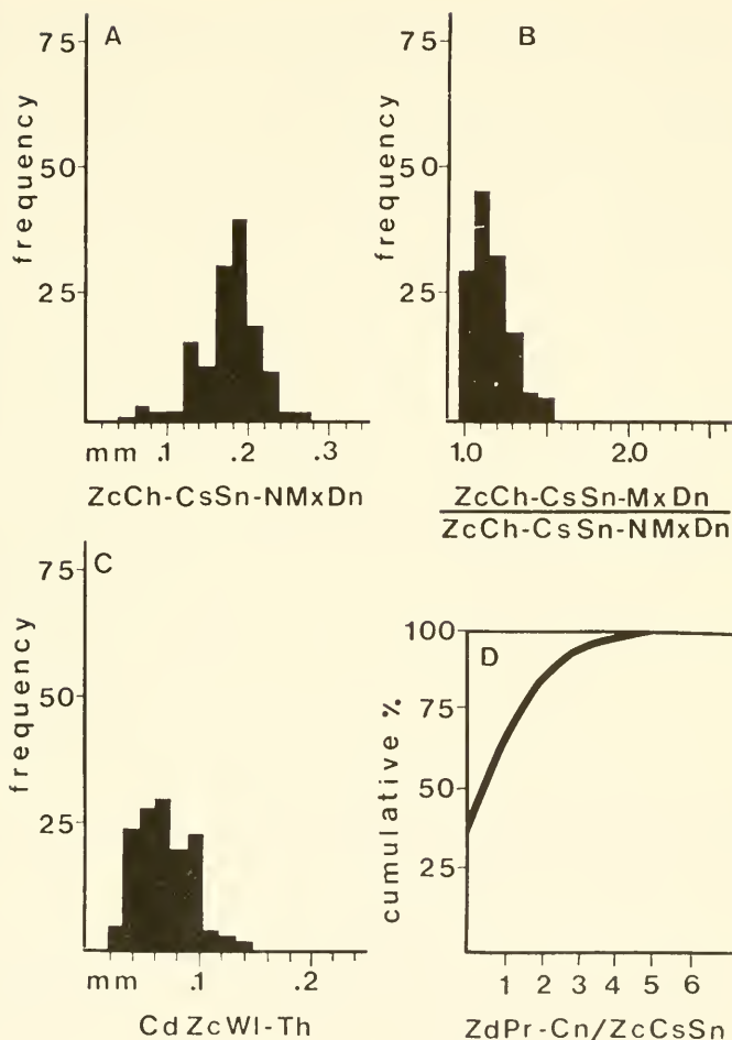
Text-figure 9 A-D. Histograms and cumulative curve from the lectotype and four topotypes of Diplocava incondita Canu and Bassler. A. Normal to maximum cross-sectional dimension of a zoecial chamber. B. Ratio of the maximum cross-sectional dimension of a zoecial chamber to the normal to maximum cross-sectional dimension of a zoecial chamber. C. Compound zoecial wall thickness. D. Count of interzoidal pores per zoecial cross section.
