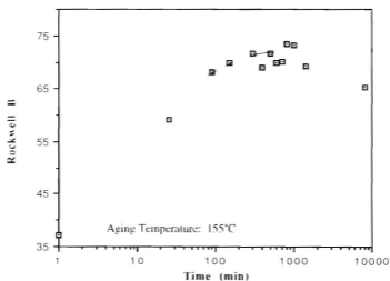
Figure 1. Aging data for A356 SiC p rolled to 24.5% reduction at 400°C.
