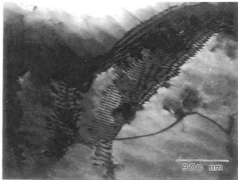
Figure 7. TEM micrograph of MMC rolled to 24.6% reduction at 400°C and 10% per rolling pass.
