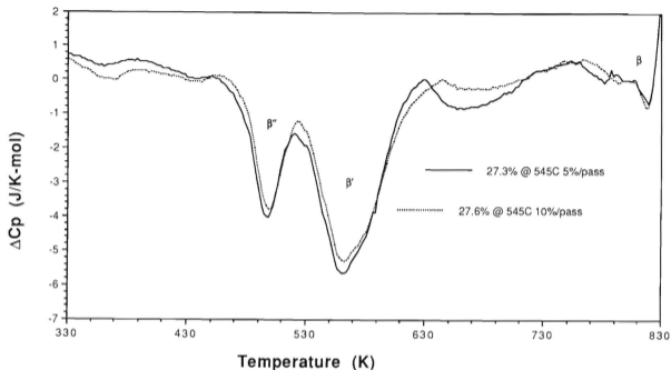
Figure 3. Effect of strain per pass in SiC p A356 Al at 545°C.
