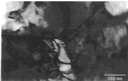
Figure 5. TEM micrograph of MMC strained 27.6% at 545°C and 10 % per rolling pass.
