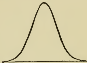
FIG. 6.—Curve showing variations in normal height. Compare with Fig. 5.
