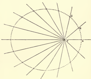
Fig. 12. Apparent Track of the Sun.
