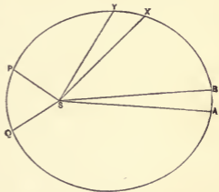
Fig. 18. The Ellipse and Kepler's Laws.
