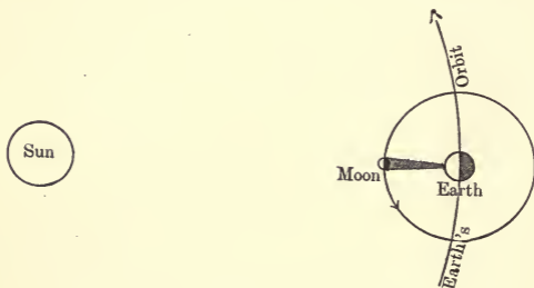
Fig. 15. Total Eclipse of Sun.
