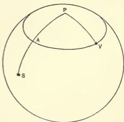
Fig. 5. Right Ascension and Declination.
