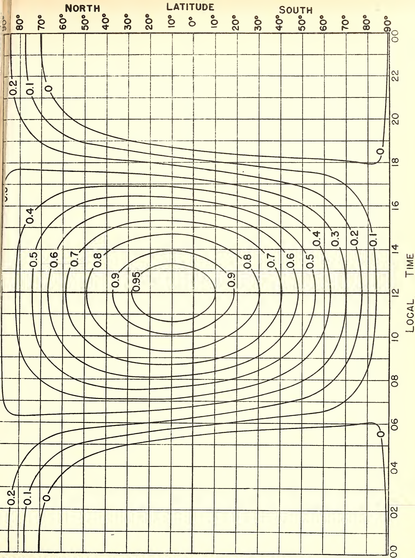
Fig.16. ABSORPTION INDEX CHART (EXCLUDING AURORAL ABSORPTION) FOR APRIL.
