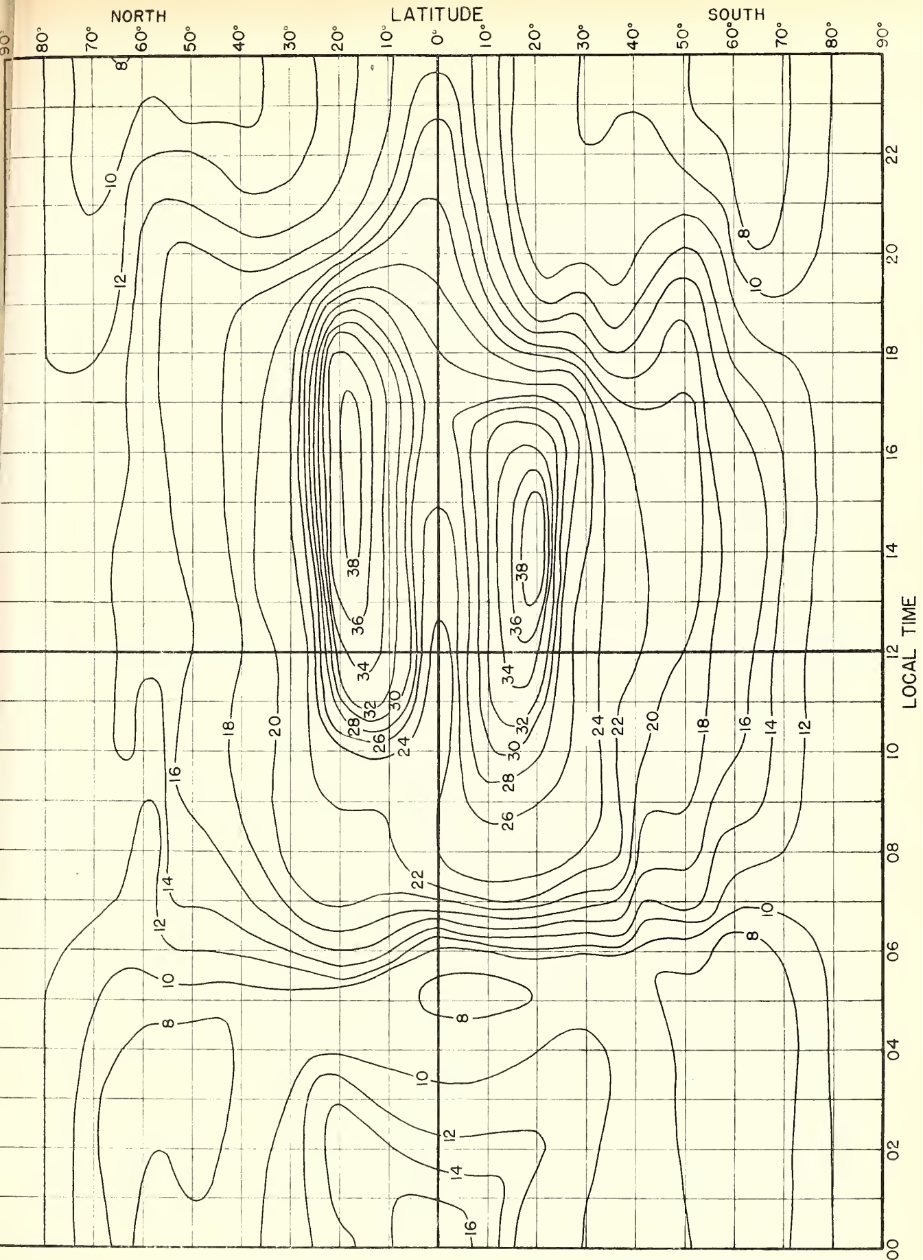
Fig. 8. F_2 4000-MUF, IN Mc, I ZONE, PREDICTED FOR APRIL, 1945.
