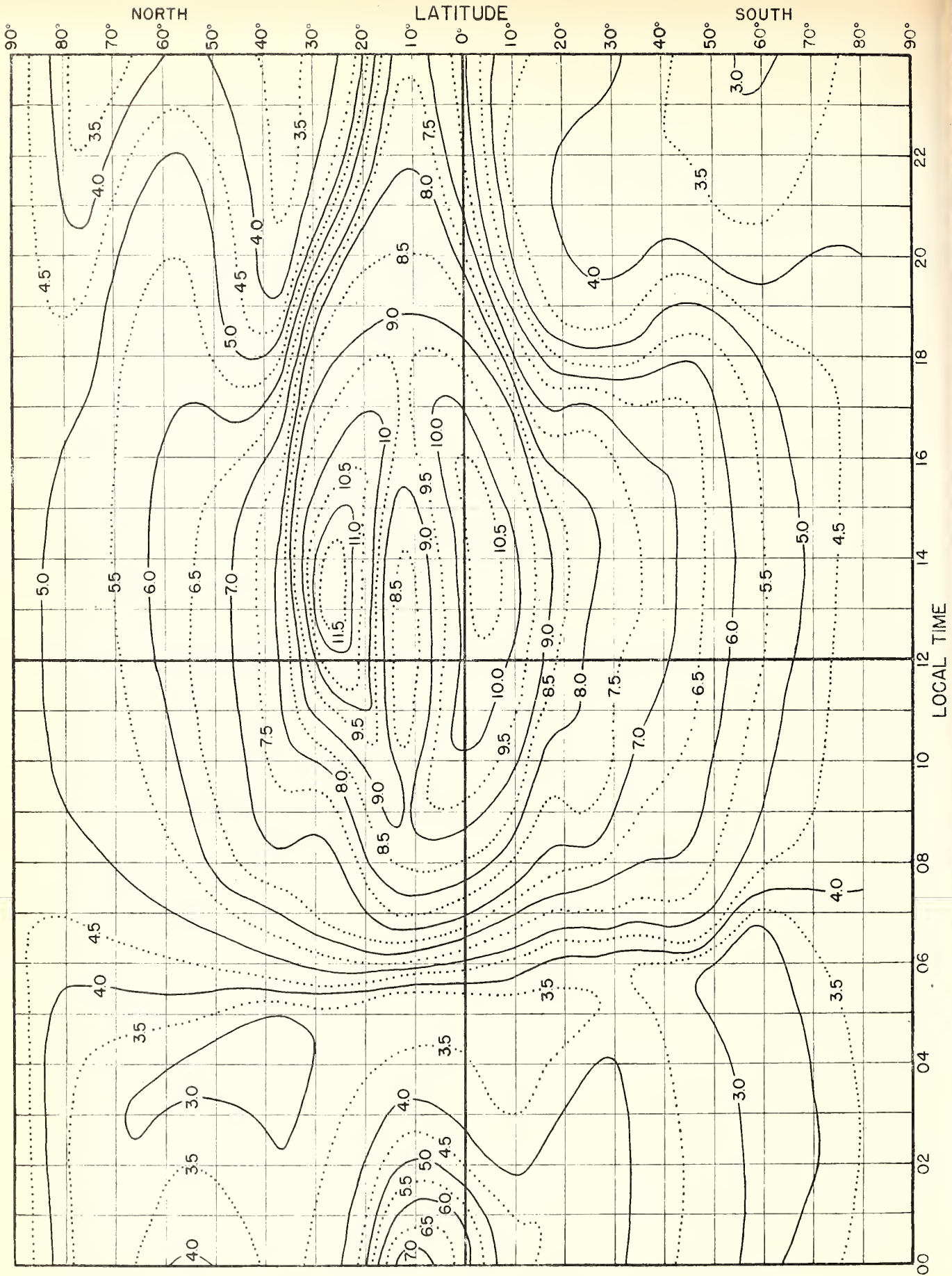
Fig. 9. F_2 ZERO-MUF, IN Mc, E ZONE, PREDICTED FOR APRIL, 1945.
