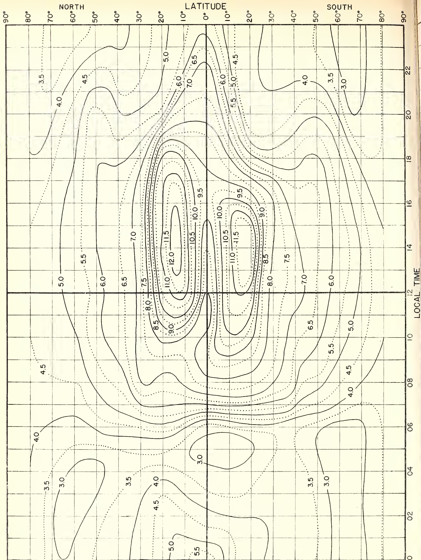
Fig 7. F 2 ZERO-MUF, IN Mc, I ZONE, PREDICTED FOR APRIL, 1945.
