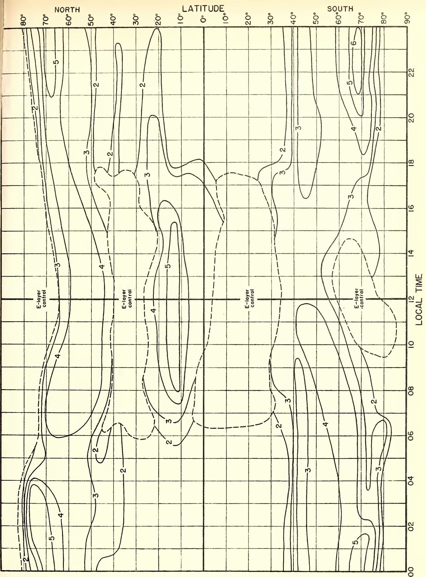
Fig. 12. MEDIAN fE_s , IN Mc, PREDICTED FOR APRIL, 1945.
