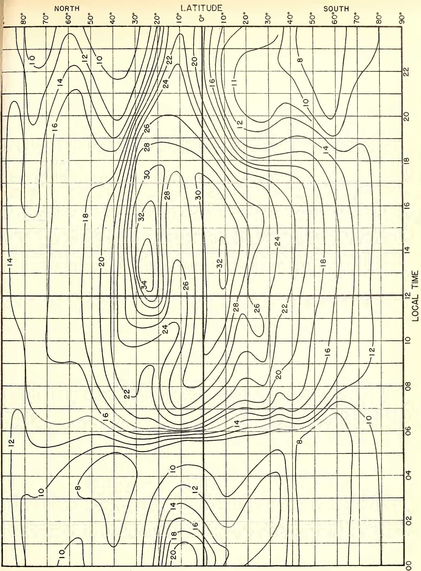
Fig. 10. F_2 4000-MUF, IN Mc, E ZONE, PREDICTED FOR APRIL, 1945.
