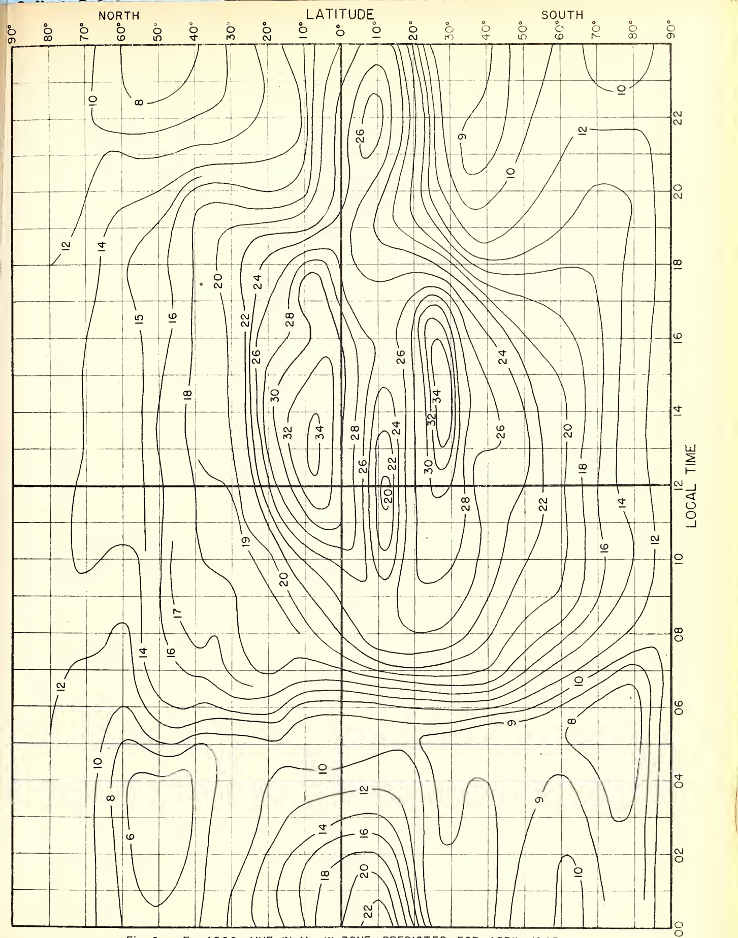
Fig. 6. F_2 4000-MUF, IN Mc, W ZONE, PREDICTED FOR APRIL, 1945.
