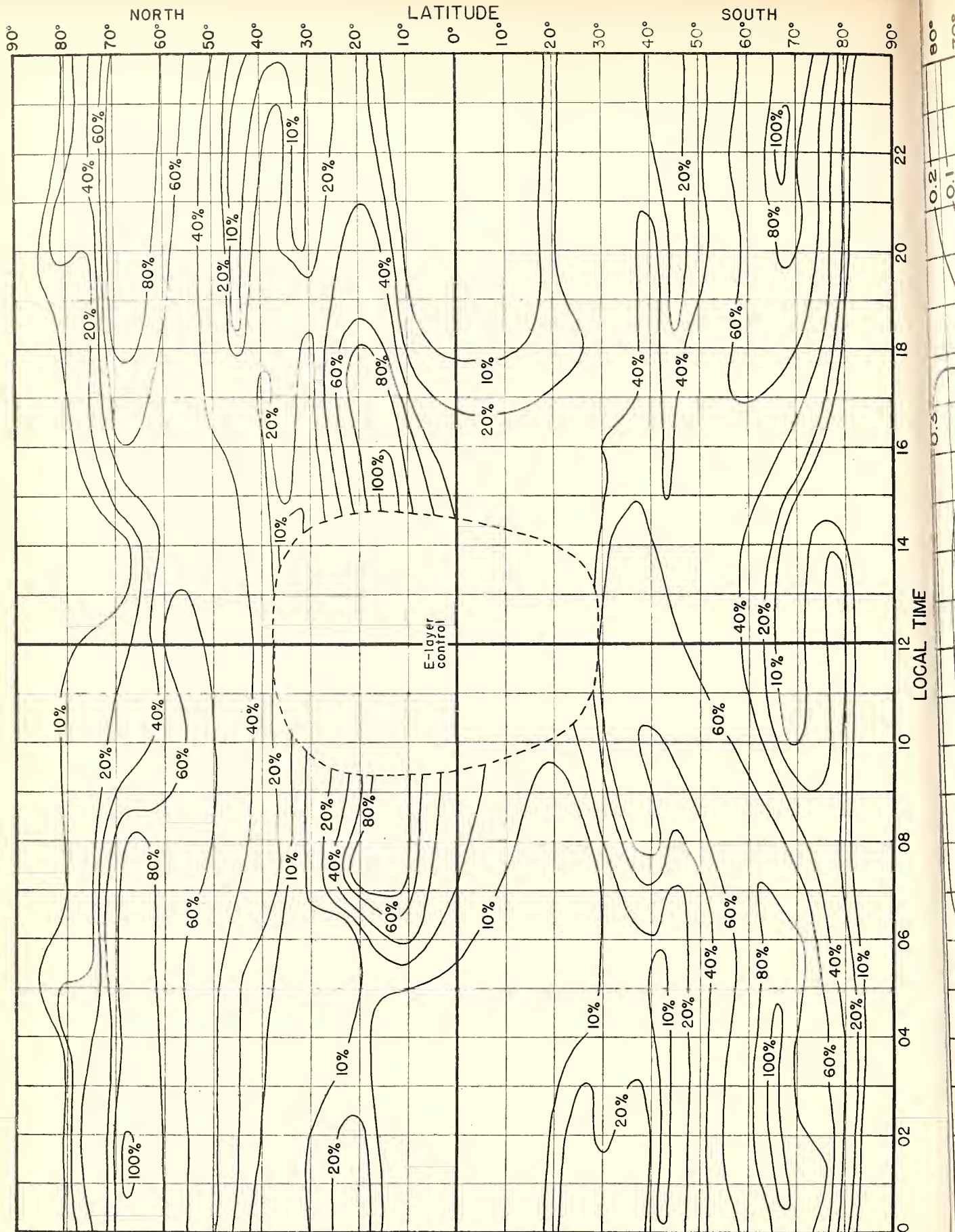
Fig. 15. PERCENTAGE OF TIME OCCURRENCE FOR E s IN EXCESS OF 15 Mc, PREDICTED FOR APRIL, 1945.
