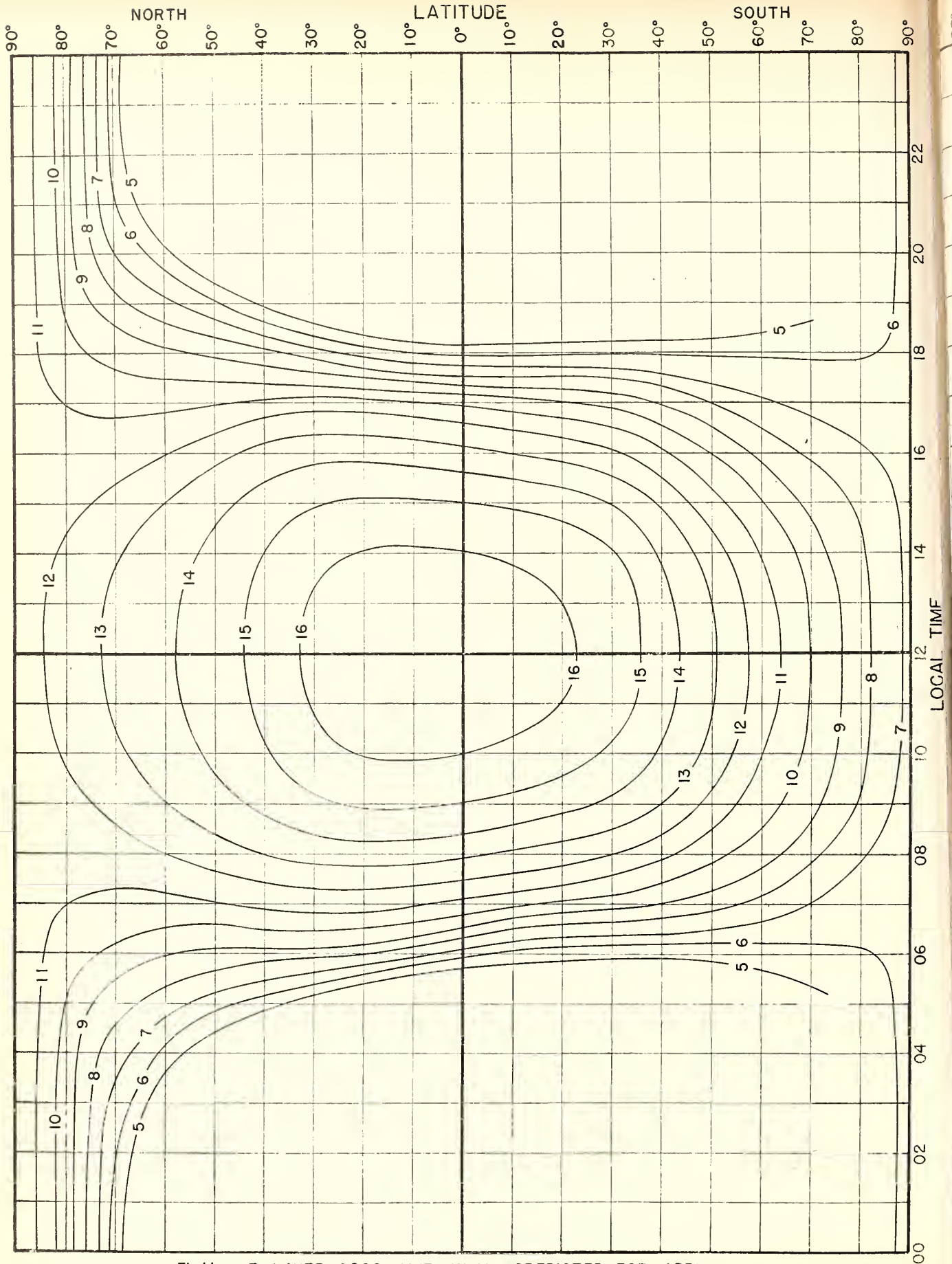
Fig.11. E-LAYER 2000-MUF, IN Mc, PREDICTED FOR APRIL, 1945.
