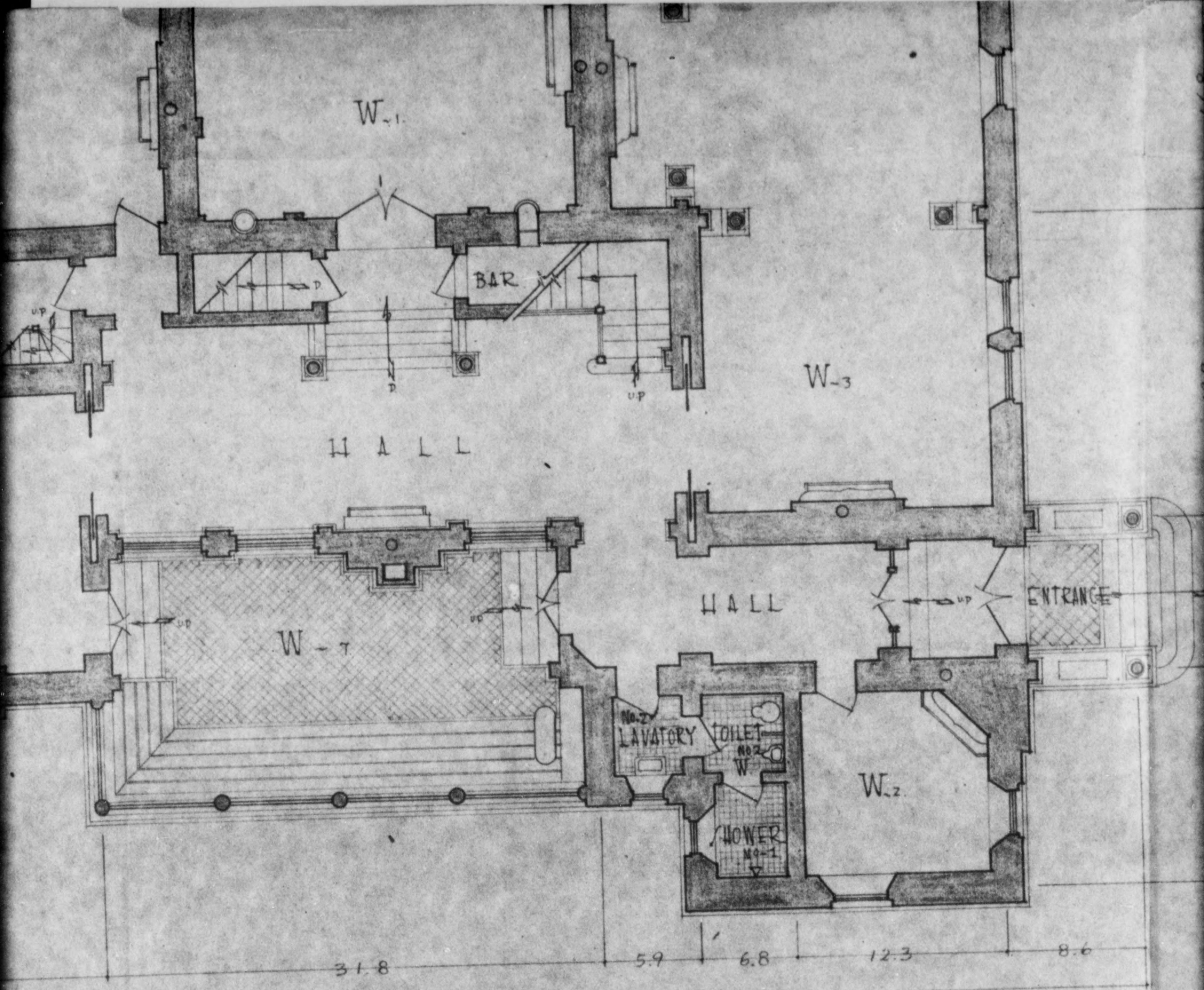
FIRST - FLOOR
