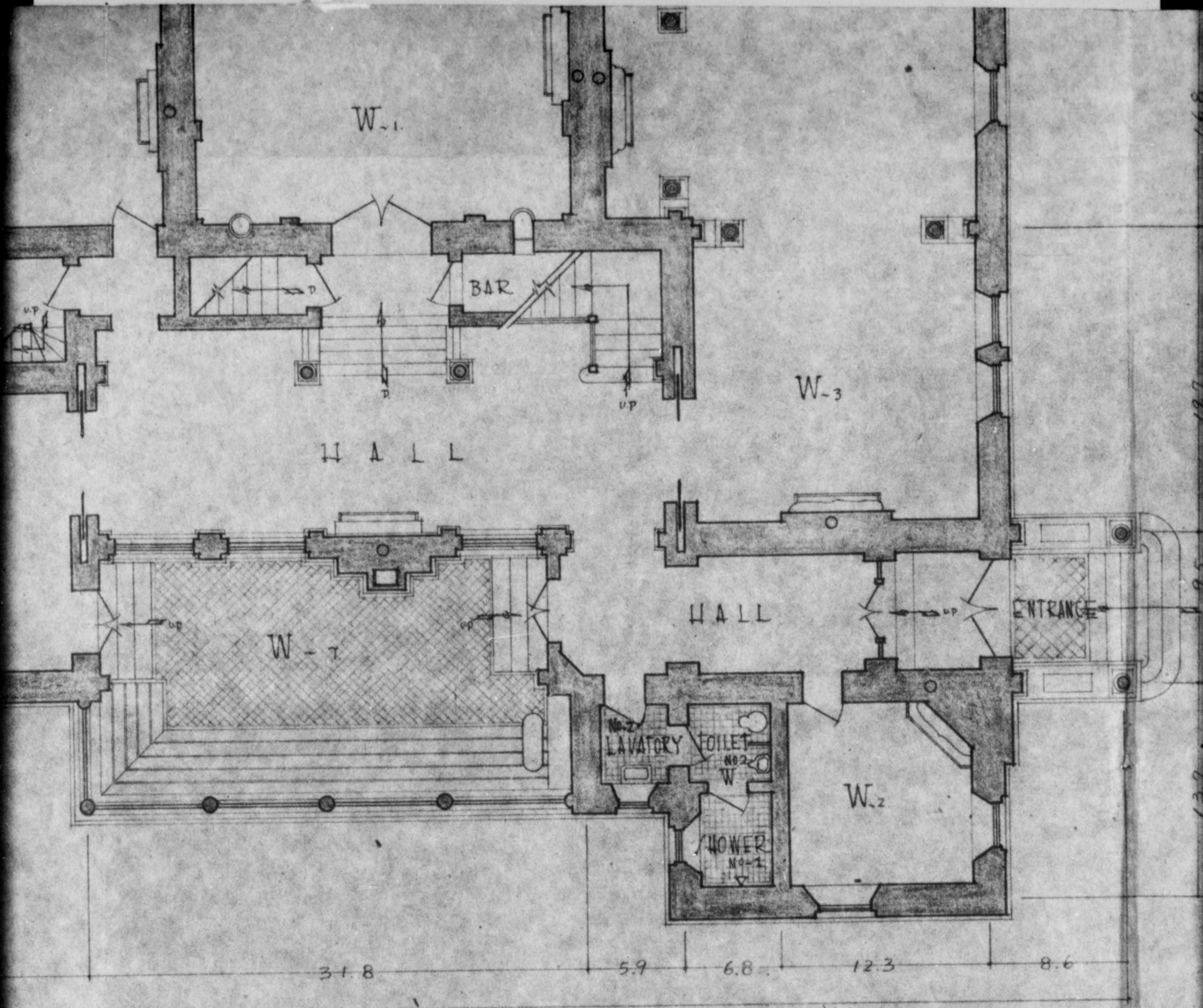
FIRST FLOOR
