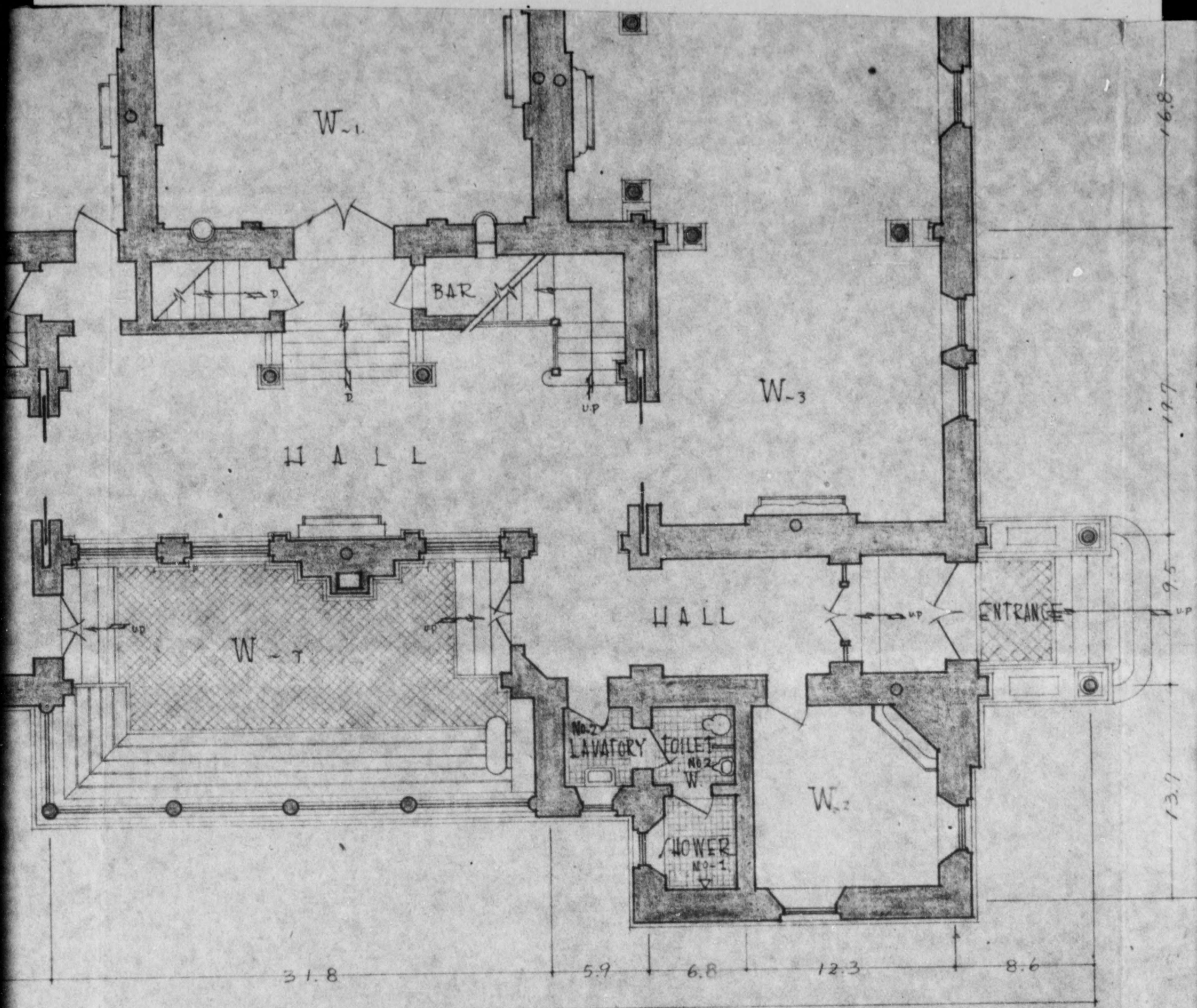
FIRST - FLOOR
