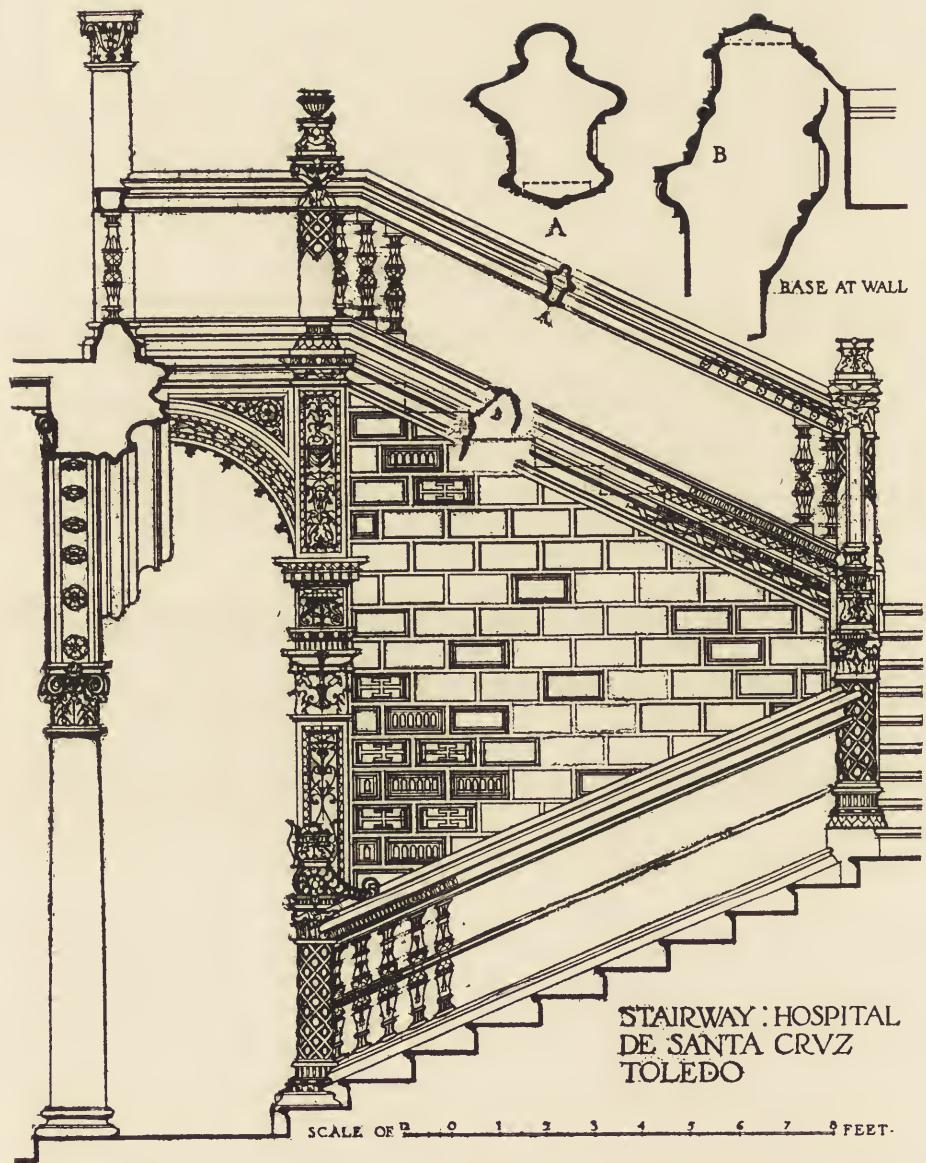
SECTION THROUGH STAIRWAY OF THE HOSPITAL DE SANTA CRUZ, TOLEDO.
