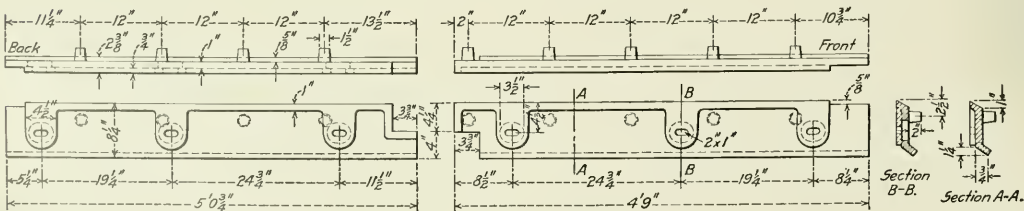
Fig. 7—Grate Side Bearing Bars.
