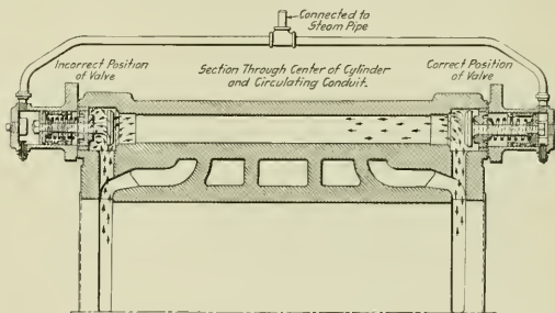
Section Through Drifting Valves and Passage Showing the Action for the Correct and Incorrect Positions.
