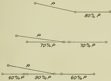
Diagram VI—Loading of Side Rods for Strength of Rods and Stubs.
