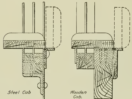
Fig. 2—Hinged Arm Rest.
