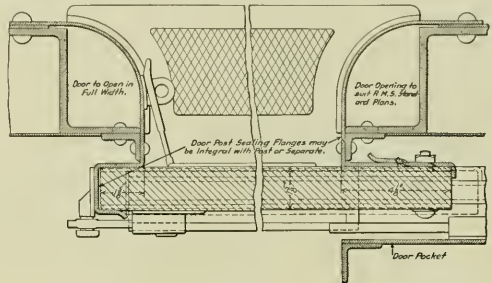
Horizontal Section Through Rumsey Postal Car Door.
