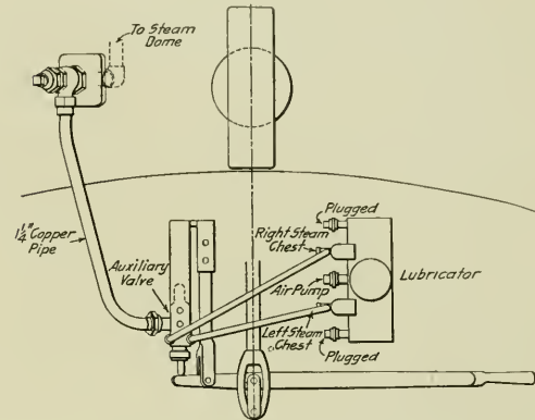
MacBain Auxiliary Lubricator Valve.
