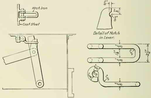
Fig. 4—Drop Gate Lever Keeper.
