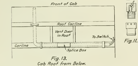
Details of Electric Wiring Installation for Headlights.
