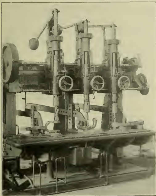
Thomson Pneumatic Clamps Applied to a 3-Spindle Foote-Burt Drill.
