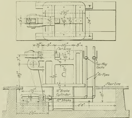
Fig. 2—Pneumatic Bulldozer for the Smith Shop.
