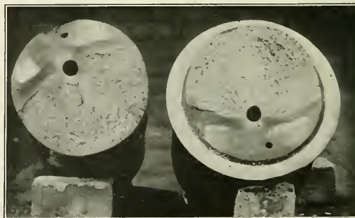
Fractured Crank Pin Discovered by Means of the Detector.
