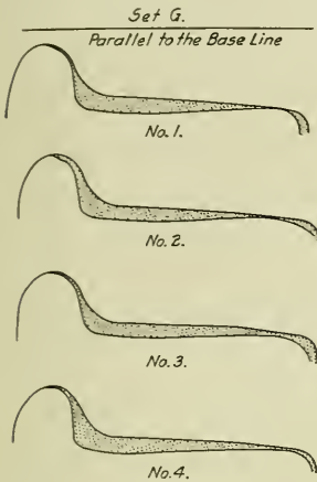
Fig. 7—Set G: Non-mated Old Cast Iron Wheels.
