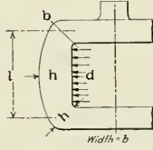
Solid End Stubs, Main or Side and Solid End Jaw Stubs.
