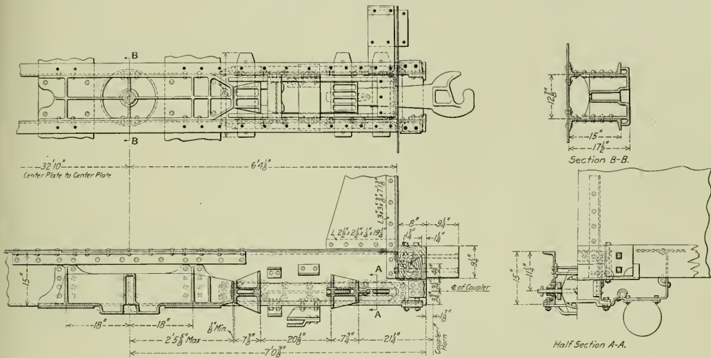
Arrangement of Draft Gear on 90-Ton Gondola Car; Norfolk & Western.
