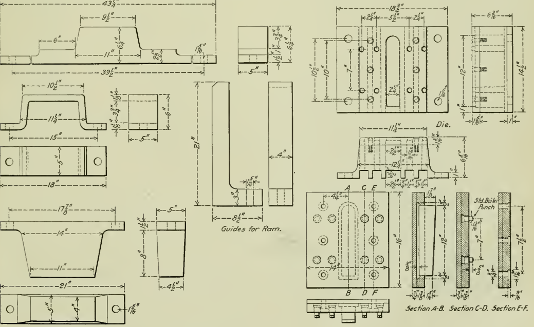
Details of Dies and Supports Used for Punching Spring Planks on a Hydraulic Press.
