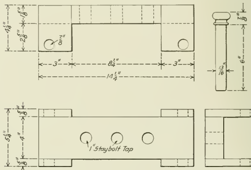
Tool for Bending Eccentric Blades.
