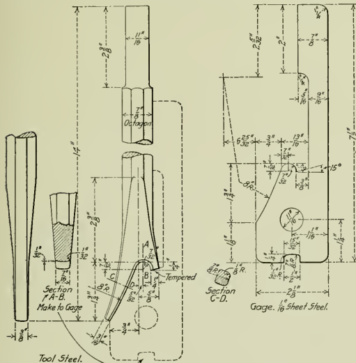
Fig. 26—Beading Tool for Brick Arch Tubes.
