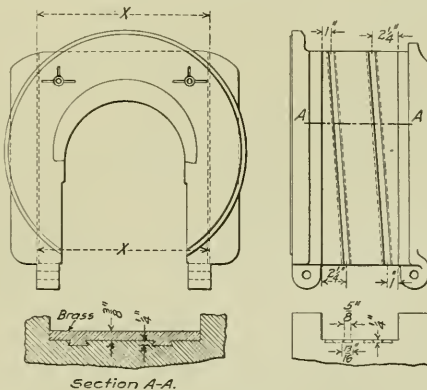
Brass Liner for Shoe and Wedge Fit of Driving Box.
