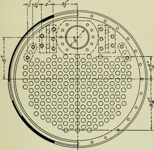
180, 1 1/2" Tubes, 2 3/8" Pitch.
