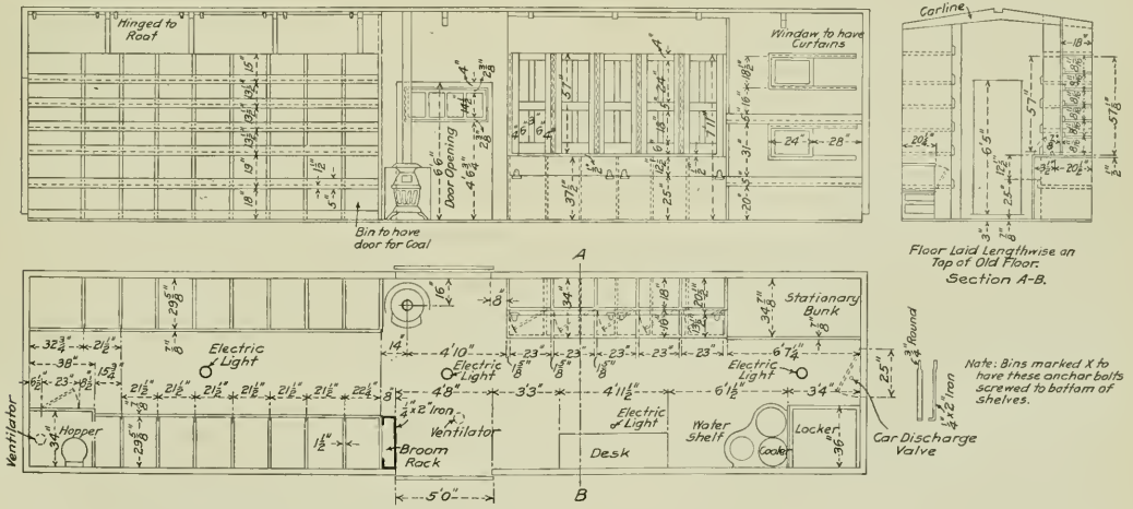
Standard General Supply Car—Southern Pacific.
