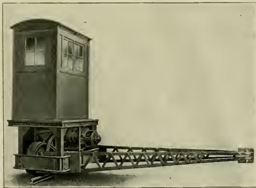
Fig. 4—Turntable Tractor.
