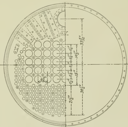
43.5" Flues Holes Drilled 5/32" Diam. 295, 2" Tubes, 2" Pitch Holes Drilled 1/8" Diam. Tubes Marked Thus + Beaded Over.
