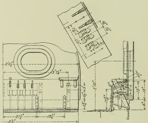
Fig. 4—Deck Shield for Locomotive with Wootten Type Boiler.
