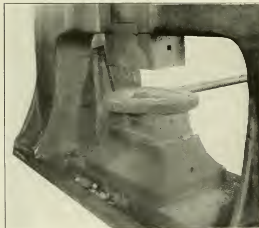
Die in Position for Punching Out the Main Part of the Transom End.
