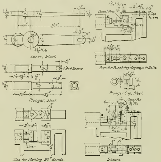
Fig. 3—Details of Pneumatic Bulldozer, with Some of the Dies Used.
