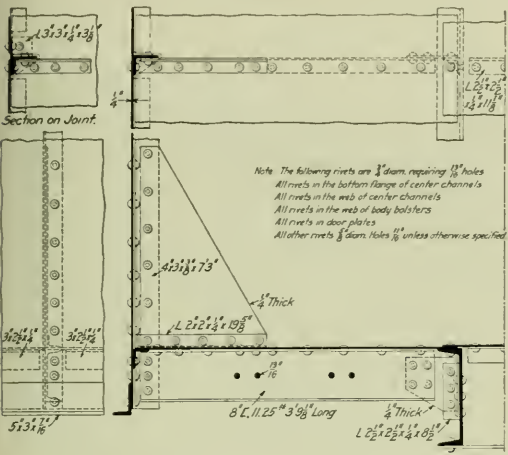
Detail Showing Arrangement of Floor Beams.
