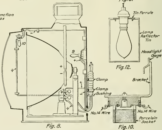
Details of Electric Wiring Installation for Headlights.
