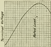
Load Current Curve of Series Generator Fig. 7.
