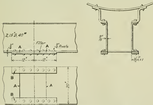
Fig. 1—A Useless Attempt at Reinforcement.
