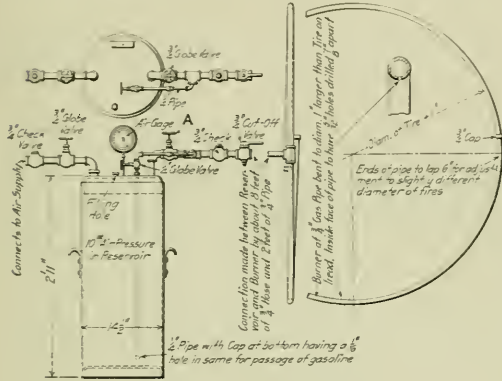
Fig. 1—Gasolene Tire Heater.
