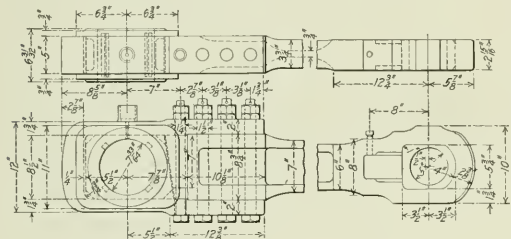
Strap End Main Rod; Chicago & North Western.
