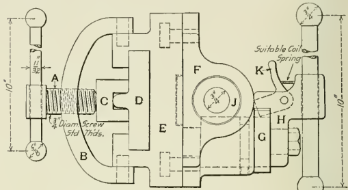
Apparatus for Drilling Tell-tale Holes in Staybolts.
