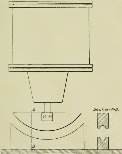
Brake Cylinder Fitted for Bending Pipe.
