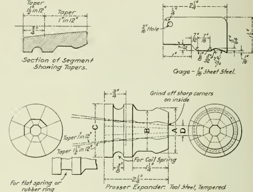
Fig. 13—Prosser Expander for Tubes 2, 2 1/4 and 2 1/2 in. in Diameter.
