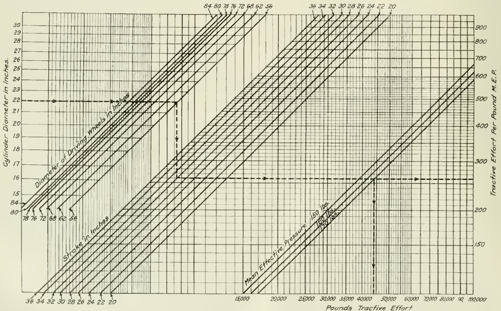
Tractive Effort Chart Giving the Pounds Pull for Any Size of Locomotive.
