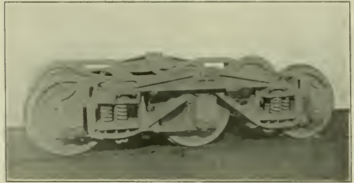
Side View of the Six-Wheel Truck Complete.
