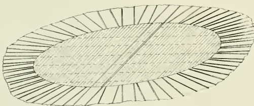
Turntable Pit Completely Covered by Revolving Floor Attached to Turntable and with Space Between Rails in Central Area Paved to the Level of the Tops of the Rails.
