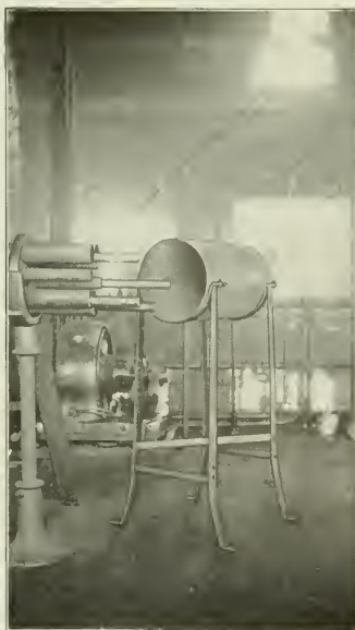
Fig. 4—Guard for Ends of Rods in Automatic Machine.
