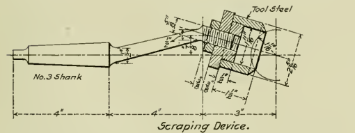
Successful Tool for Finishing the Ball Joint on Unit Pipes.
