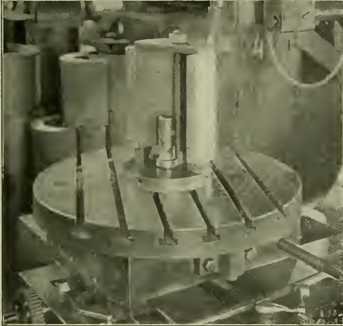
Fig. 1—Attachment for Slotting Driving Box Brasses.
