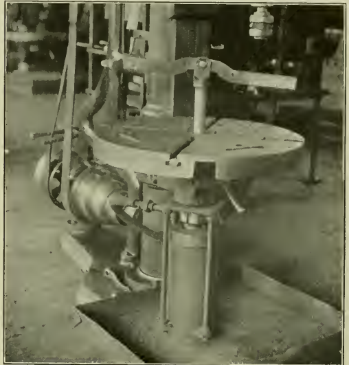
Fig. 3—Pneumatic Clamp for Drill Press.
