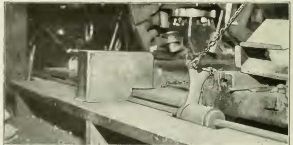
Fig. 16—Foot Guard on Wheel Lathe.
