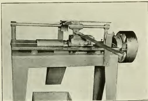
Brass Boring Machine Ready for Operation.
