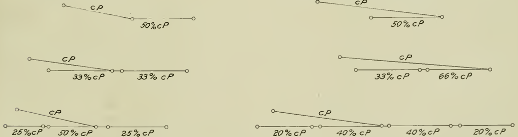
Diagram VII—Loading of Side Rods Due to Reduced Main Rod Load C P (Diagram III). Locomotive Travelling at High Speed.
