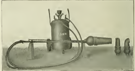
Fig. 1—Mahr Oil Burner for Car Repairs.
