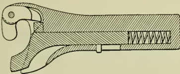
New Design of Automatic Car Coupler.
