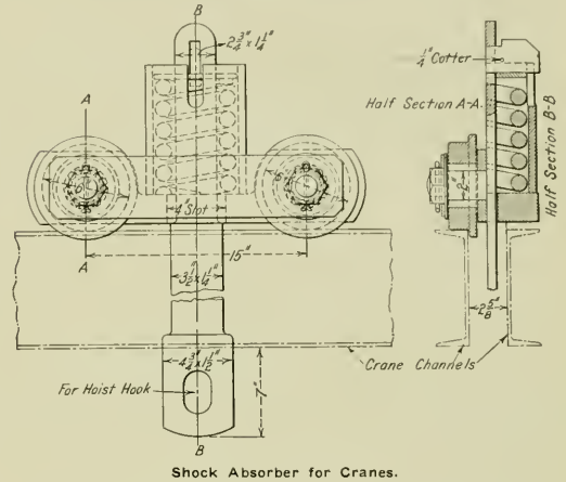
Shock Absorber for Cranes.
