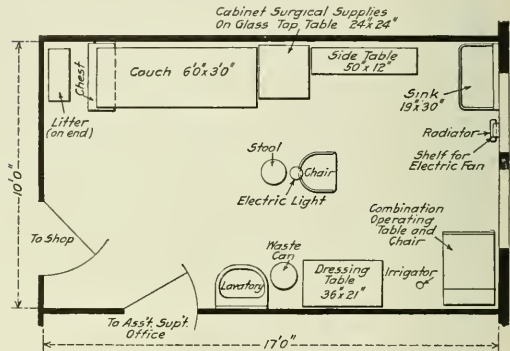
Plan of Hospital Room at the Rock Island Shops, Silvis, Ill.
