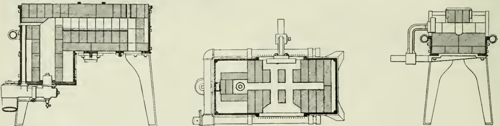
Fig. 6—General Construction of Ferguson Flue Welding Furnace.
