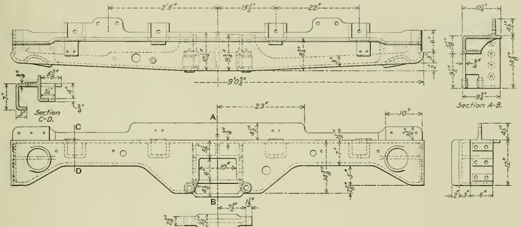
Cast Steel End Sills for Jersey Central Gondola.
