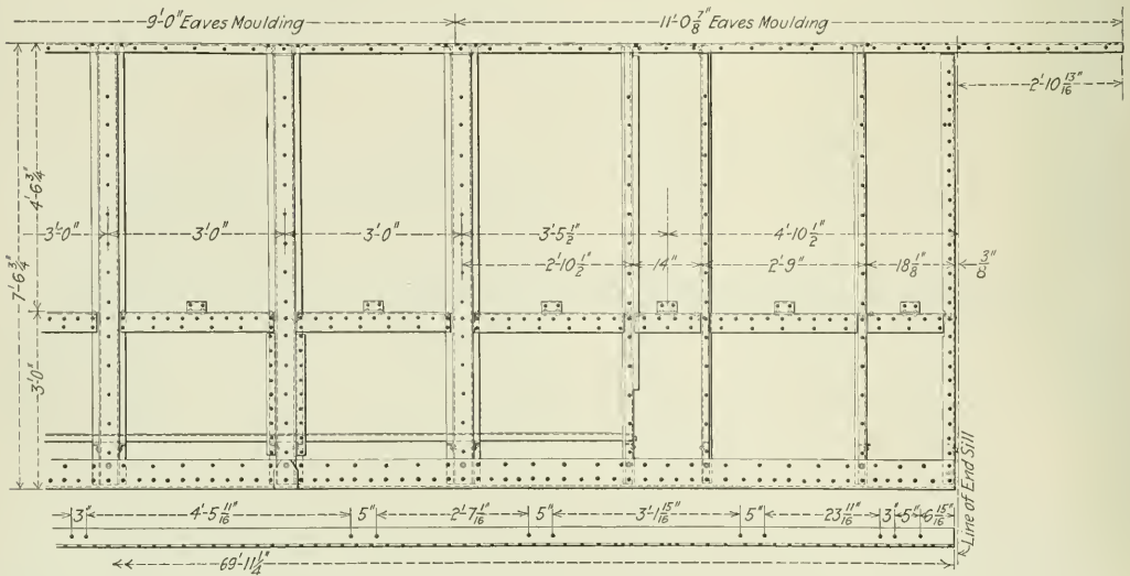
Elevation of Body Side Framing at End of Car; New York Central Lines Steel Coach.
