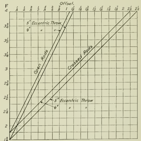
Curves for Determining the Base from Which the Proper Saddle Pin Offset Can Be obtained.
