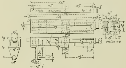
Fig. 1—Table Grate Bar.
