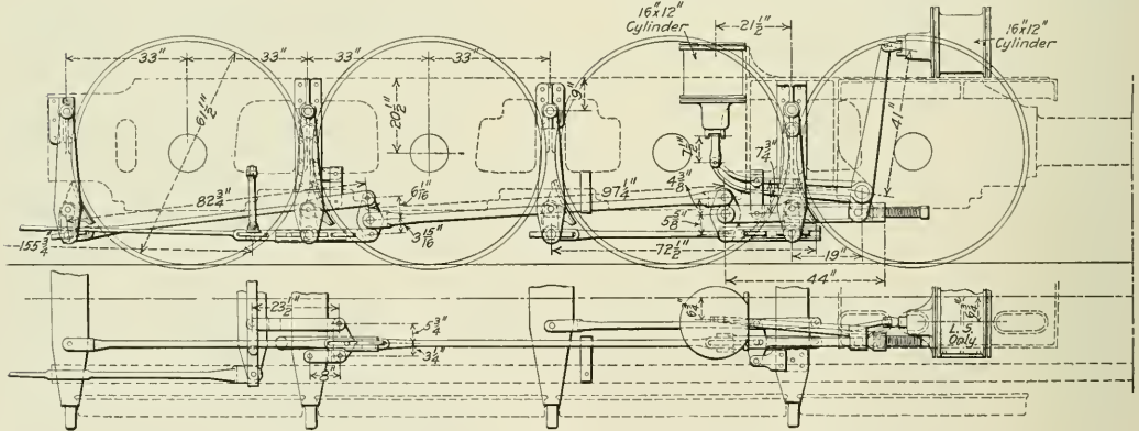
Arrangement of Brake Rigging Which Includes a Connection to the Trailing Truck.
