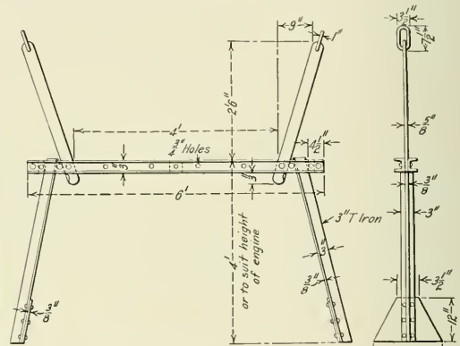
Rack For Handling Tubes Rack Used for Boiler Tubes.
