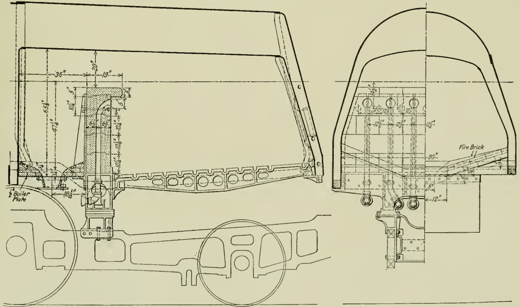
Arrangement of Gaines Combustion Chamber on Illinois Central Mikado.
