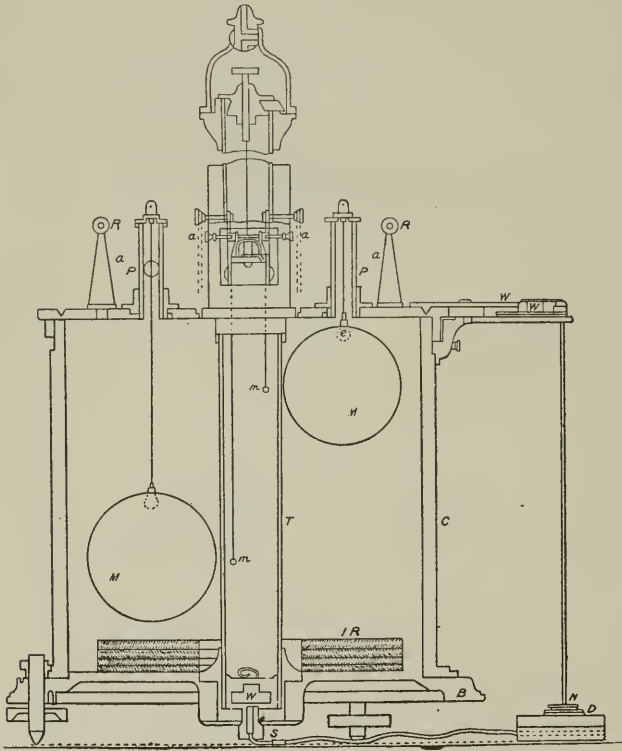
FIG. 2.—Boys's apparatus.
