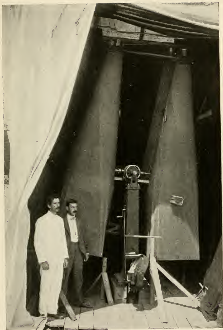
THE INTRA-MERCURIAL PLANET APPARATUS OF THE SMITHSONIAN INSTITUTION.
