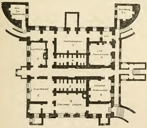
Bushy House, basement.
