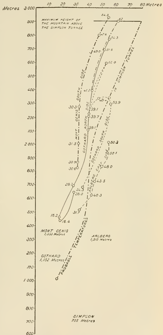
Fig. 5.—Curves showing depths corresponding to an increase in temperature of 1° C. for the Mout Genis, Gothard, and Arlberg tunnels (with curve of probable temperature for the Simplon Tunnel).
