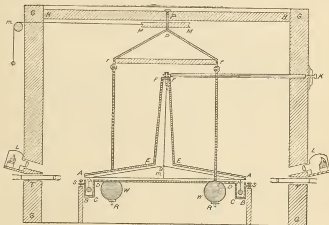
FIG. 1.—Cavendish's apparatus.
