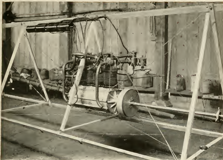
SIXTEEN-HORSEPOWER PETROLEUM MOTOR OF SANTOS-DUMONT V, GIVING SCREW 200 REVOLUTIONS PER MINUTE.
