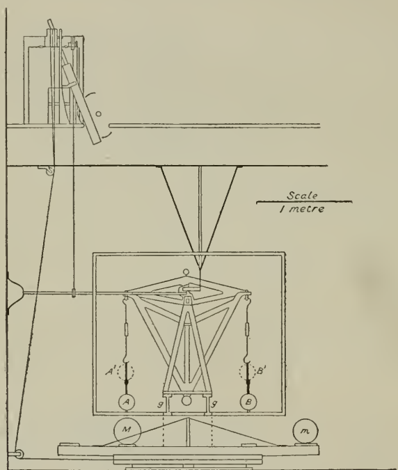
FIG. 3.—Common balance experiment (Poynting).
