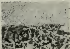
FIG. 4.—SECTION OF BAD RAIL, SHOWING SURFACE TO WHICH FRACTURE WAS DUE.
