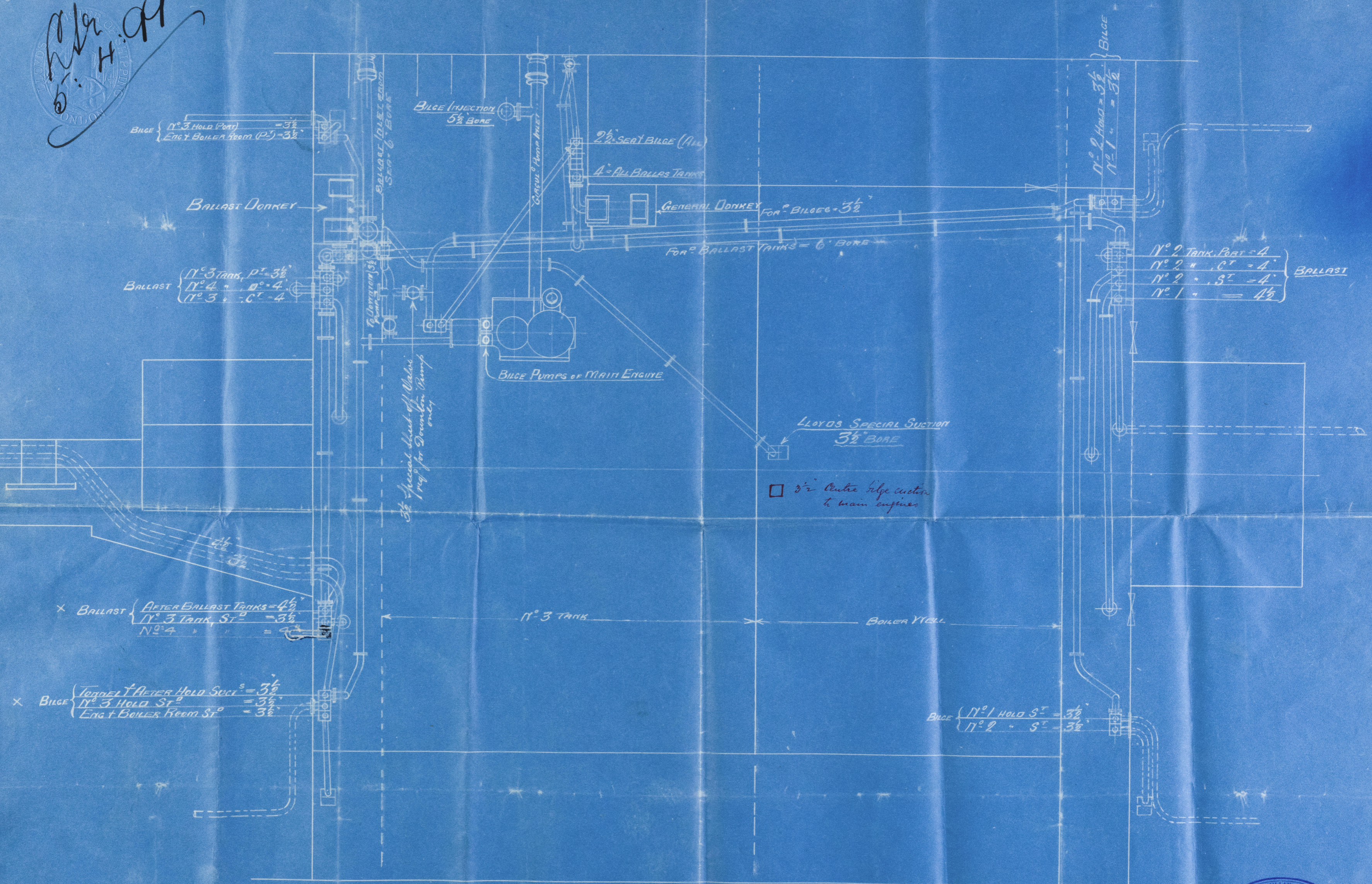
Arrang t of Bilge & Ballast Pipes in Ship N o 367 Engine N o 214 Scale 1/4" = 1 foot
