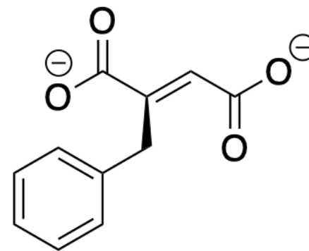
( R )-Benzylsuccinate
