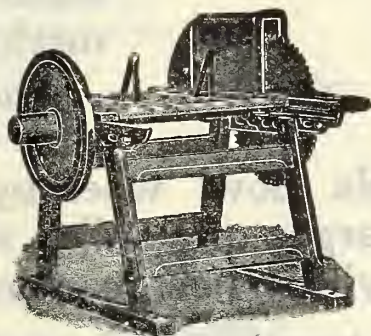
SLIDING TABLE WOOD SAW Weight, 300 Pounds
