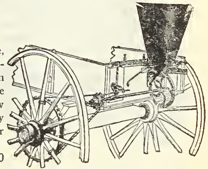
John Deere No. 999 Two-Row Corn Planter
