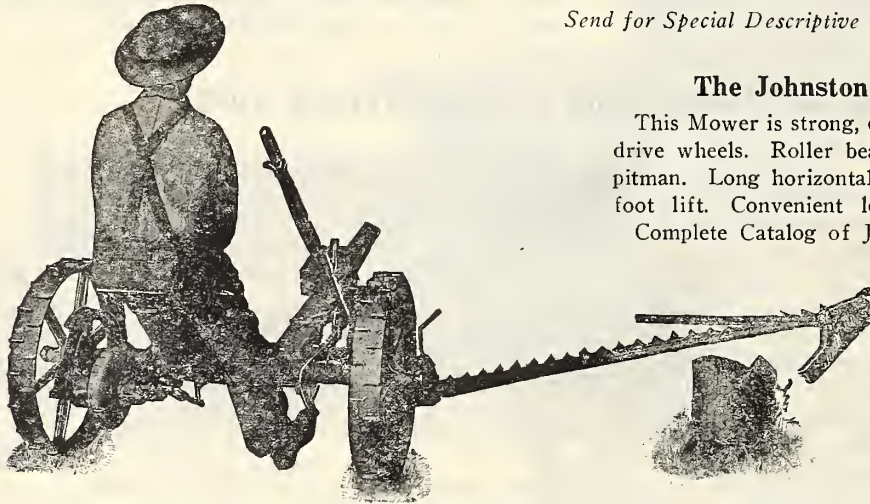
Showing Ease of Handling Johnston Lever Fold Mower in Passing Over Obstruction
