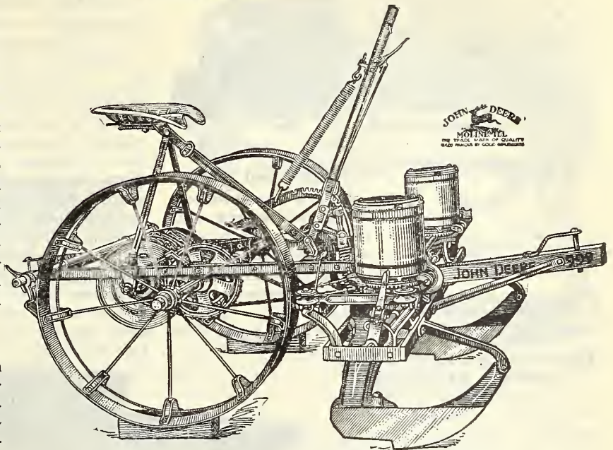
John Deere No. 999 Two-Row Corn Planter
