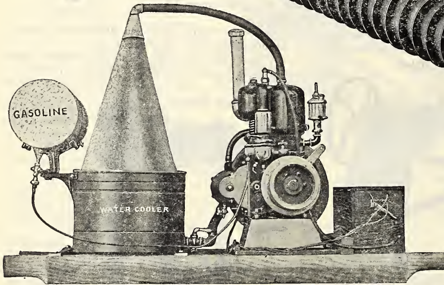
4 H. P. Cushman Engine
