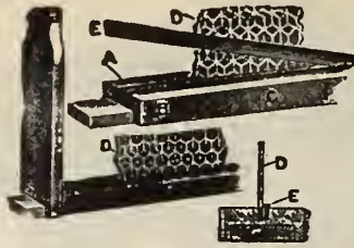
Manner of fastening foundation in latest improved Hoffman frame with the little wedge.
