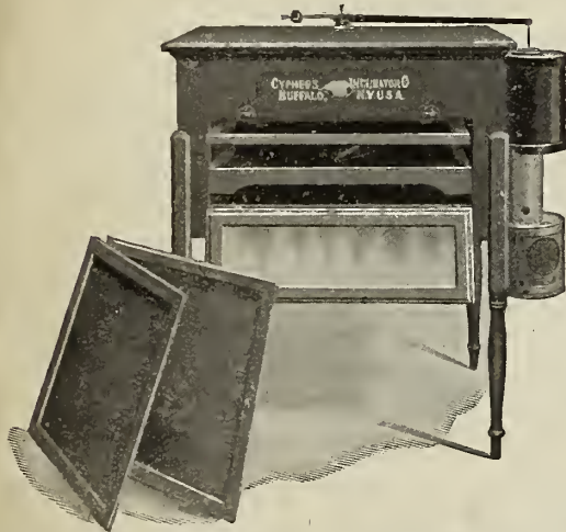
No. 1 Standard Cyphers Incubator, Fire-Proofed, Insurable, 144-egg capacity. Showing, "split" lower diaphragm removed, egg tray and upper diaphragm partly drawn out.
