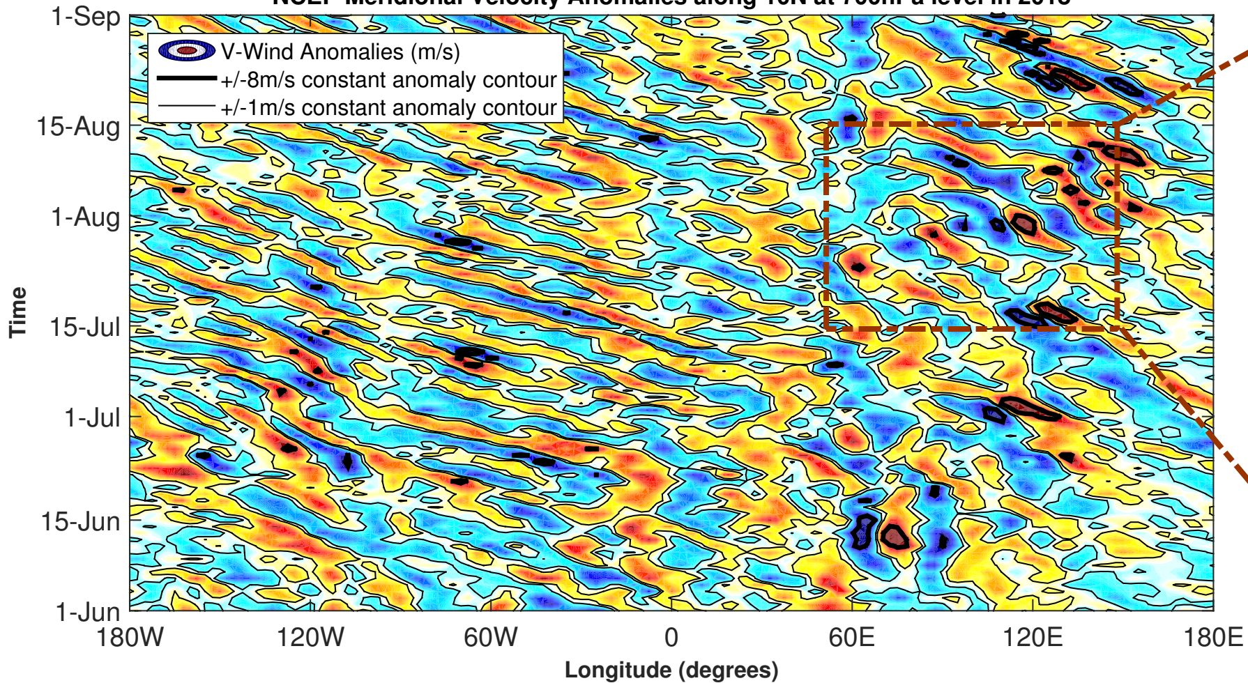
NCEP Meridional Velocity Anomalies along 10N at 700hPa level in 2018
