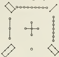
The lo-shu .
