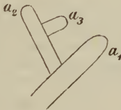
Fig. 13. Sympode monopodial.
