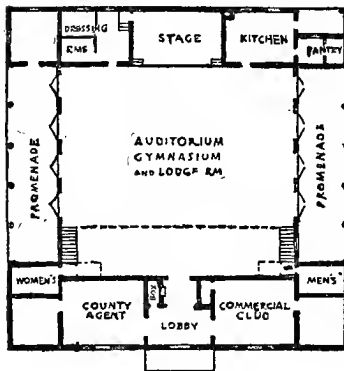
MAIN-FLOOR PLAN
