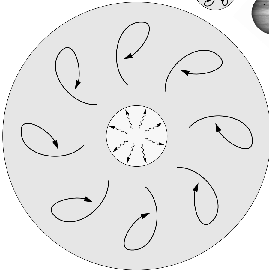
Gliese 752A Thermal Structure
