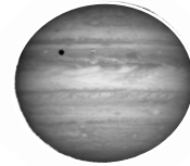
Jupiter to scale
