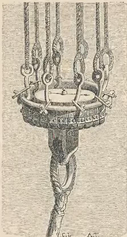
FIG. 1. THE WEIGHING MACHINE OF THE "CAPTIVE."
