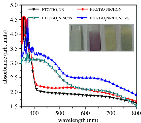
Figure 6. UV–vis absorption spectra and photographs of TiO 2 NR, TiO 2 NR/HGN, TiO 2 NR/HGN/CdS and TiO 2 NR/CdS hybrids. The electrophoretic deposition time of HGNs was 13 min, and the number of SILAR cycles applied to deposit CdS was 7.
