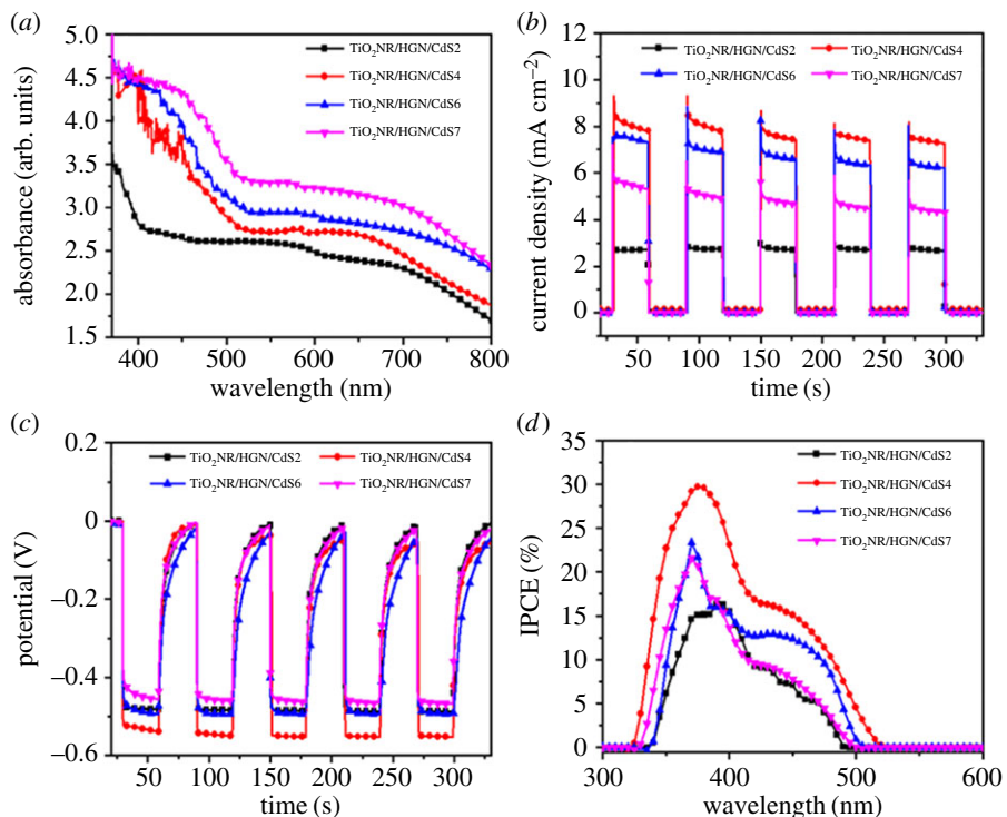
Figure 8. (a) UV-vis absorption spectra, (b) photocurrent density, (c) open-circuit voltage and (d) IPCE of TiO 2 NR/HGN/CdS hybrids with different numbers of SILAR cycles applied to deposit CdS. The electrophoretic deposition time of HGNS was 7 min.
