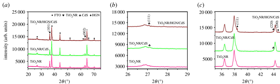
Figure 4. (a) XRD patterns of TiO 2 NR, TiO 2 NR/CdS and TiO 2 NR/HGN/CdS. Detailed XRD patterns of these three samples in the range (2θ) (b) from 26° to 29° and (c) from 36° to 45°. The electrophoretic deposition time of HGNs was 13 min, and the number of SILAR cycles applied to deposit CdS was 7.
