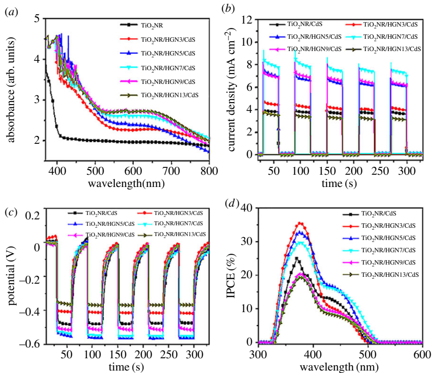
Figure 7. (a) UV-vis absorption spectra, (b) photocurrent density, (c) open-circuit voltage and (d) IPCE of TiO 2 NR/HGN/CdS hybrids with varied amounts of HGNS conducted by varied electrophoretic deposition times. The number of SILAR cycles applied to deposit CdS was 4.
