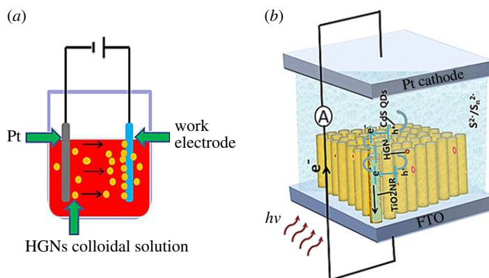
Figure 1. (a) Schematic of surface decoration strategy of \text{TiO}_2 nanorods electrodes based on electrophoretic deposition in the HGNS colloidal solution. The DC voltage was 35 V. (b) Schematic of separation and transfer of electron-hole pairs in CdS QD-sensitized \text{TiO}_2 solar cell with plasmonic HGNS.
