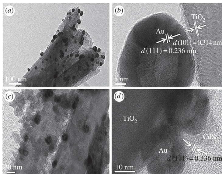
Figure 5. TEM images of (a) TiO 2 NR/HGN and (c) TiO 2 NR/HGN/CdS hybrids. High-resolution TEM images of (b) TiO 2 NR/HGN and (d) TiO 2 NR/HGN/CdS hybrids.
