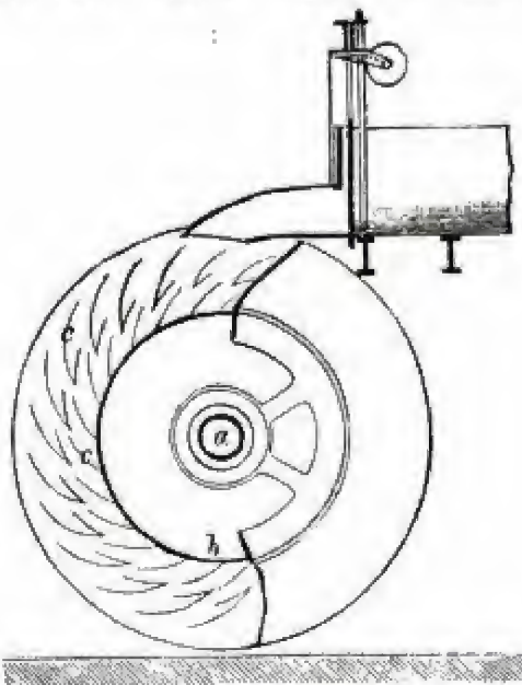
Diagram of Hydrovalve.
