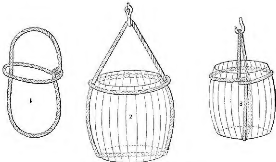
Slinging a Cask Having One Head Out
