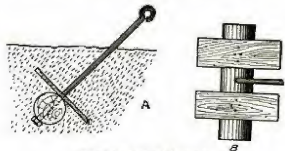
Best Method of Guying
