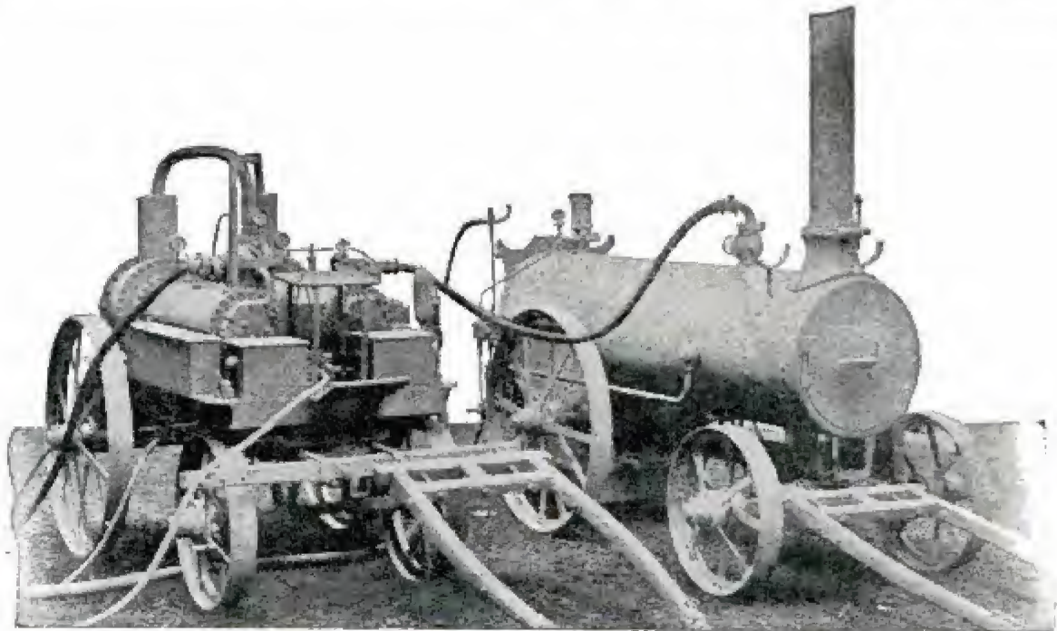
Produces 65 Gallons of Pure Distilled Water Per Hour
