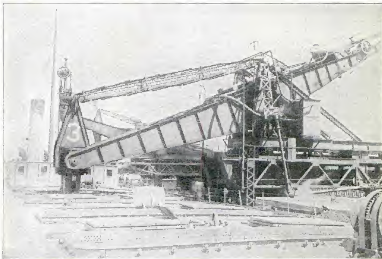
How the Bucket is Lowered into the Hold—Showing the Operation of the Walking-Beam
