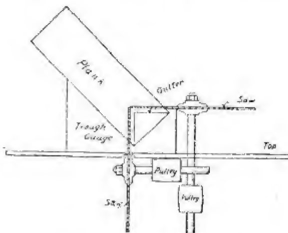
Device for Sawing Wood Gutters
