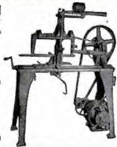
A Roth Motor Drives this Hackaw.
