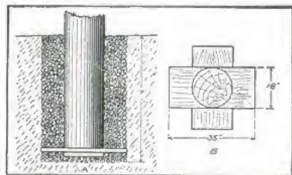
Setting Poles in Soft Ground.
