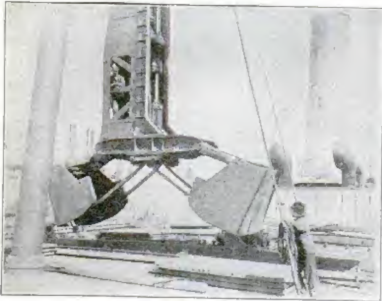
Clam-Shell Bucket Open
