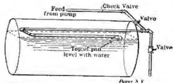
BOILER FEED AND BLOW-OFF ARRANGEMENT.
