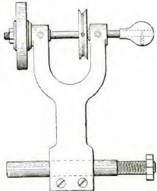
Machine for Truing Collector Rings
