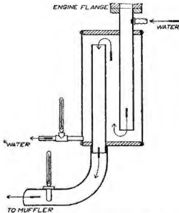
Method of Measuring Waste Heat from Gas Engines.
