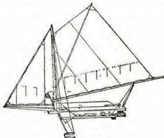
Plan of Ice Boat
