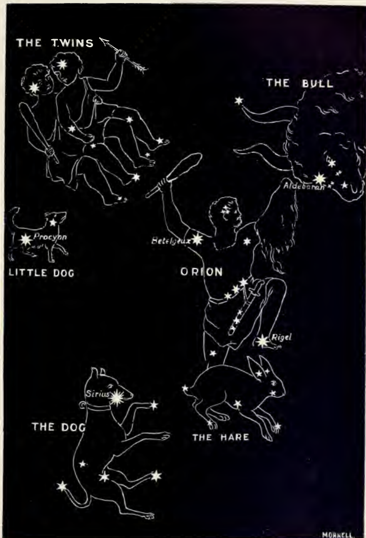
ORION AND HIS NEIGHBOURS.
