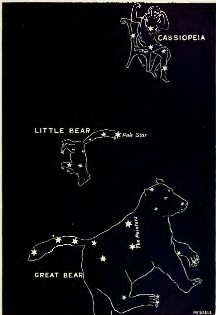
CONSTELLATIONS NEAR THE POLE STAR.
