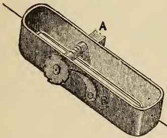
Fig. 96.—Tightener.
