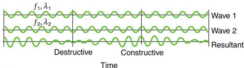
Figure 16.42 Beats are produced by the superposition of two waves of slightly different frequencies but identical amplitudes. The waves alternate in time between constructive interference and destructive interference, giving the resulting wave a time-varying amplitude.
