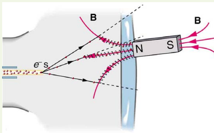
Figure 22.21 Side view showing what happens when a magnet comes in contact with a computer monitor or TV screen. Electrons moving toward the screen spiral about magnetic field lines, maintaining the component of their velocity parallel to the field lines. This distorts the image on the screen.
