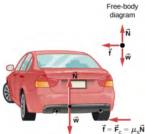
Figure 6.21 This car on level ground is moving away and turning to the left. The centripetal force causing the car to turn in a circular path is due to friction between the tires and the road. A minimum coefficient of friction is needed, or the car will move in a larger-radius curve and leave the roadway.
