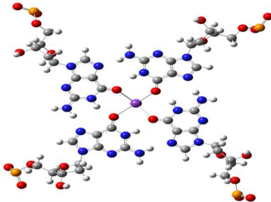
Figure 3 | Structure of a representative G-Quadruplex consisting of Hoogsteen base pairs between every neighboring Guanine residues (PDB: 1KF1)
