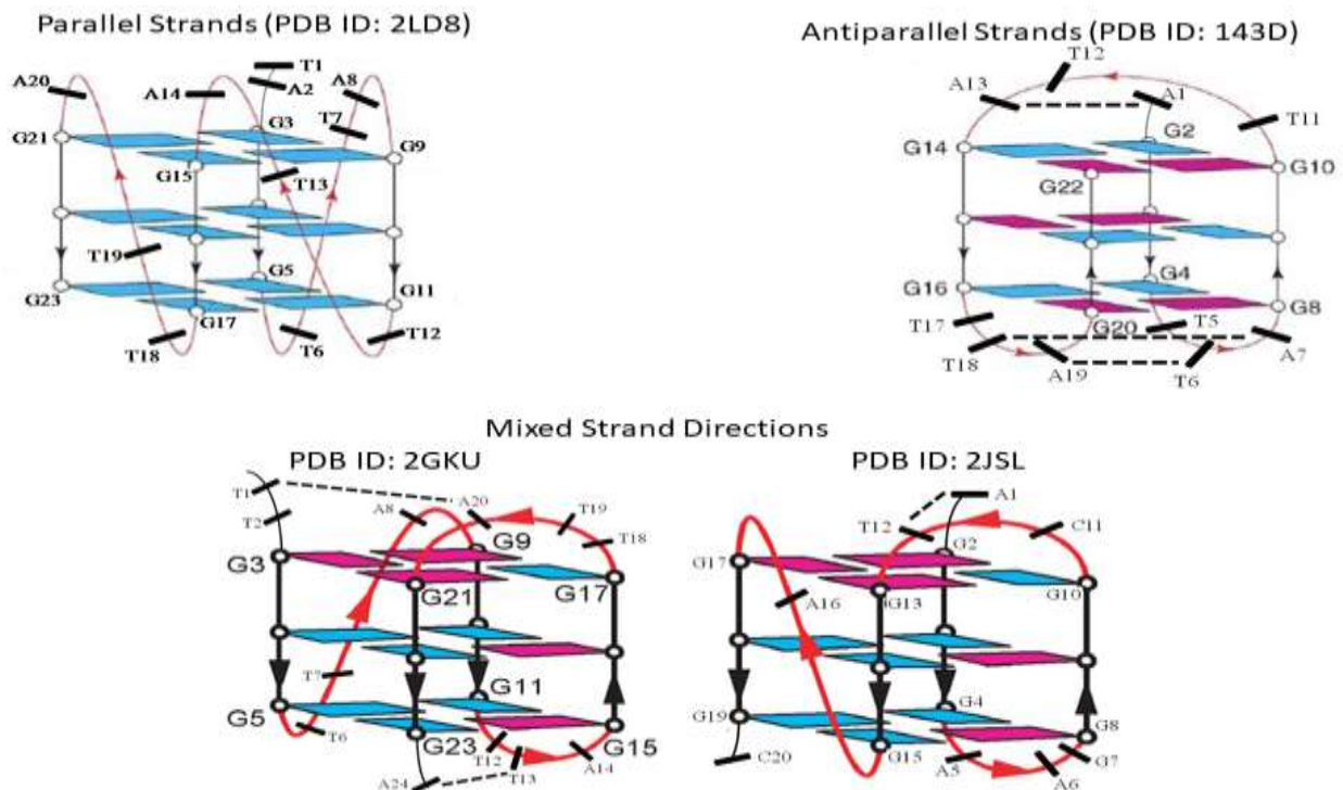
Figure 4 | Three G-quadruplexes stack to form four stranded telomere with different topologies for d(GGGATTGGGATTGGGATTGGG) sequence
