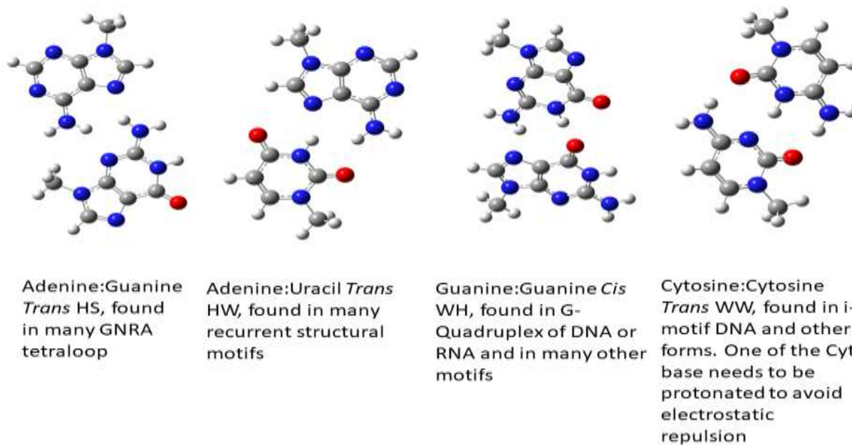
Figure 1 | Examples of few frequently observed non-canonical base pairs, (a) Adenine: Guanine trans Hoogsteen/Sugar-edge, (b) Adenine: Uracil trans Hoogsteen/Watson-Crick, (c) Guanine: Guanine cis Watson-Crick/Hoogsteen; (d) Protonated Cytosine (+): Cytosine trans Watson-Crick/Watson-Crick
