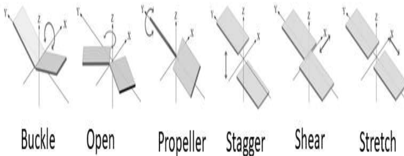
Figure 8 | IUPAC recommended Intra Base Pair parameters used to describe geometry of Watson-Crick or Non-Canonical base pair
