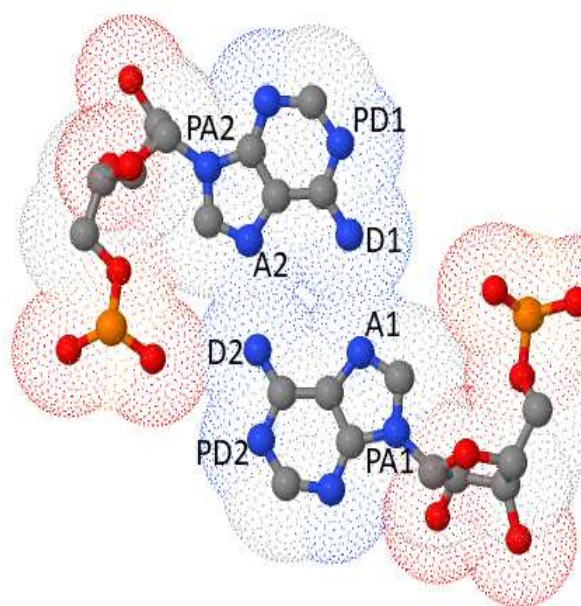
Figure 7 | Descriptions of the hydrogen bonding atoms, along with their precursors, for a typical non-canonical base pair (as used by BPFIND)
