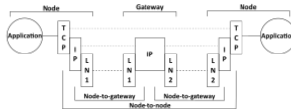
Figure 5: ARPANET model for a transmission path between two hosts and a gateway.
