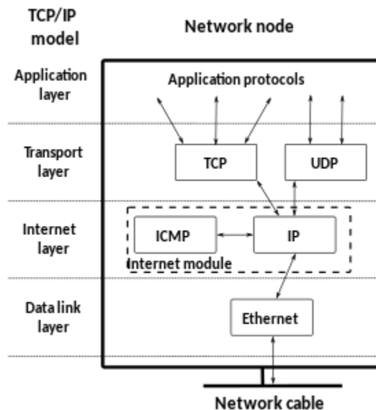
Figure 4: Basic TCP/IP network node.
