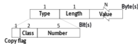
Figure 8: IPv4 option general structure
