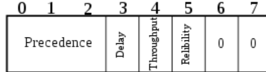
Figure 9: The structure of the ToS field in the IPv4 header according to RFC 791
