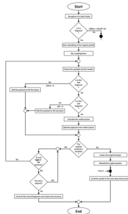
Figure 21: IPv4 Reassembly algorithm as specified in RFC 791.
