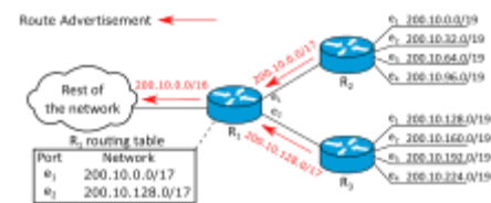
Figure 26: An example of route aggregation as a part of CIDR.
