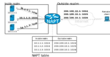
Figure 29: PNAT in a SOHO
