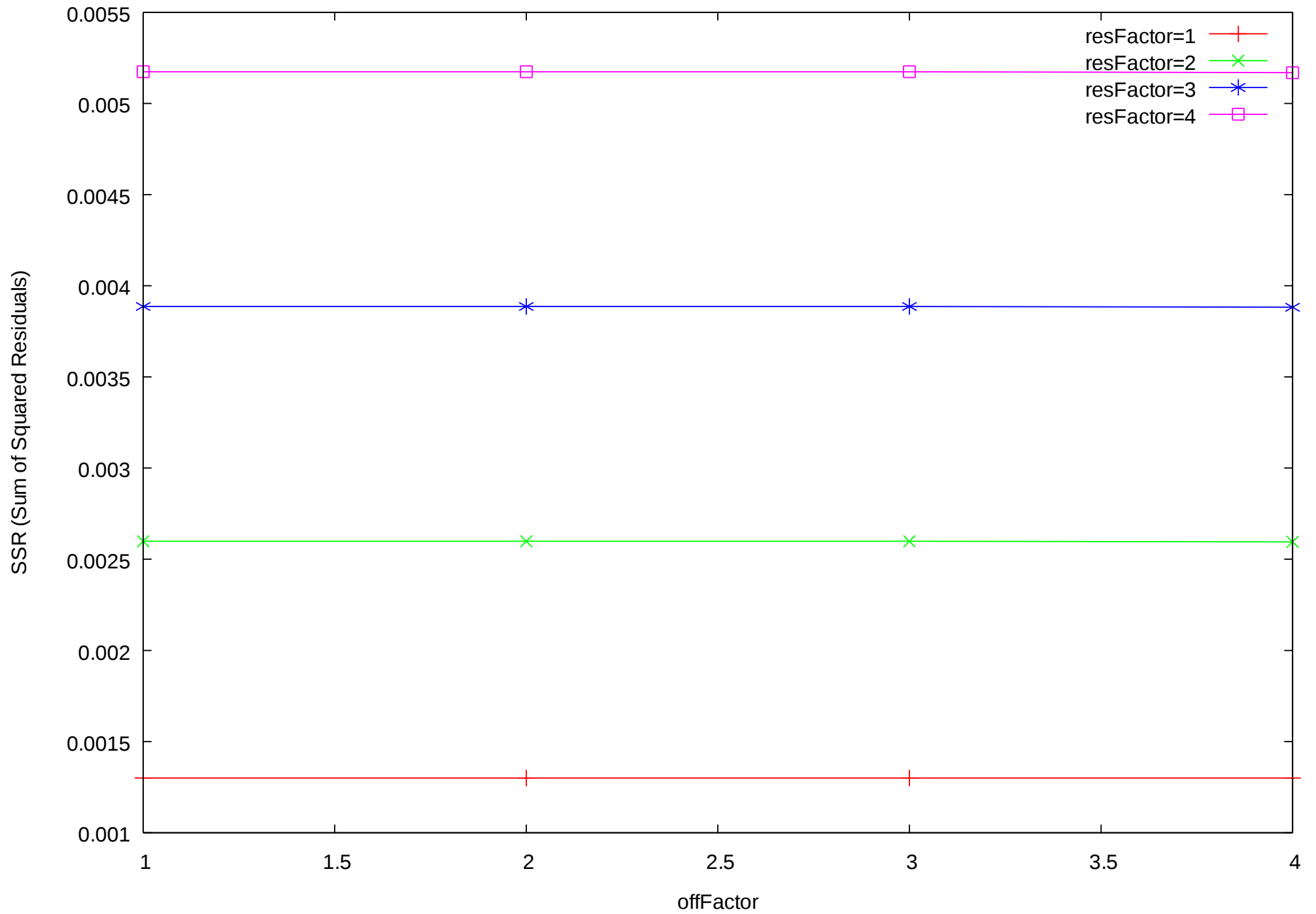
offFactor-SSR Plot (Leaf)
