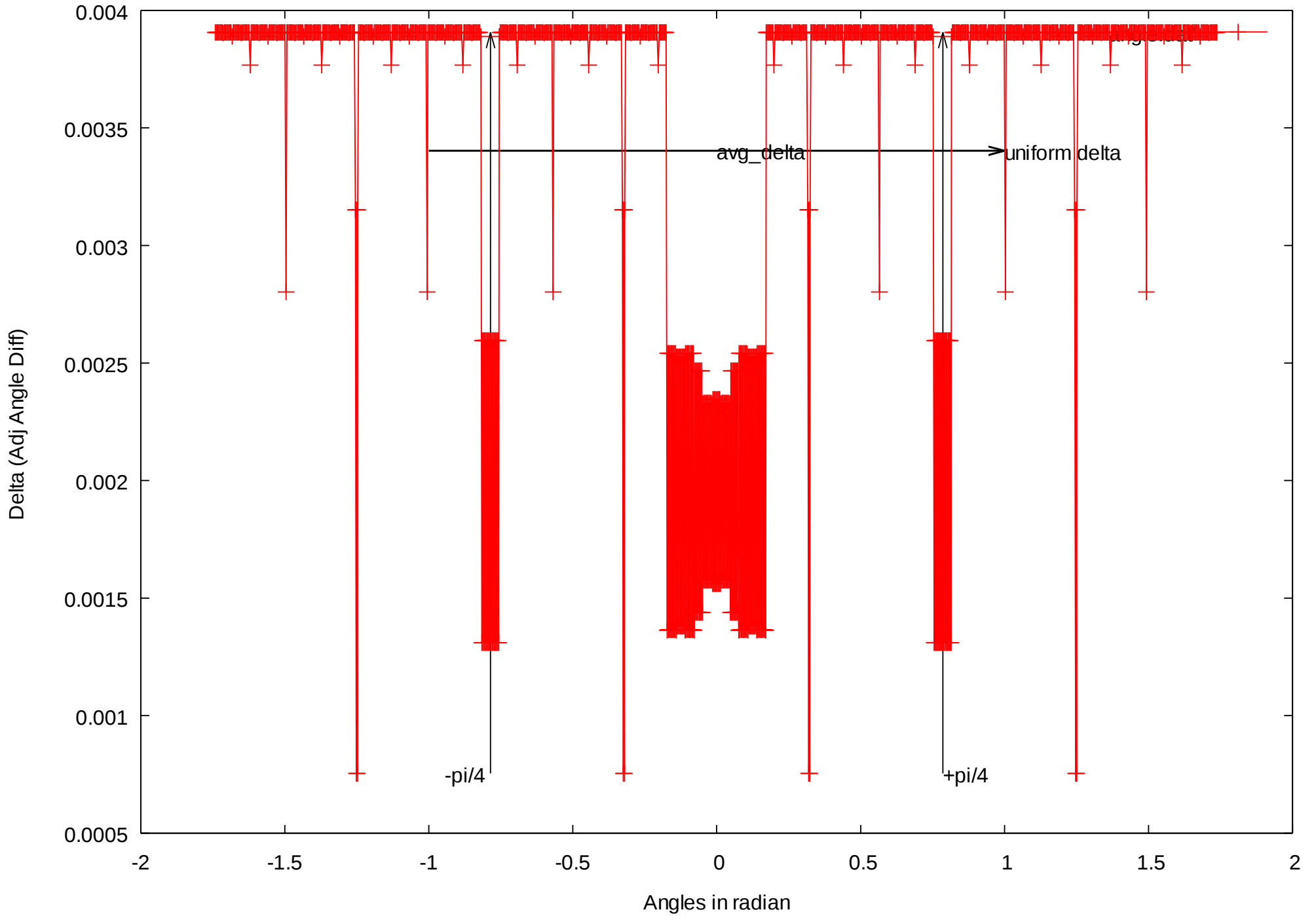
Angle-Delta Plot of Leaf Angles
