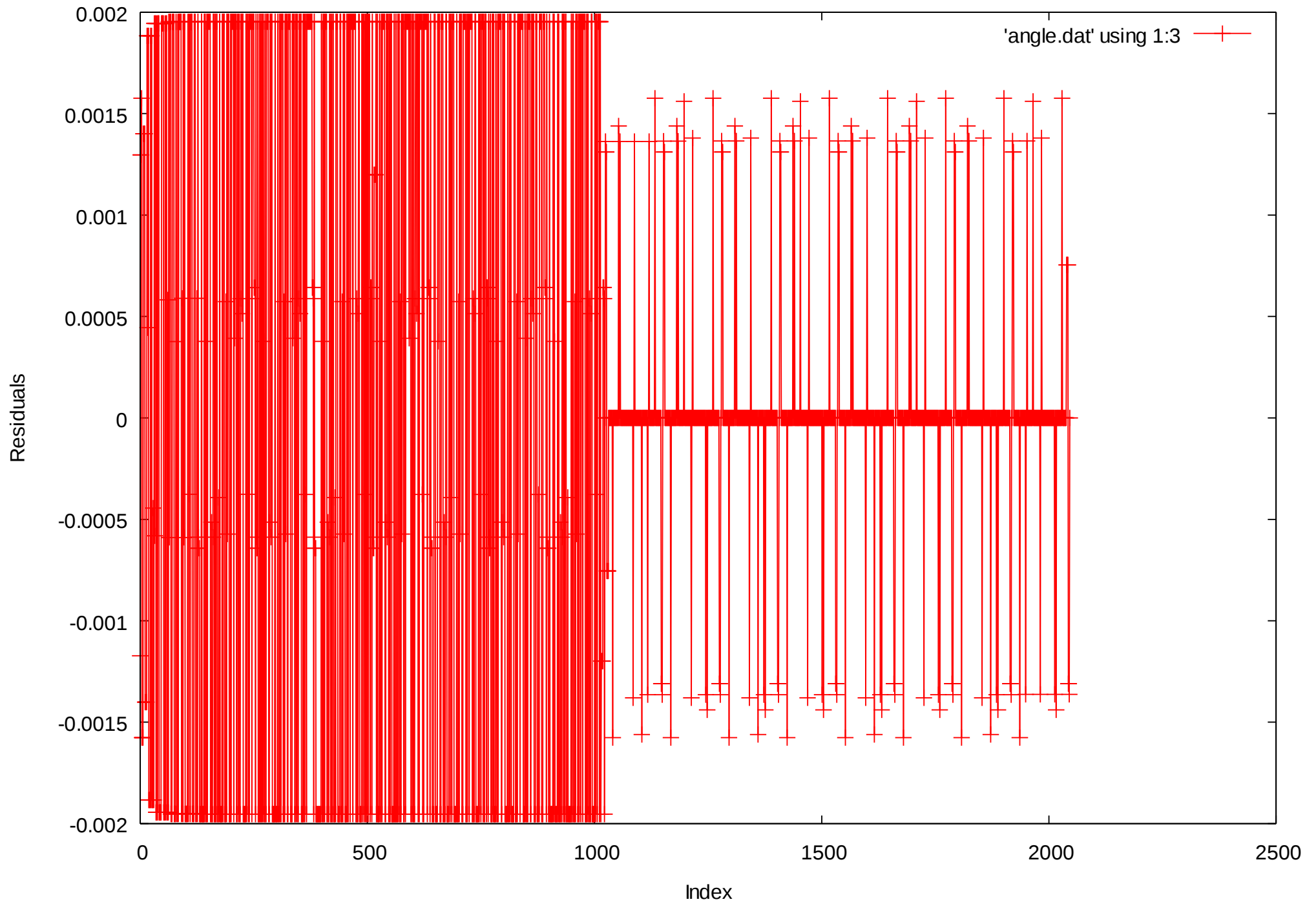
Index-Residual Plot (All)
