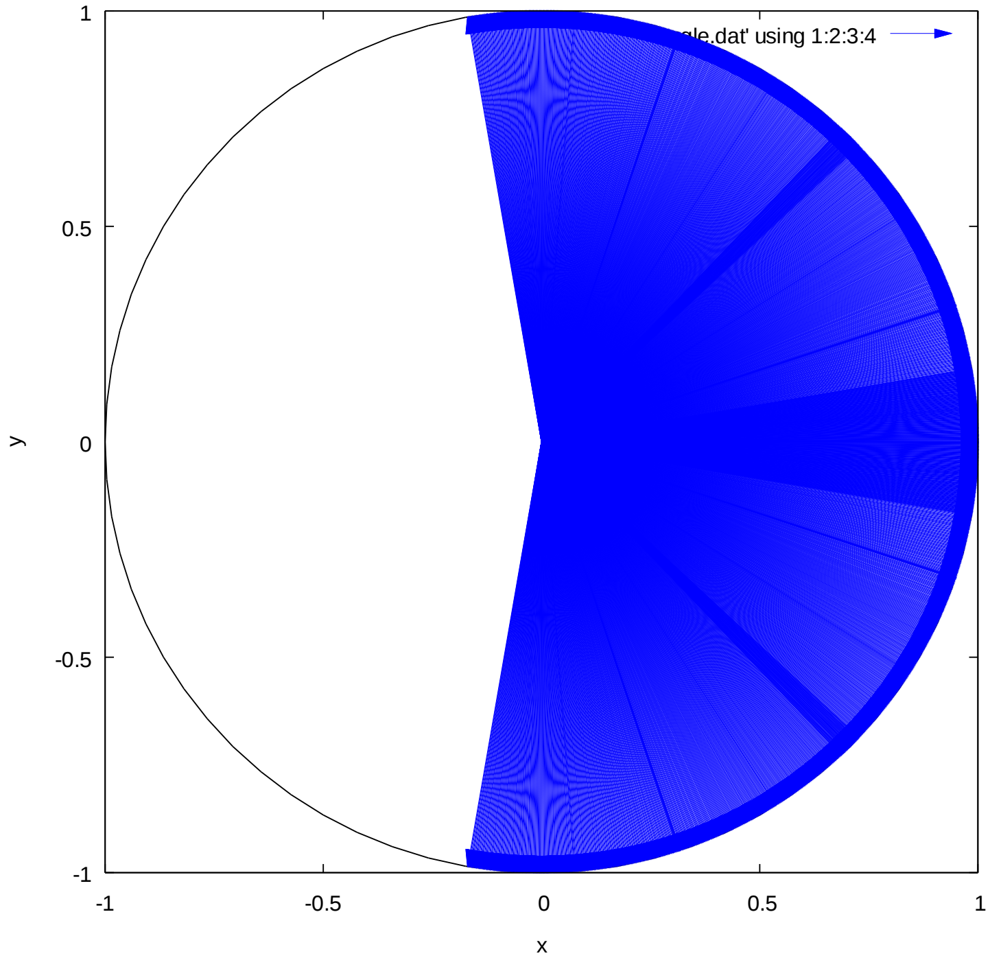
All Angles on a unit circle
