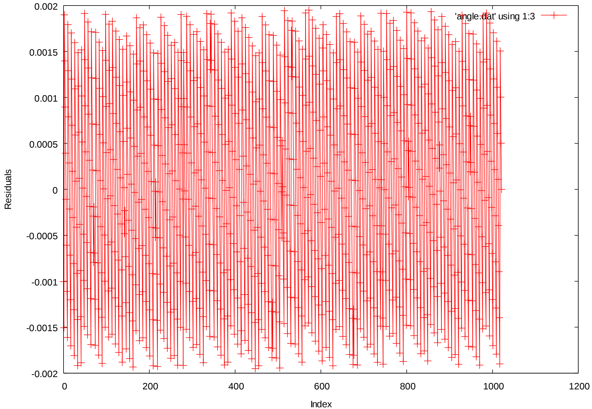
Index-Residual Plot (uScale-Leaf)
