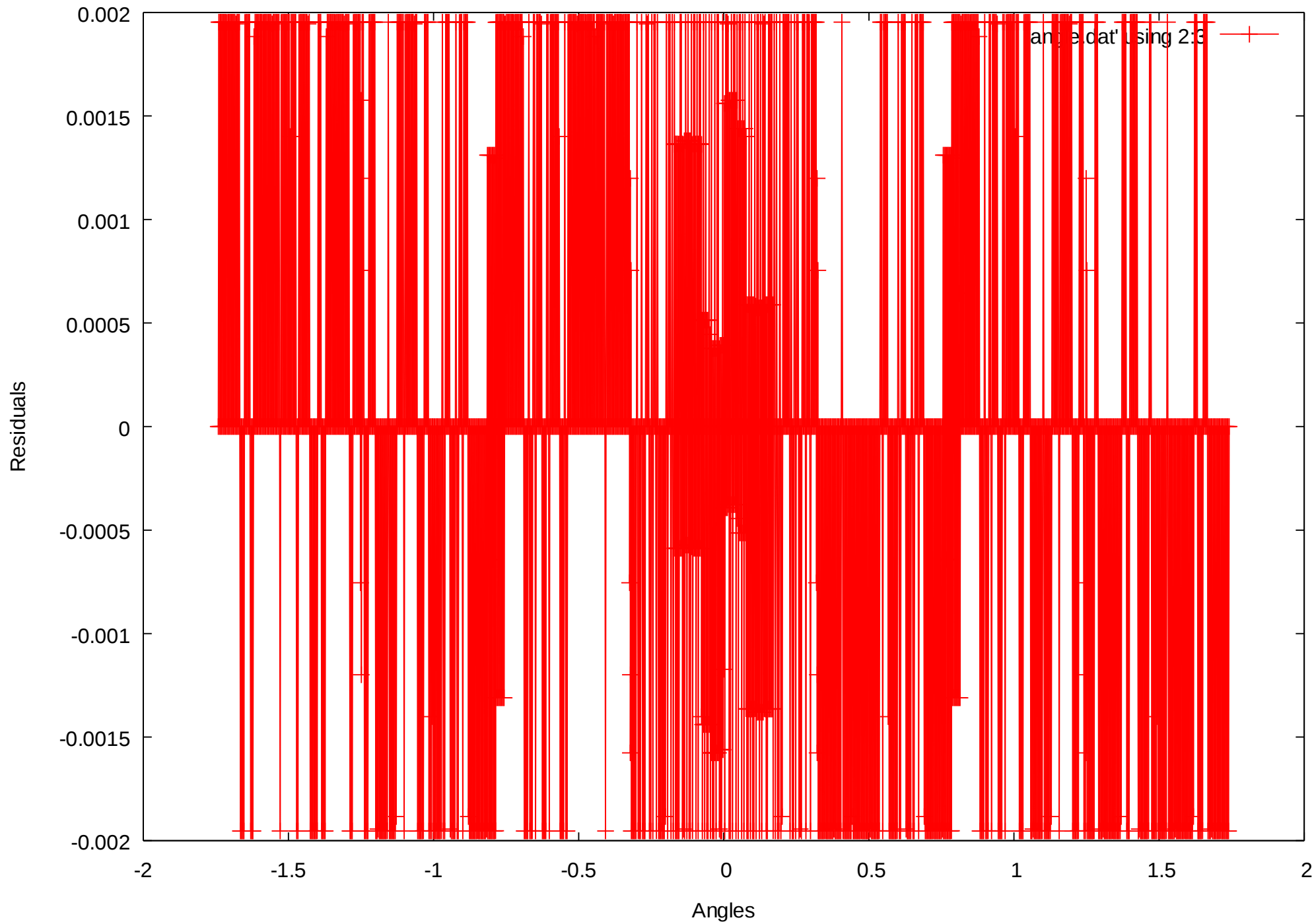
Angle-Residual Plot of (All)
