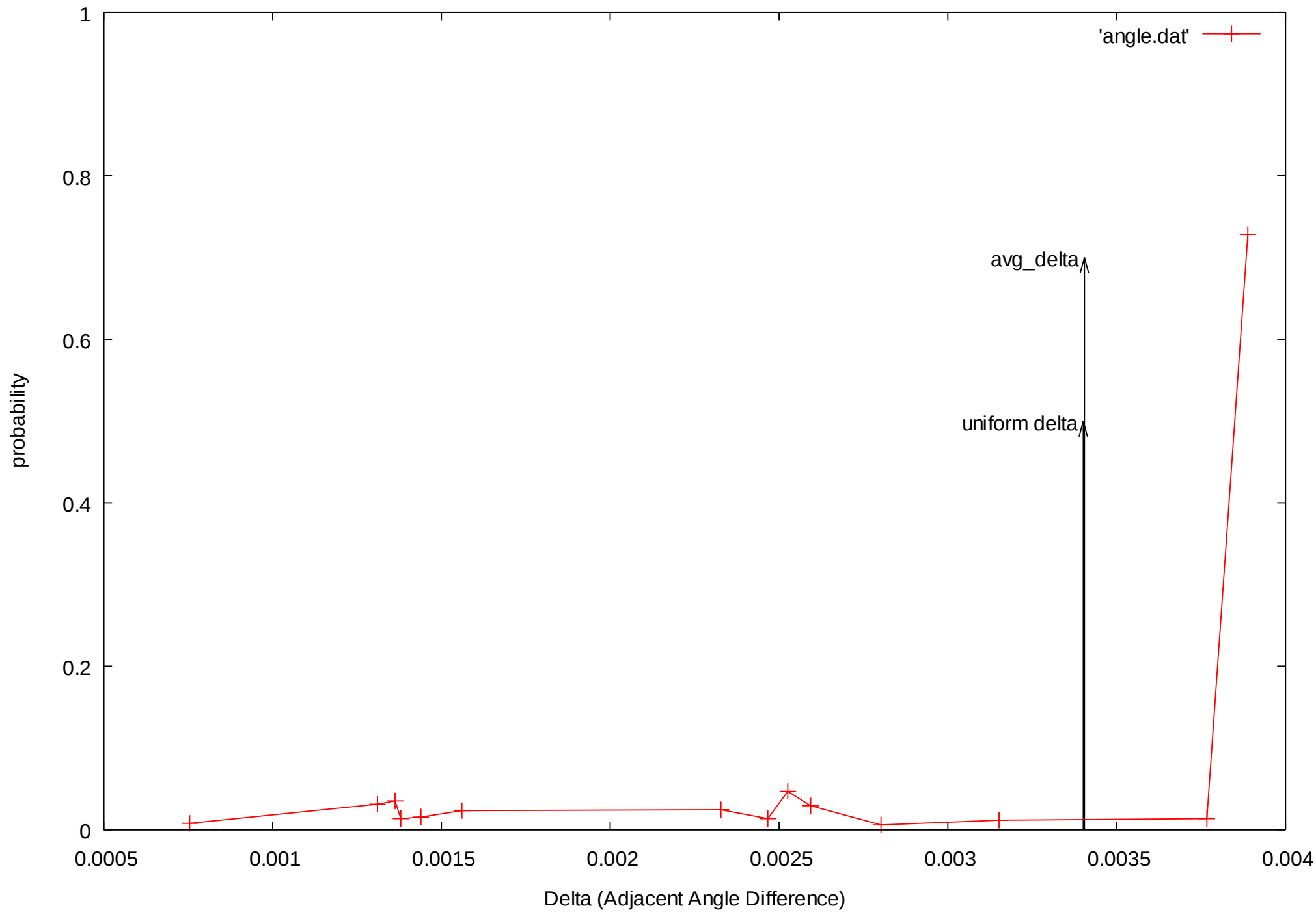
Delta Distribution of Leaf Angles
