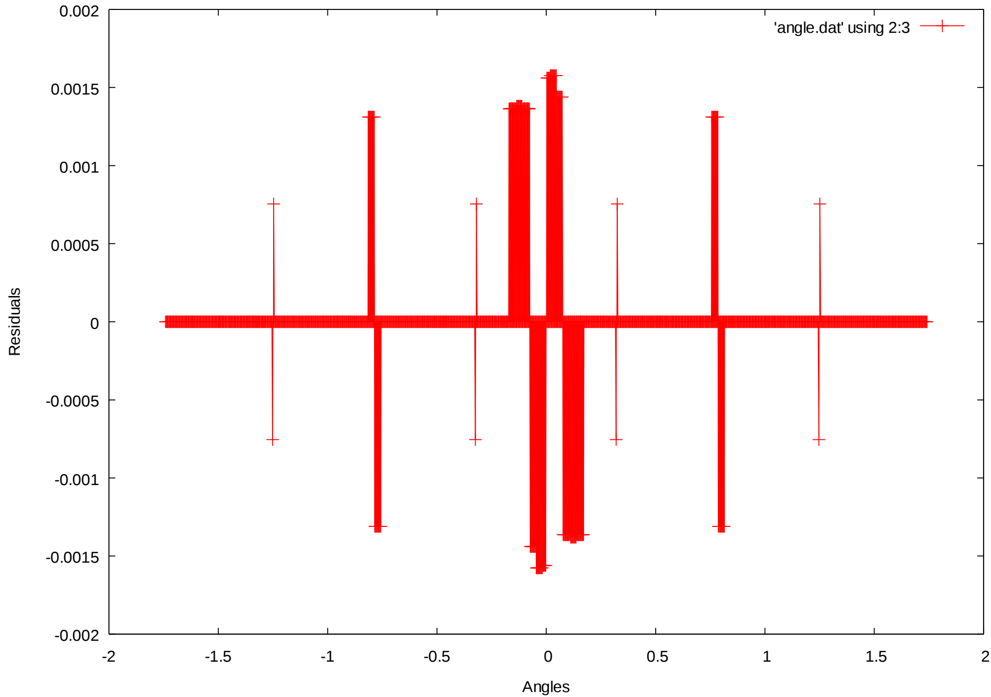
Angle-Residual Plot (Leaf)
