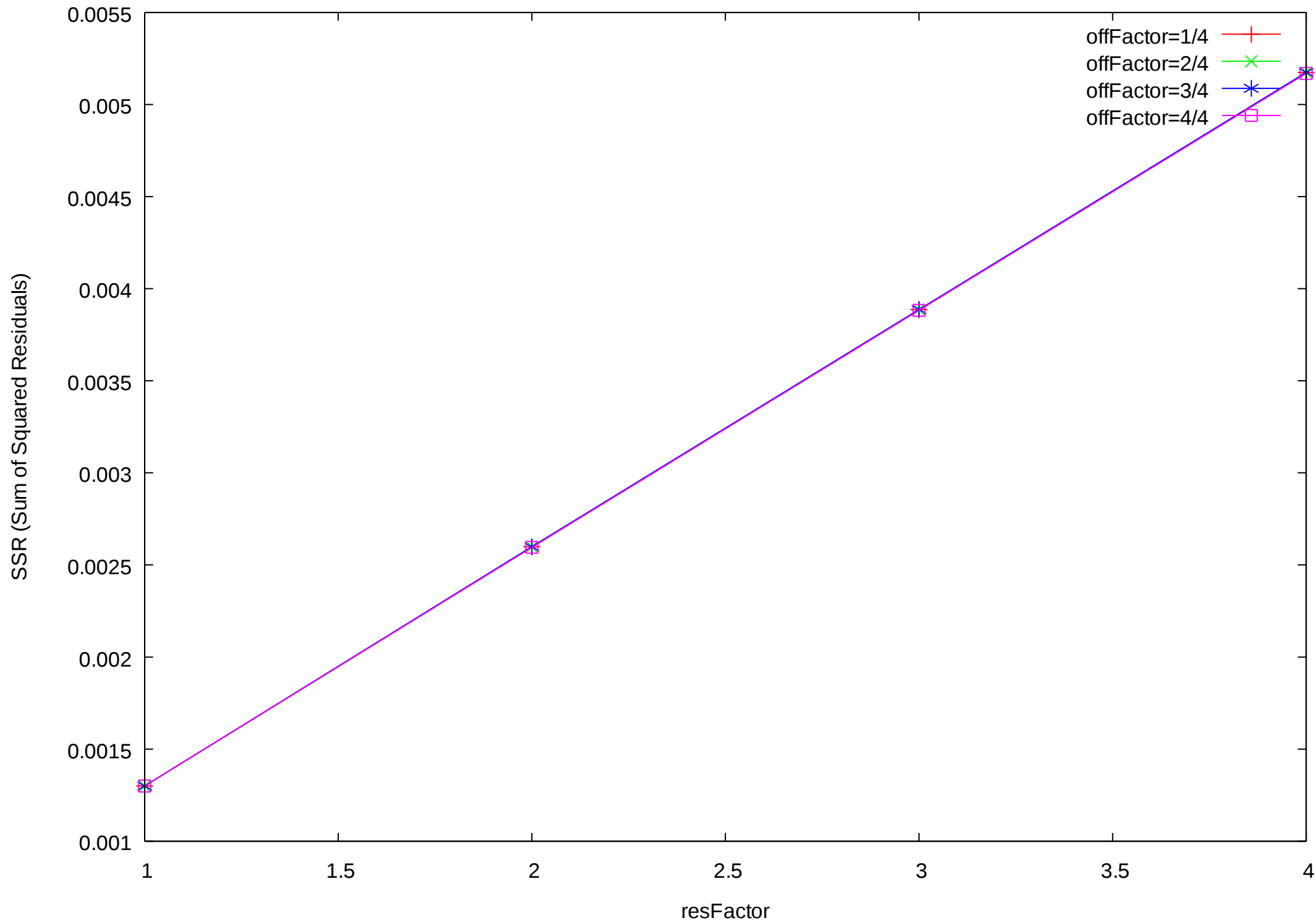
resFactor-SSR Plot (Leaf)
