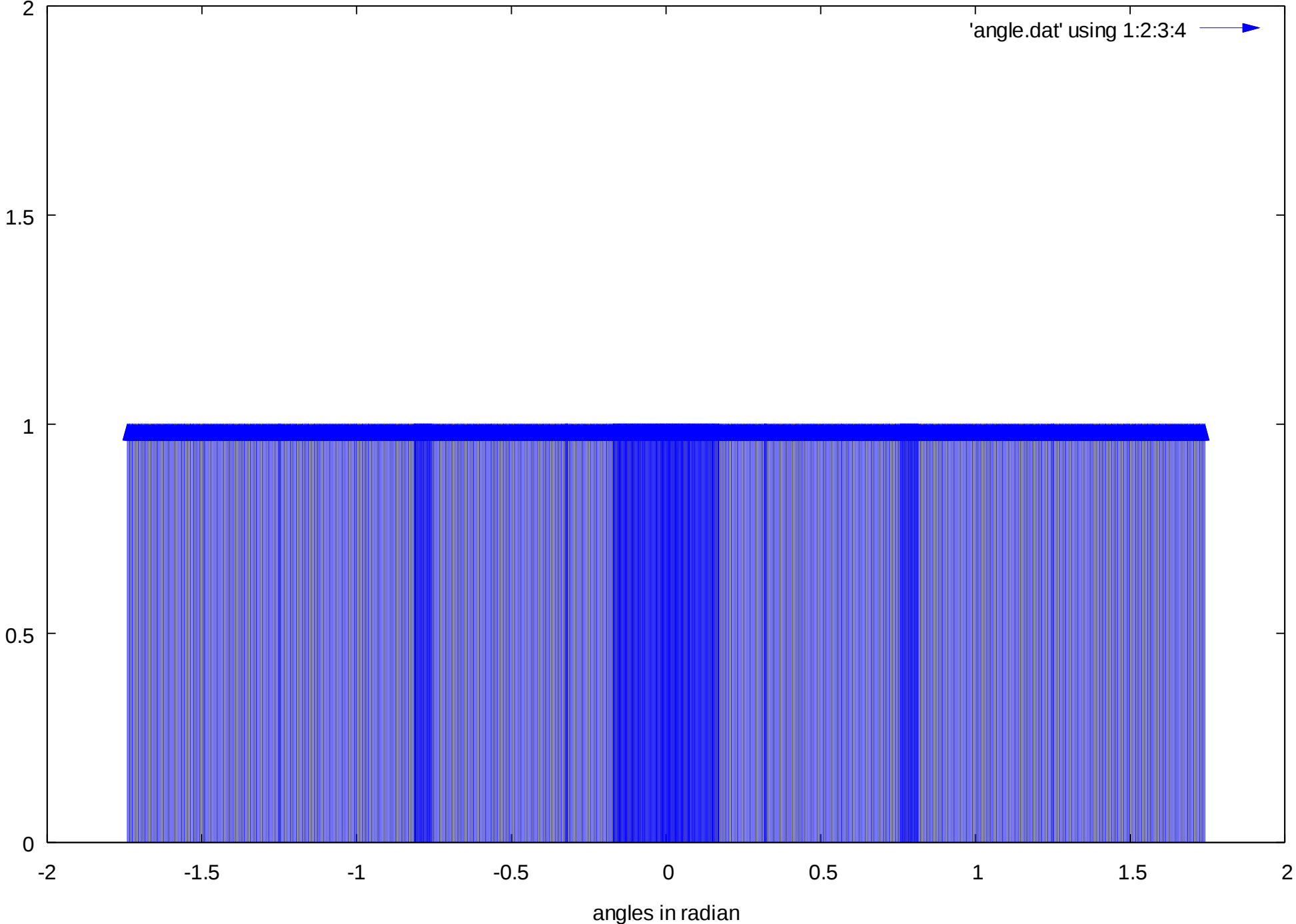
Leaf Angles on a linear scale
