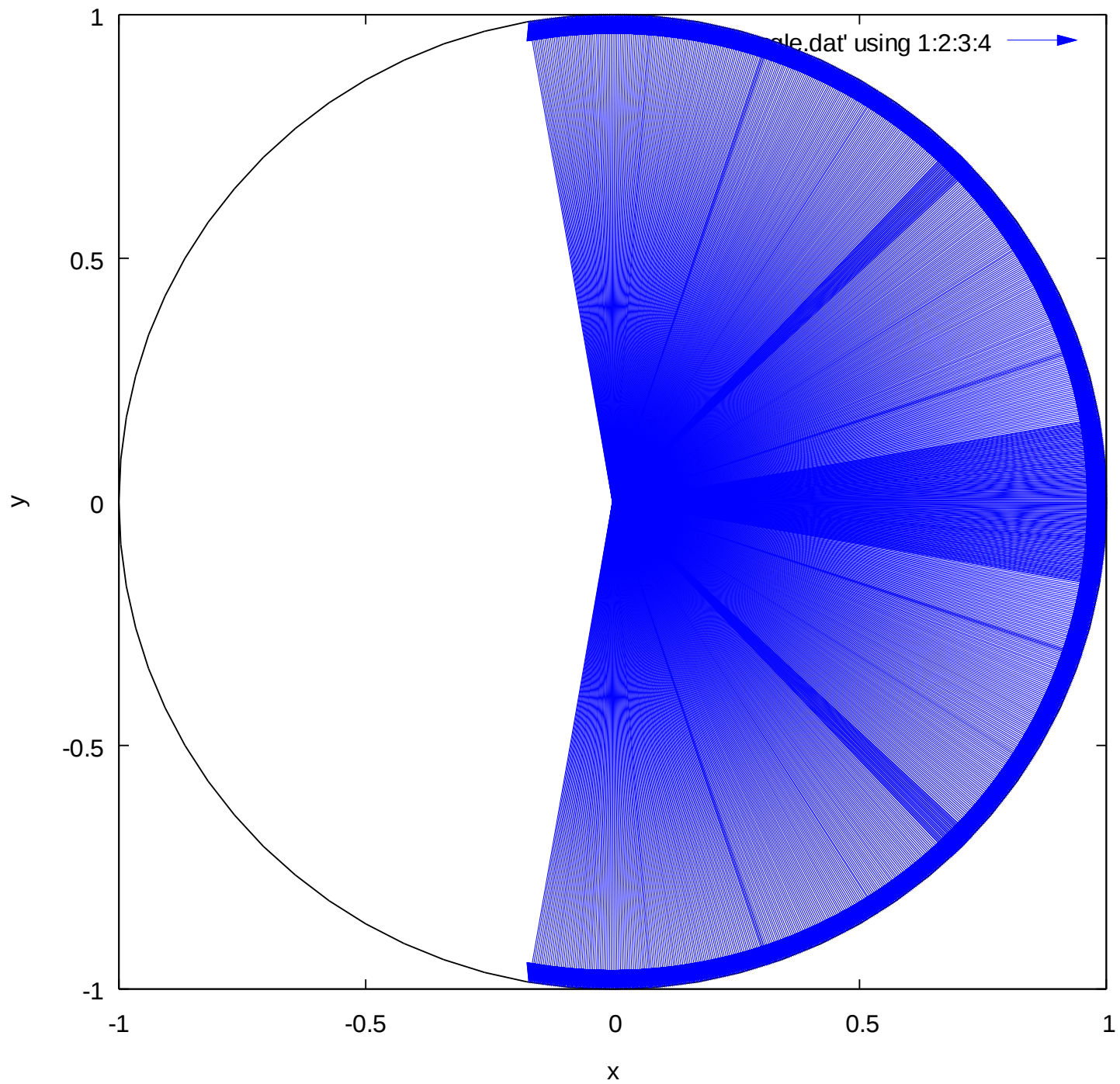
Leaf Angles on a unit circle
