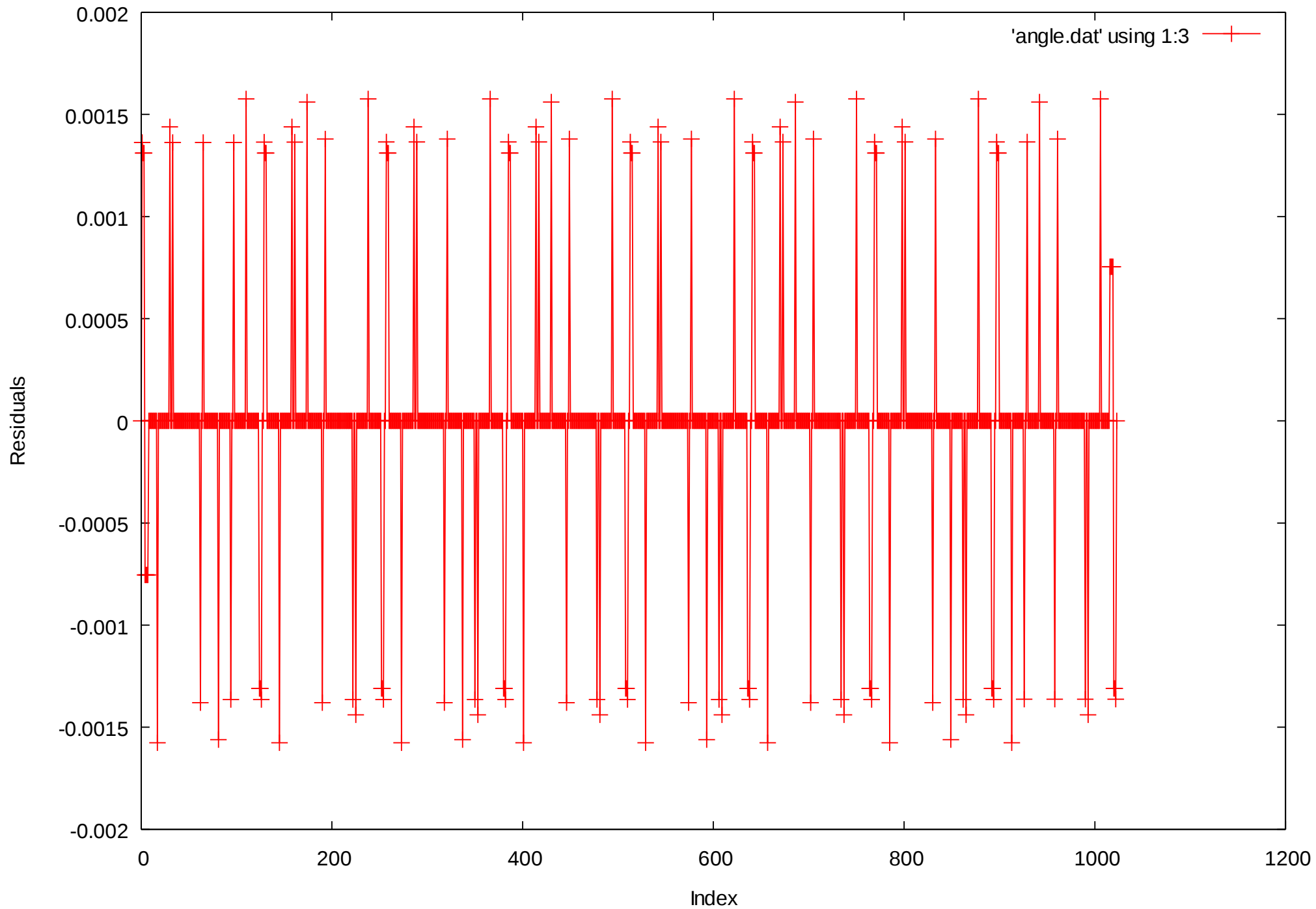
Index-Residual Plot (Leaf)
