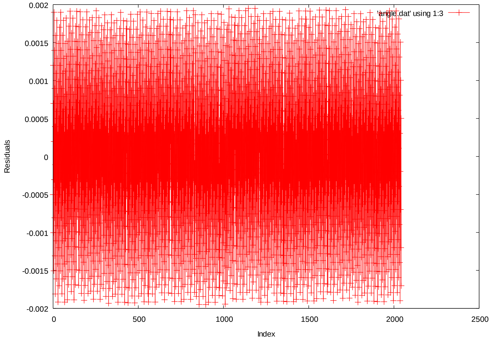
Index-Residual Plot (uScale-All)
