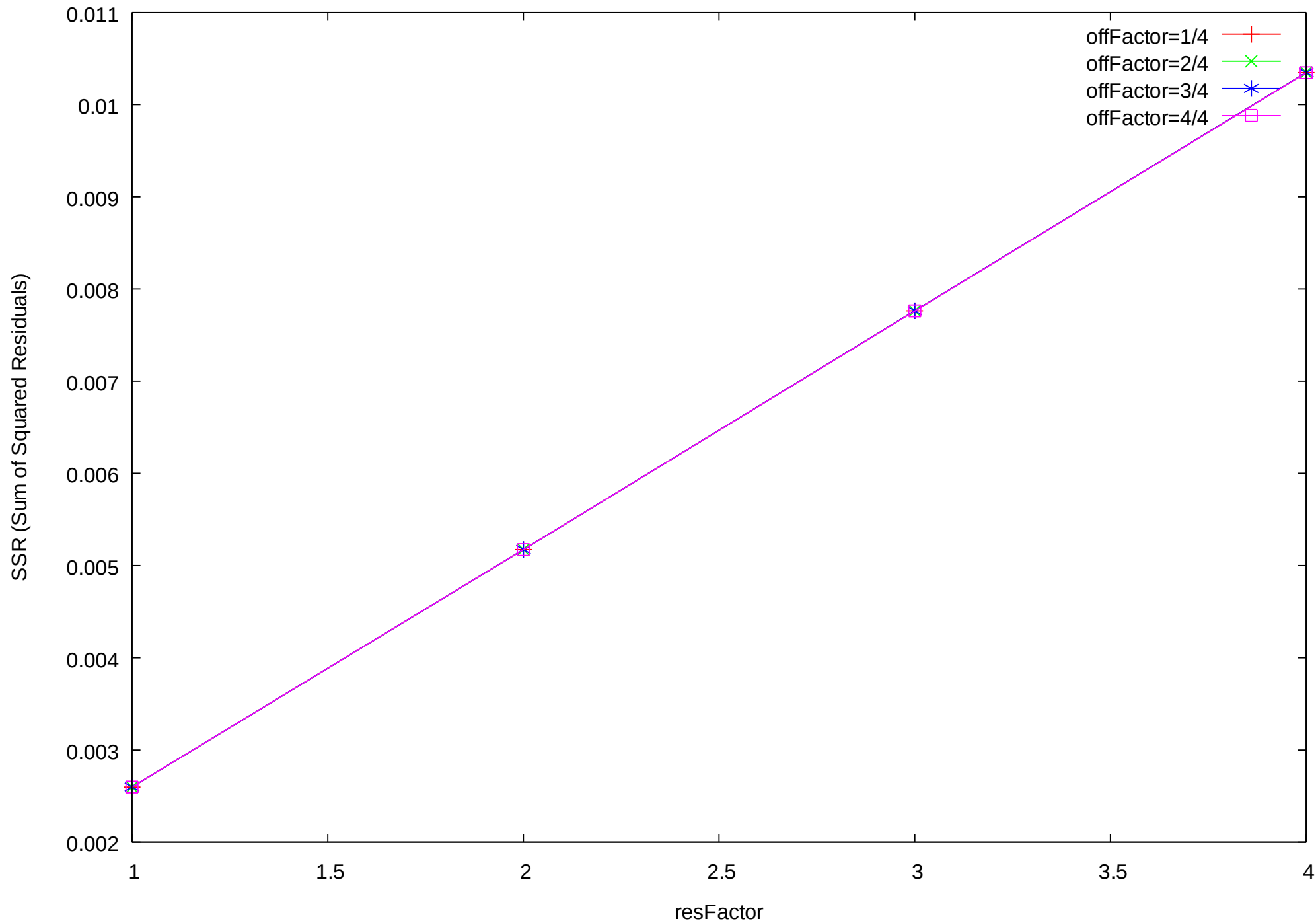
resFactor-SSR Plot (All)
