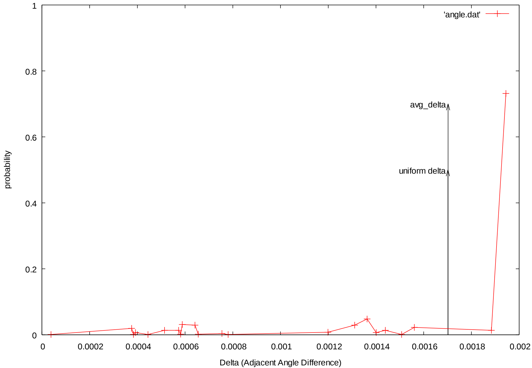
Delta Distribution of All Angles
