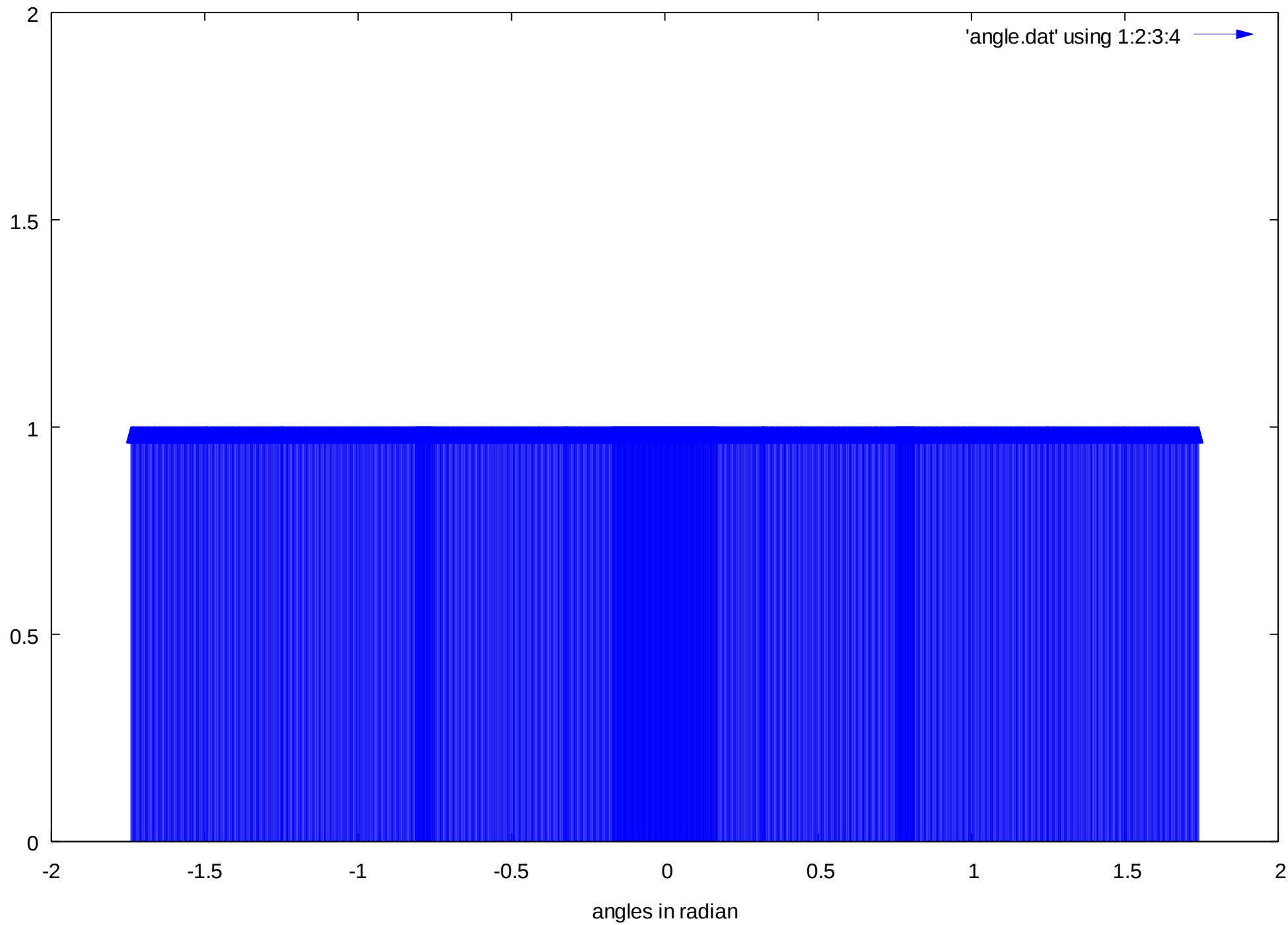
All Angles on a linear scale
