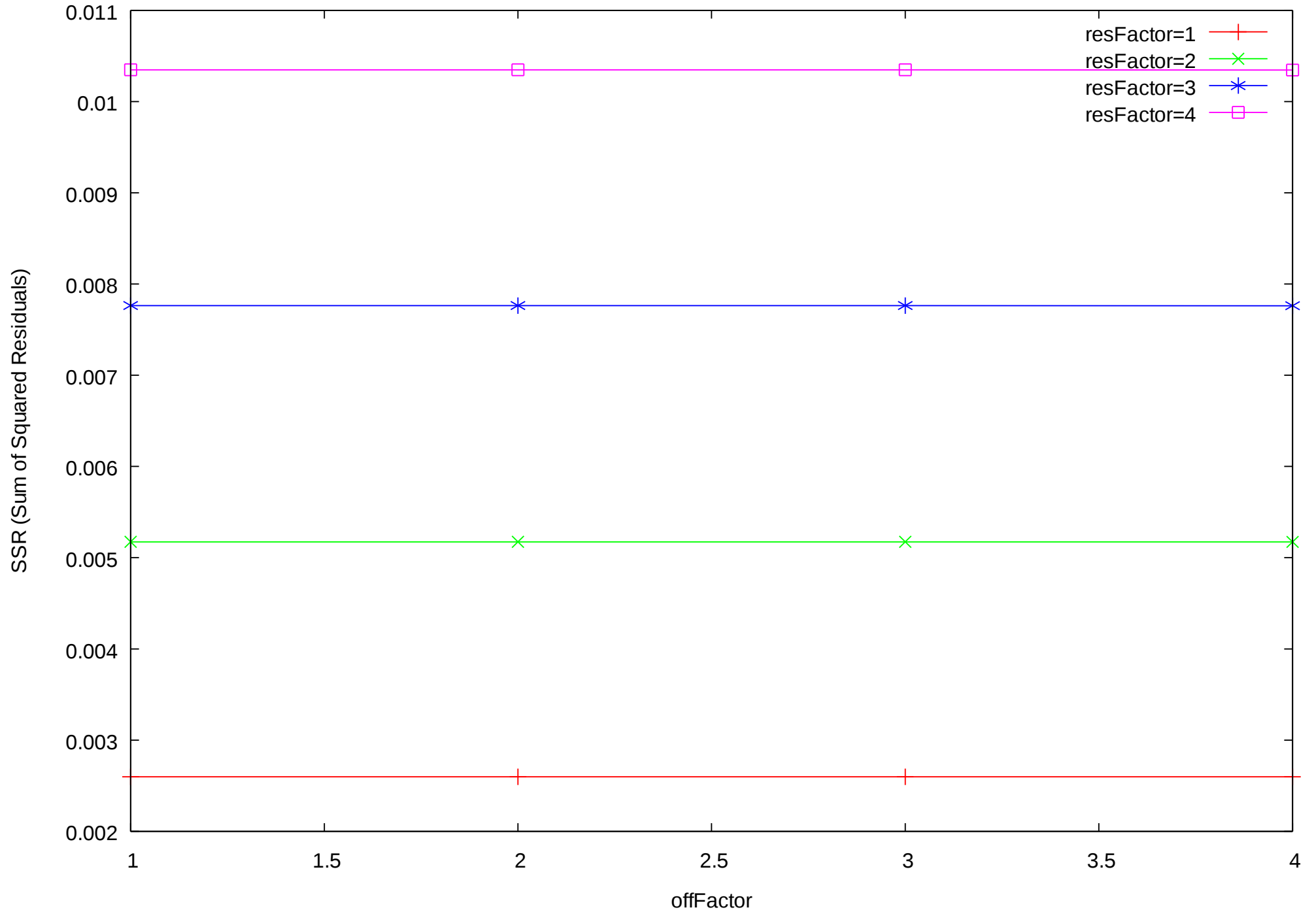
offFactor-SSR Plot (All)
